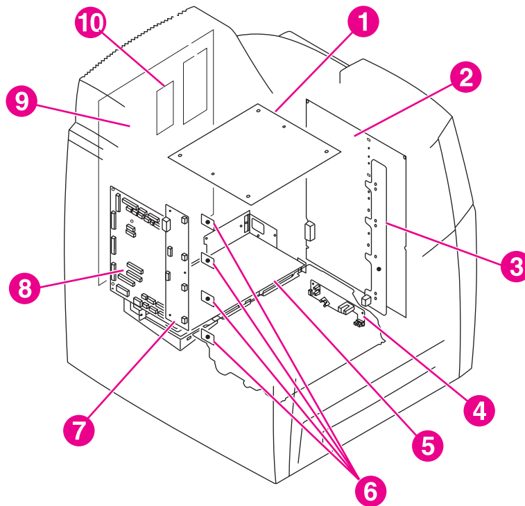
Figure 7-43 PCA locations
