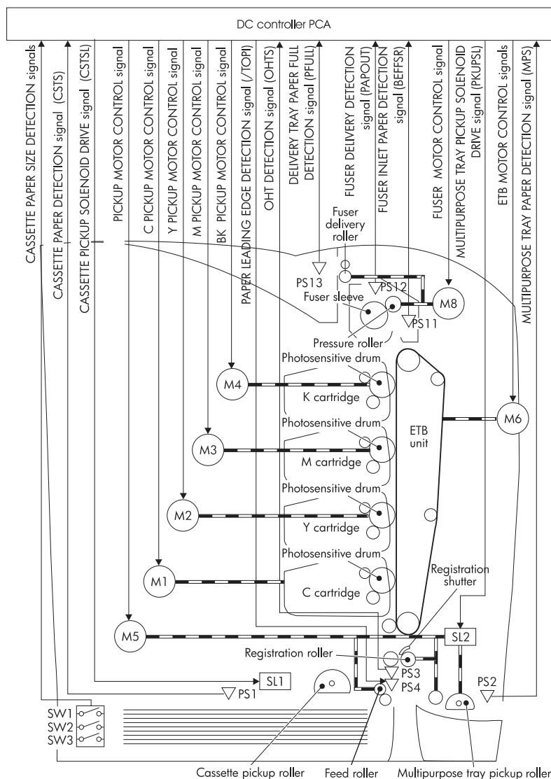
Figure 5-33 Pickup/feed system
