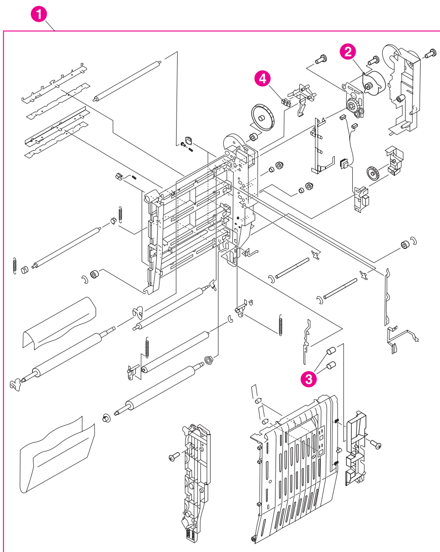
Figure 8-15 ETB assembly
