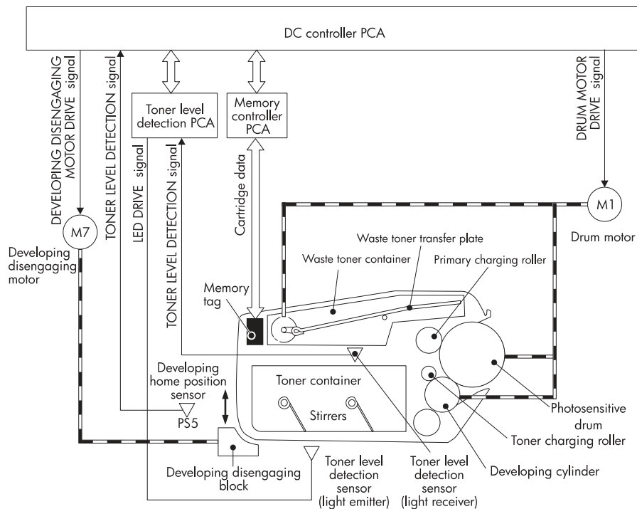
Figure 5-15 Print cartridge
