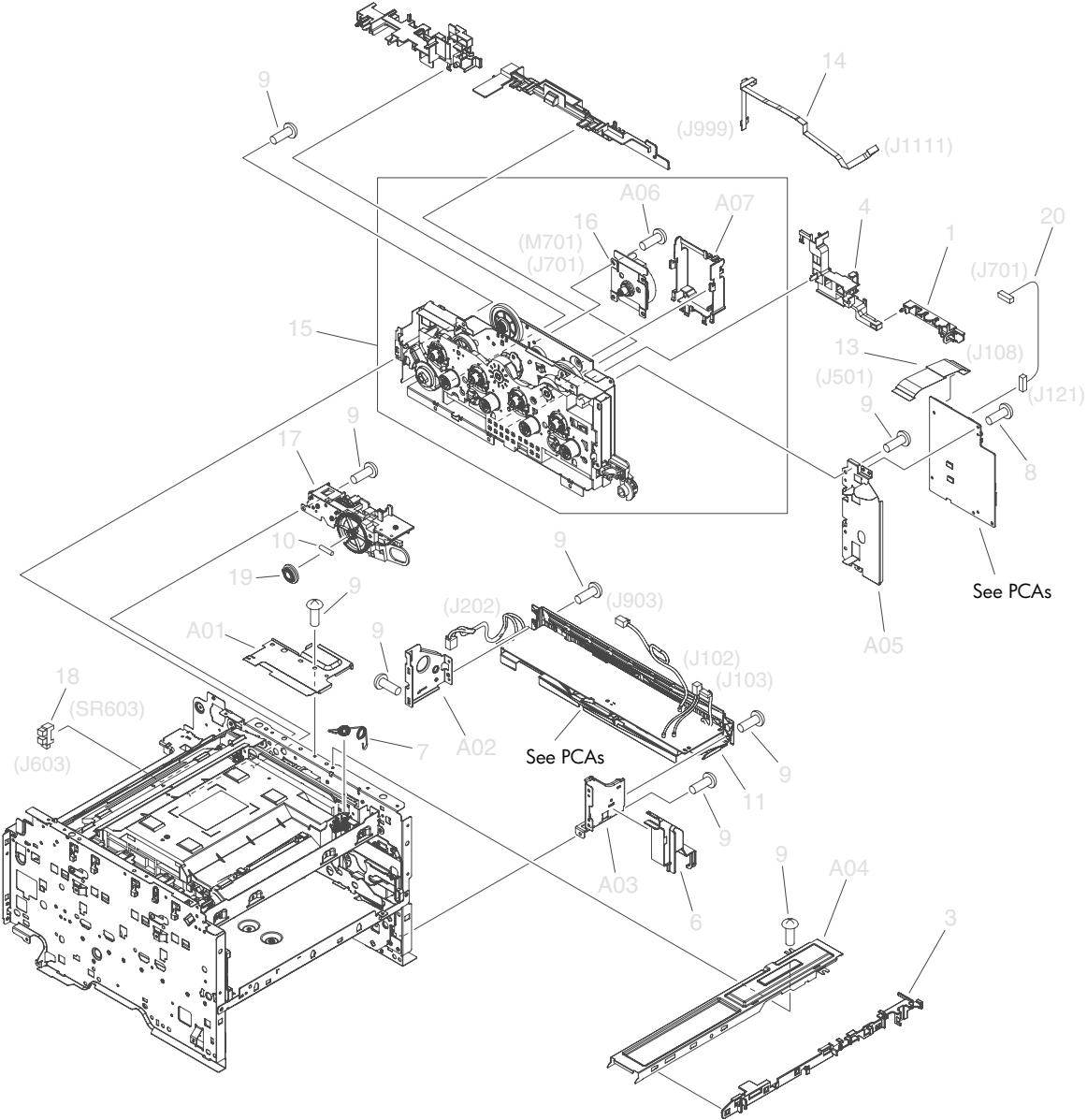
Figure 8-4 Internal components (2 of 4)
