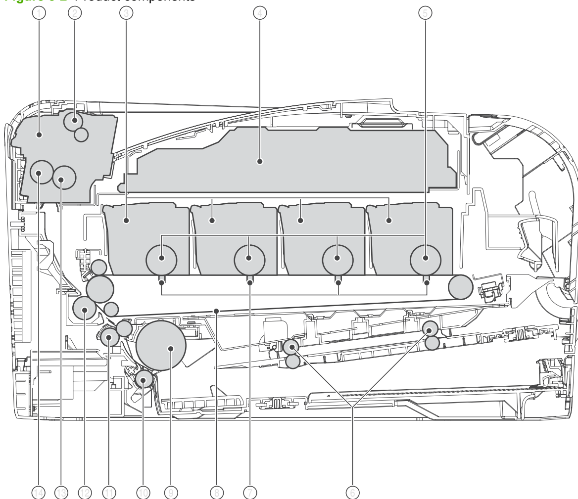
Figure 5-2 Product components
