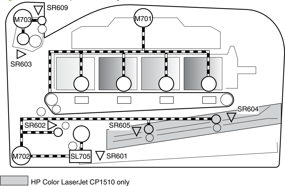
Figure 5-19 Pickup-and-feed system
