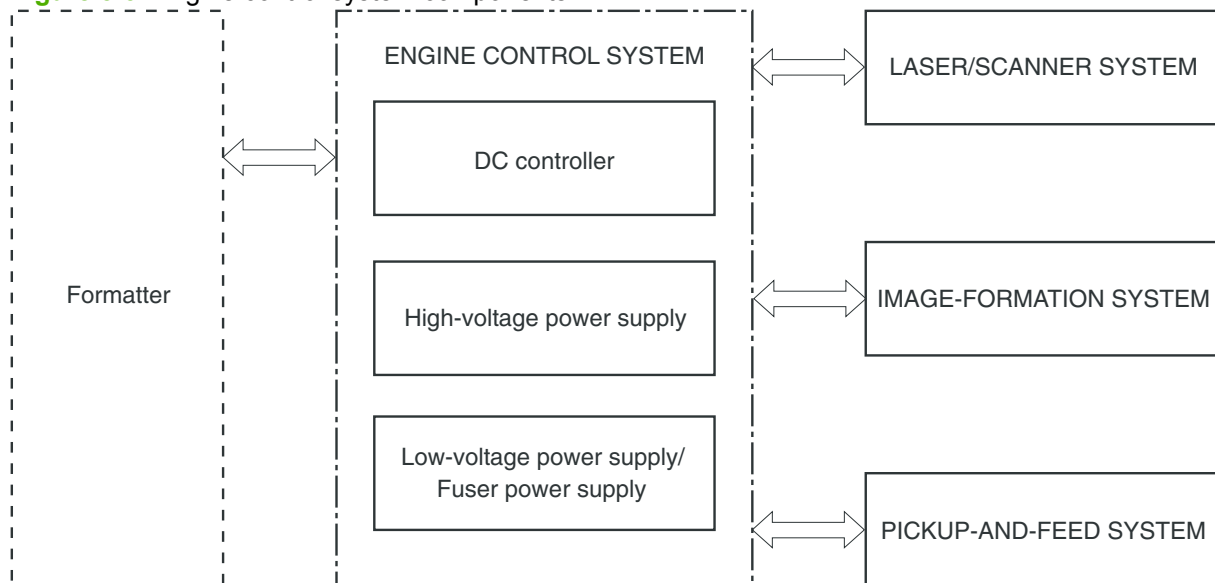
Figure 5-3 Engine control system components
