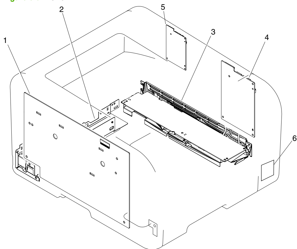
Figure 8-9 PCAs
