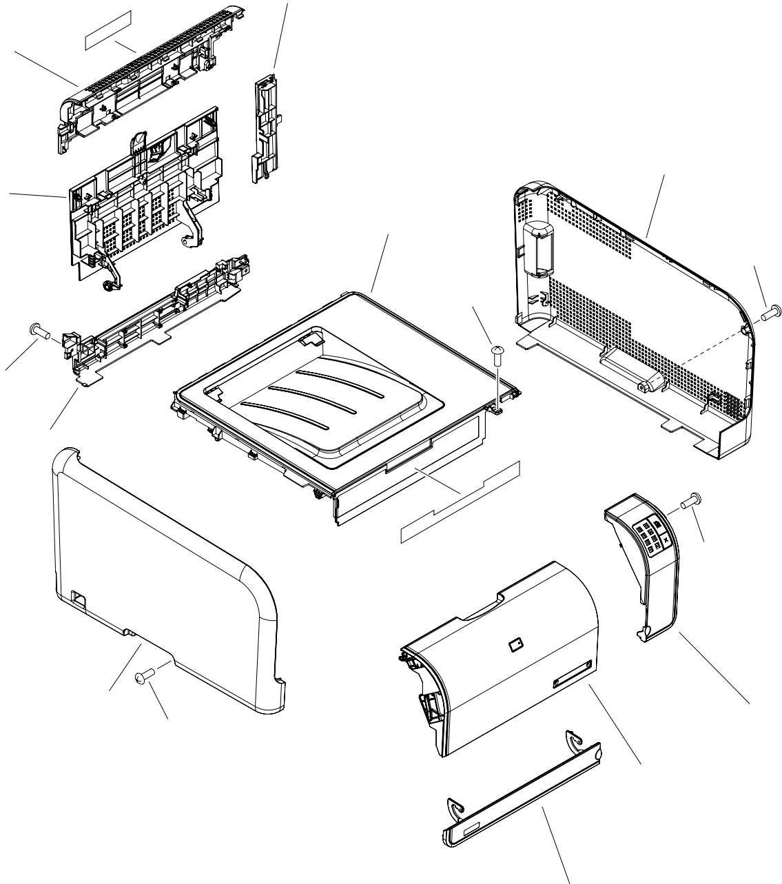
Figure 8-1 Covers, panels, and doors (HP Color LaserJet CP1210 Series Printer)
