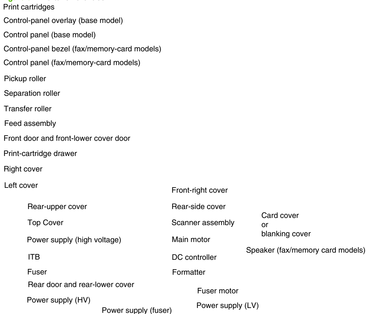
Figure 6-2 Parts-removal tree
