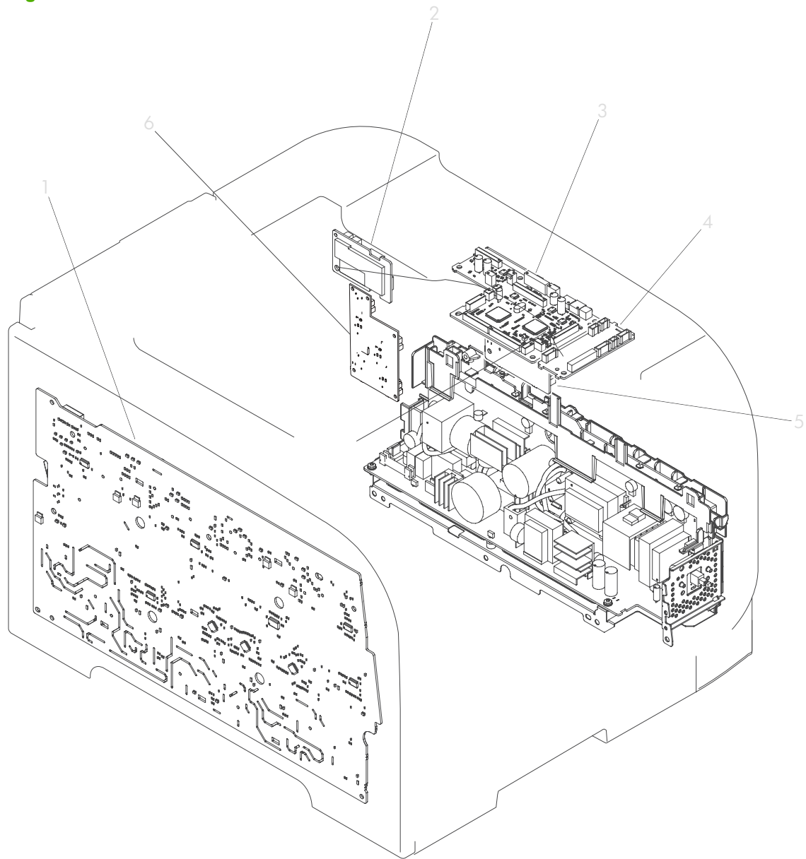
Figure 8-11 PCAs
