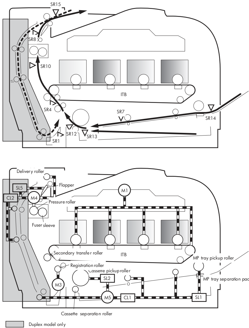
Figure 5-19 Pickup-and-feed system
