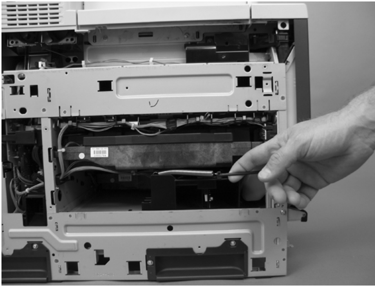
Figure 2-102 Remove the cartridge fan and environmental sensor (2 of 7)
