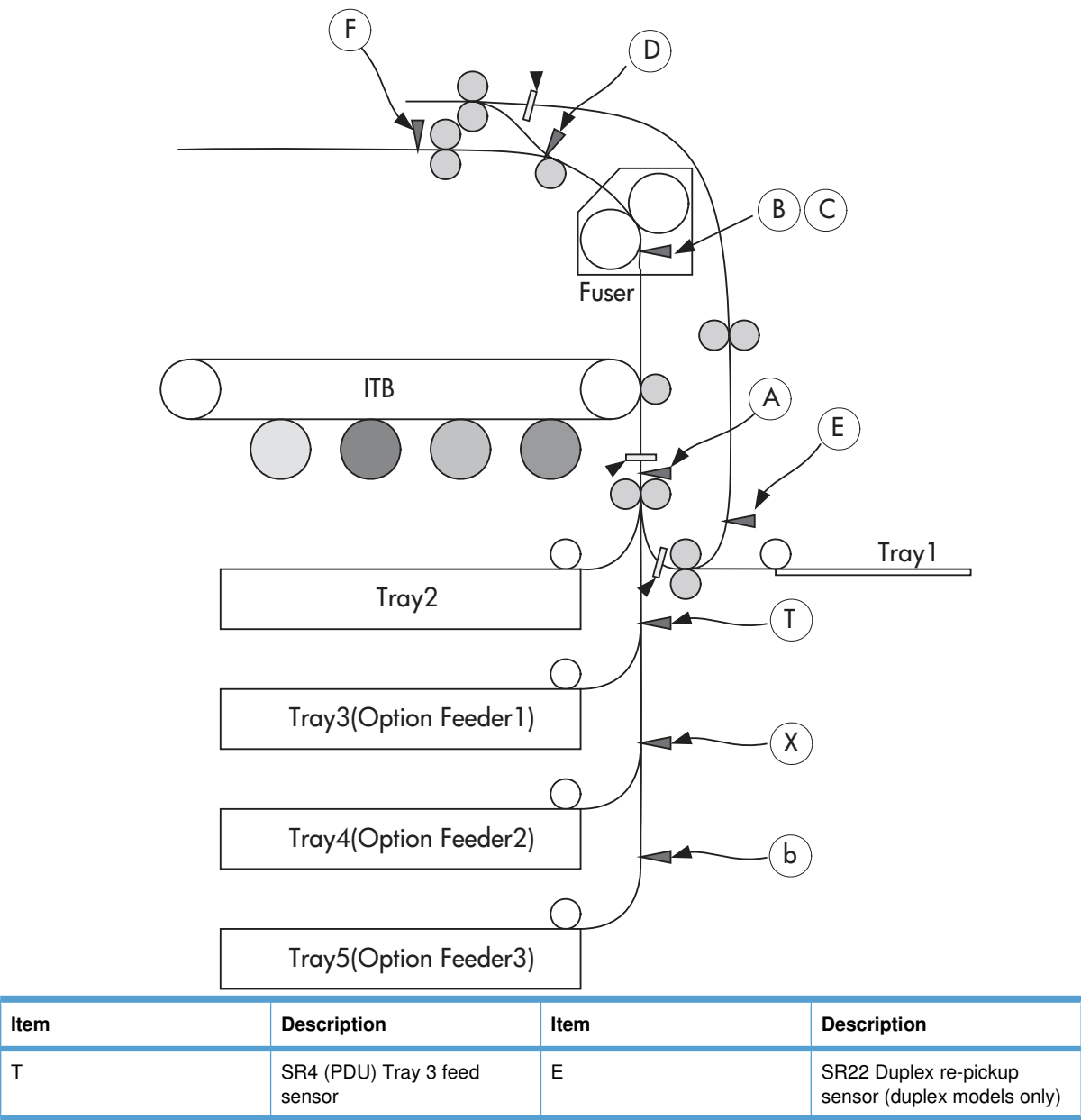
Figure 3-57 Common causes of jams (by area)
