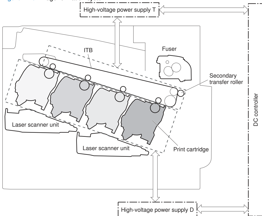
Figure 1-10 Image-formation system
