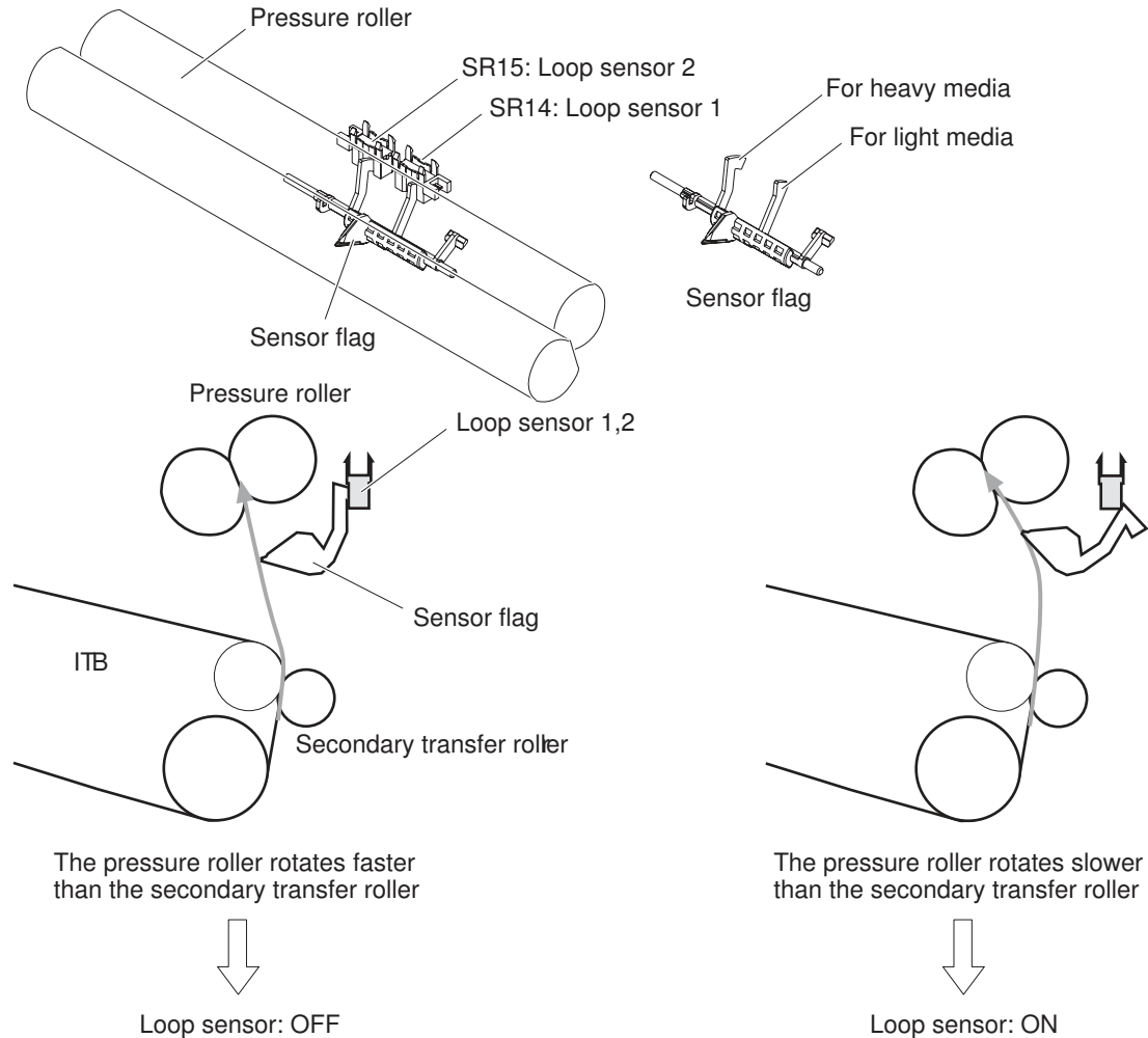
Figure 1-41 Loop-control mechanism
