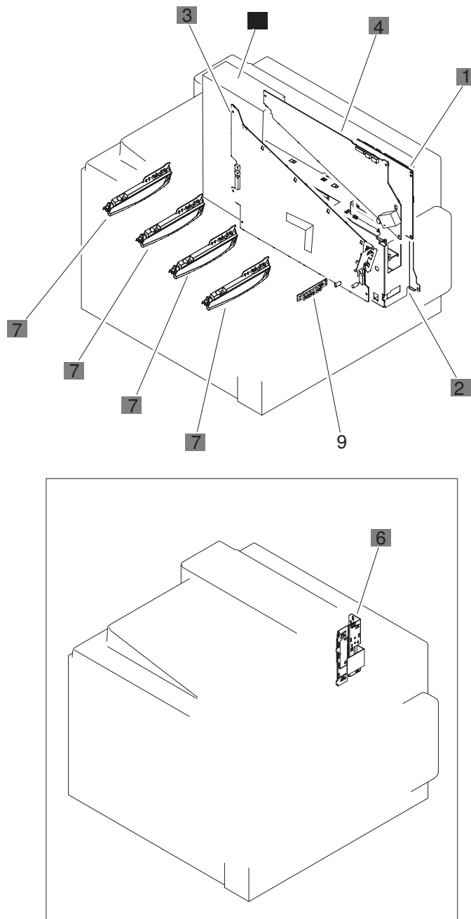
Figure 4-18 PCAs
