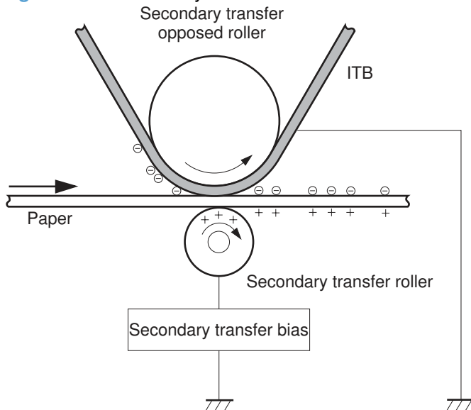
Figure 1-18 Secondary transfer
