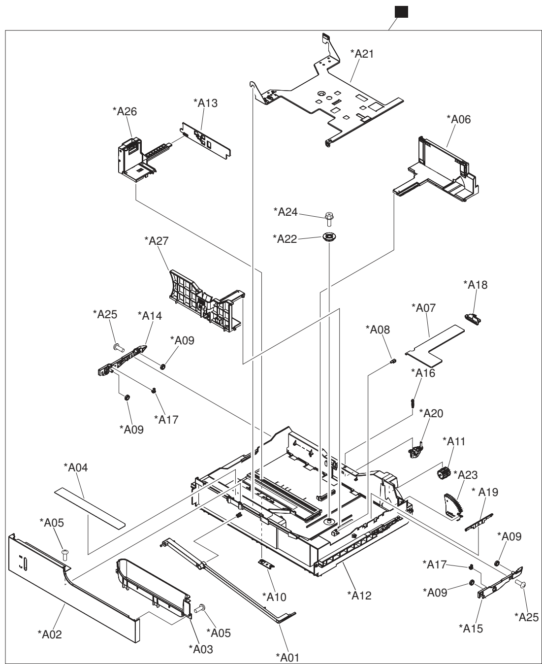
Figure 4-11 Cassettes 2-5
