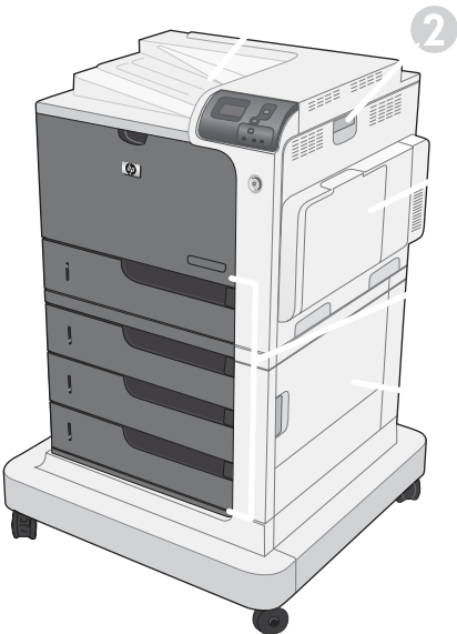
Figure 3-58 Jam locations
