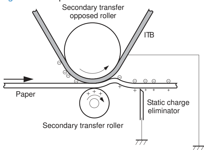
Figure 1-19 Separation
