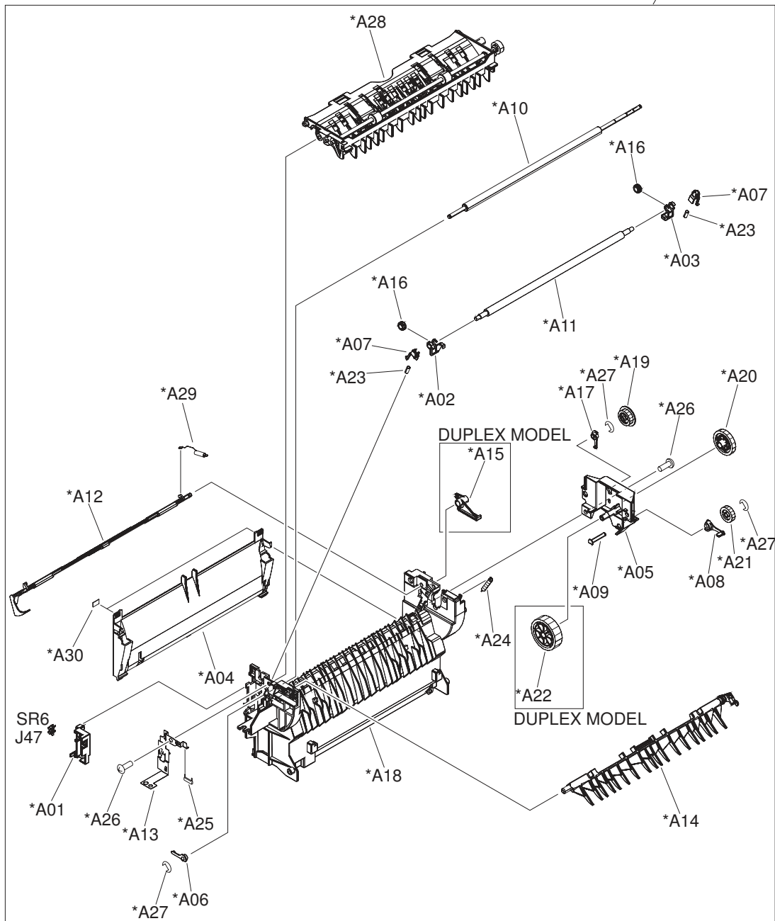
Figure 4-16 Delivery assembly
