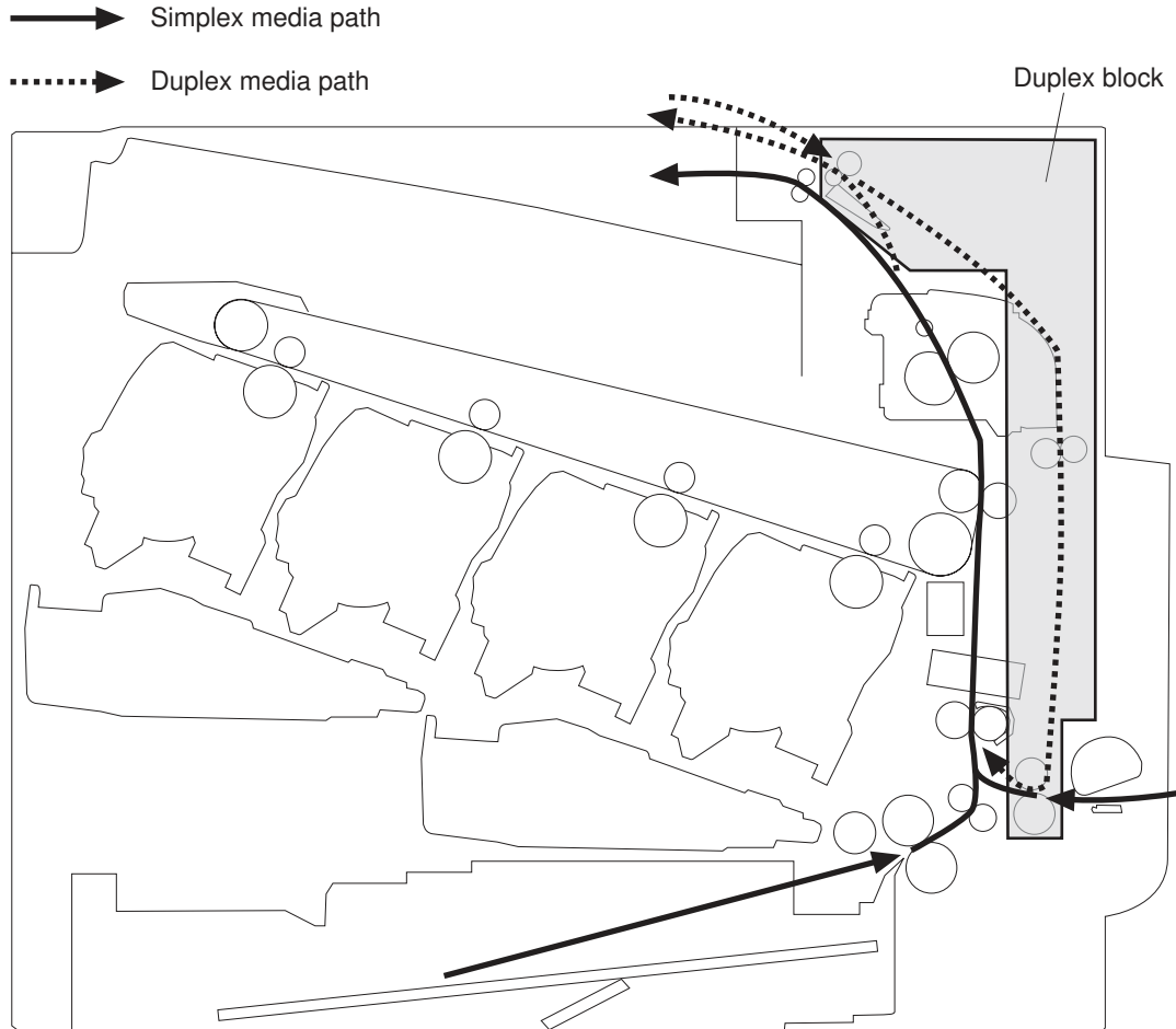
Figure 1-43 Duplexing unit
