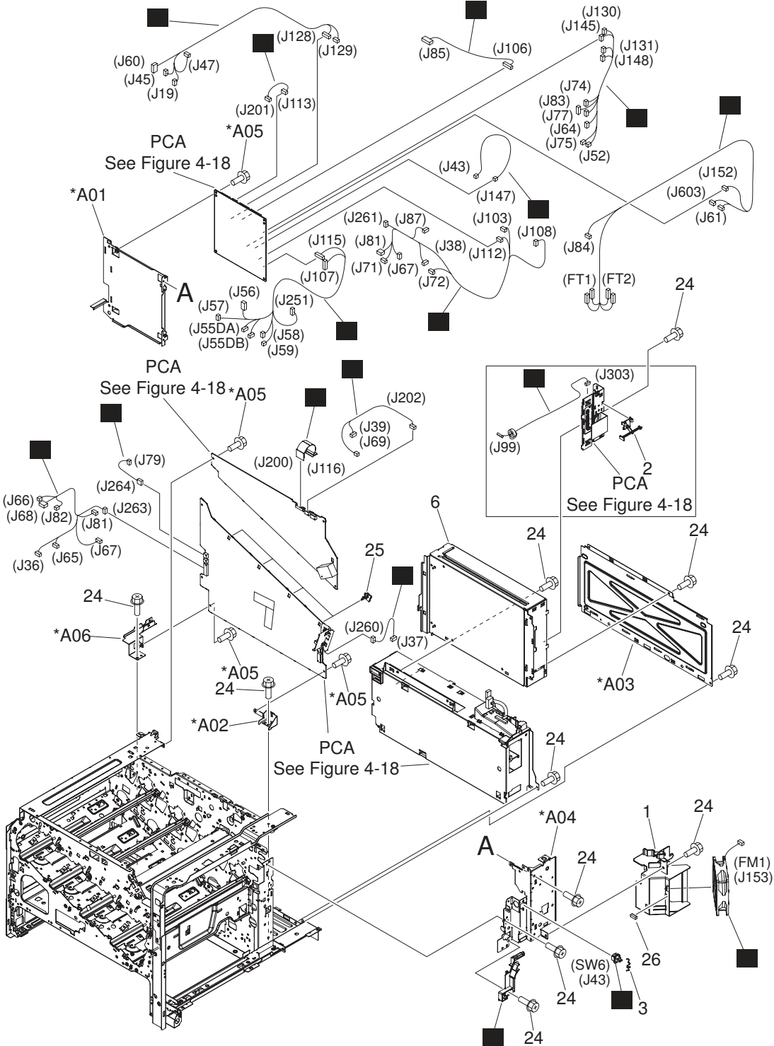
Figure 4-10 Internal components 7 of 7
