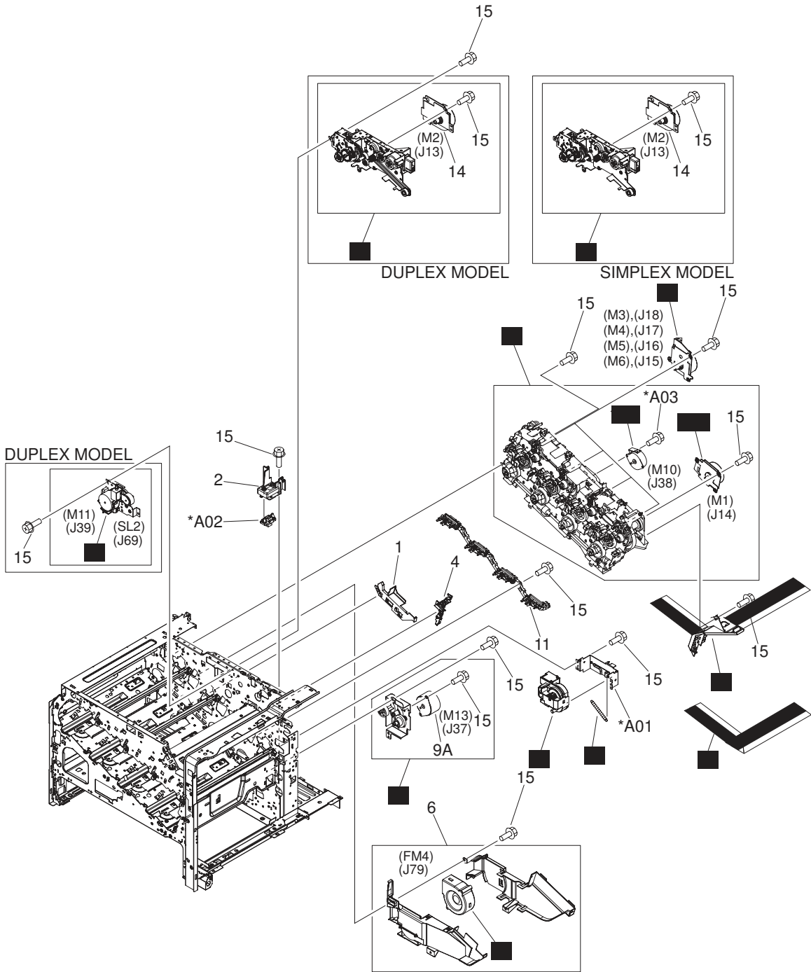
Figure 4-9 Internal components 6 of 7
