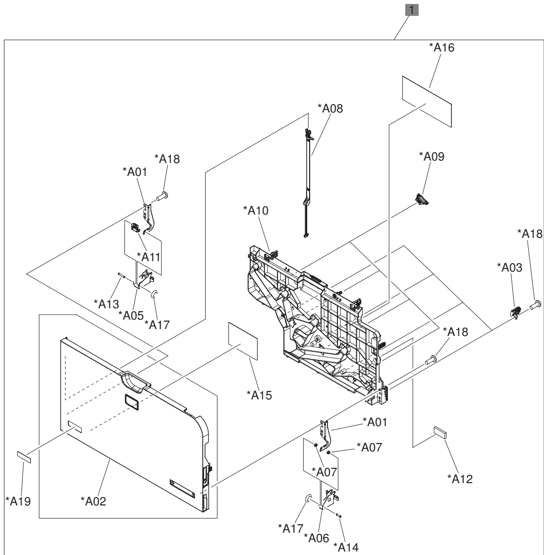
Figure 4-3 Front door assembly
