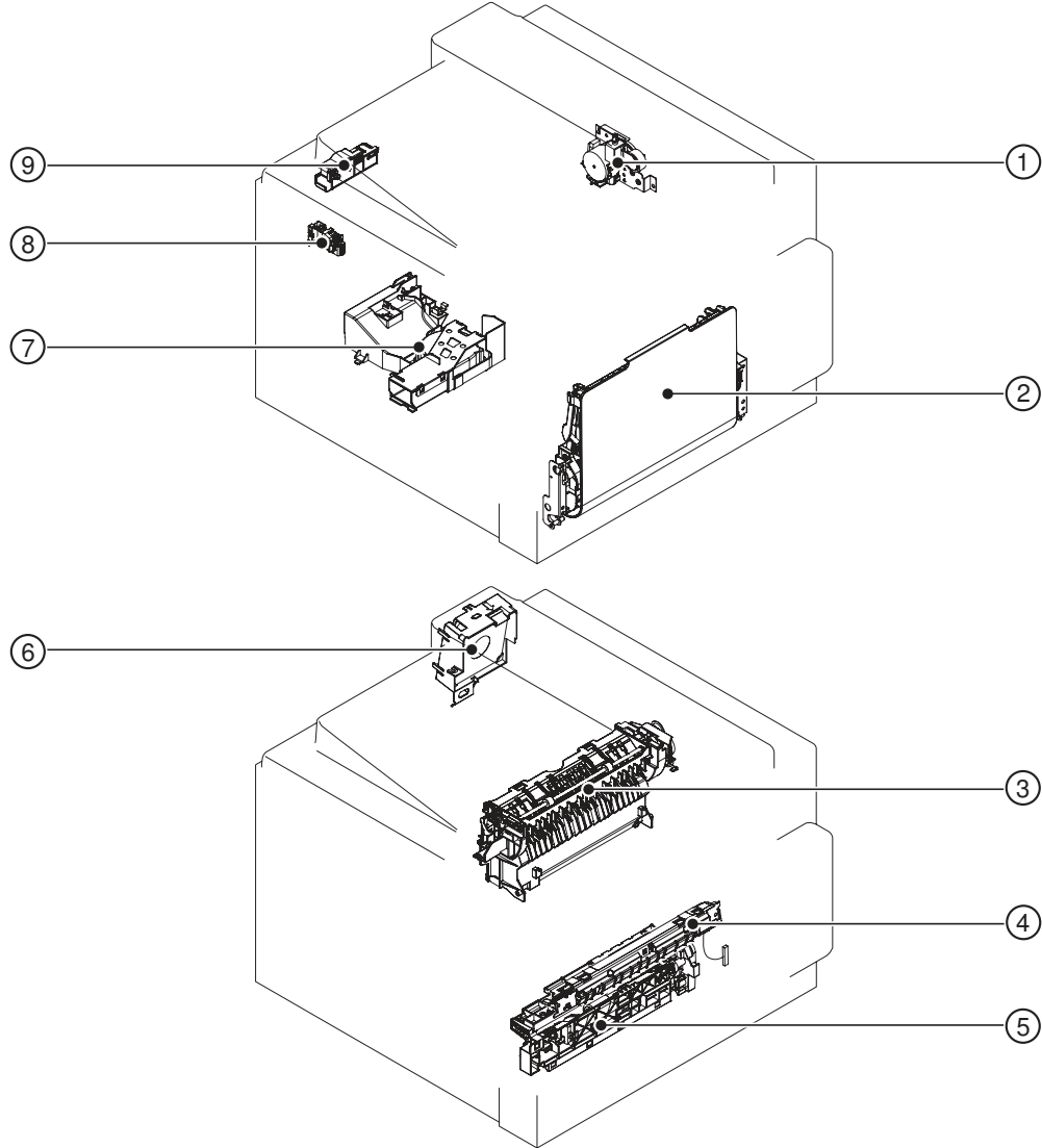
Figure 3-35 Major component locations (2 of 3)
