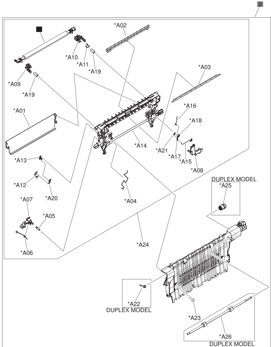
Figure 4-15 Secondary transfer assembly
