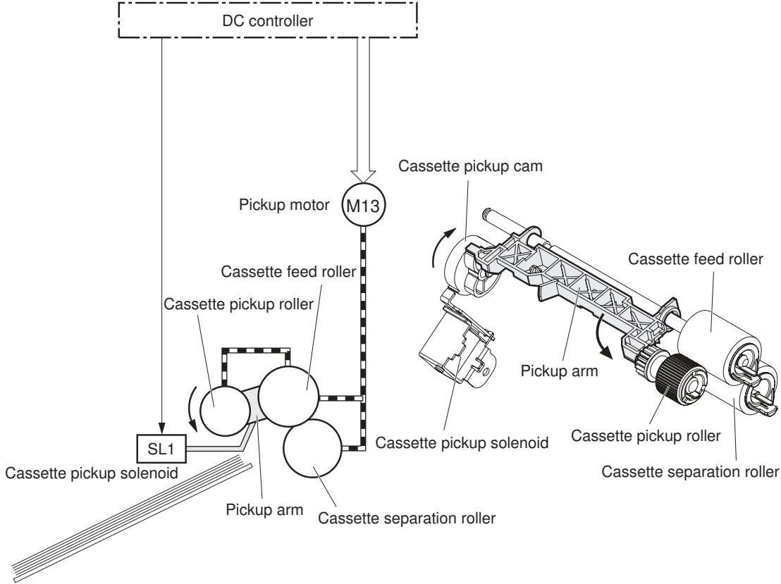
Figure 1-34 Cassette-pickup mechanism
