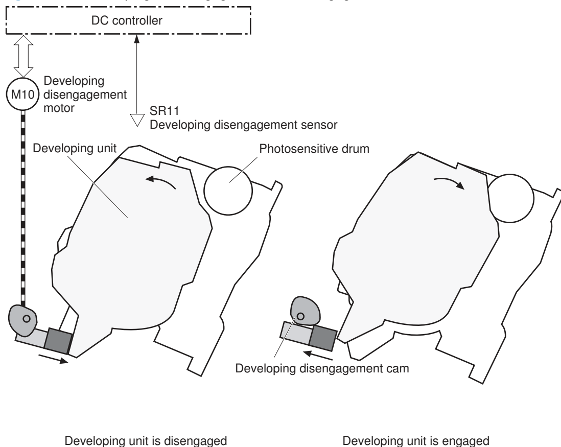
Figure 1-24 Developing-roller engagement and disengagement control
