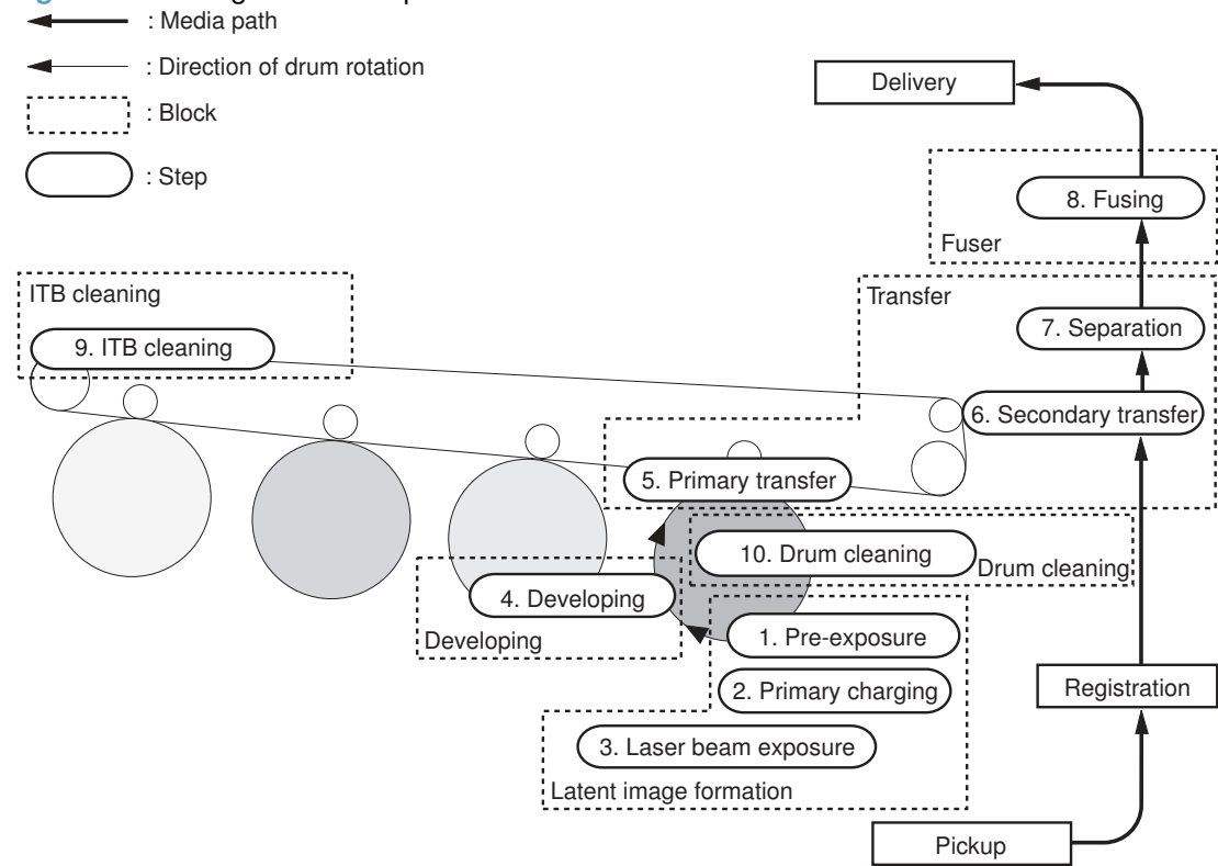
Figure 1-12 Image-formation process
