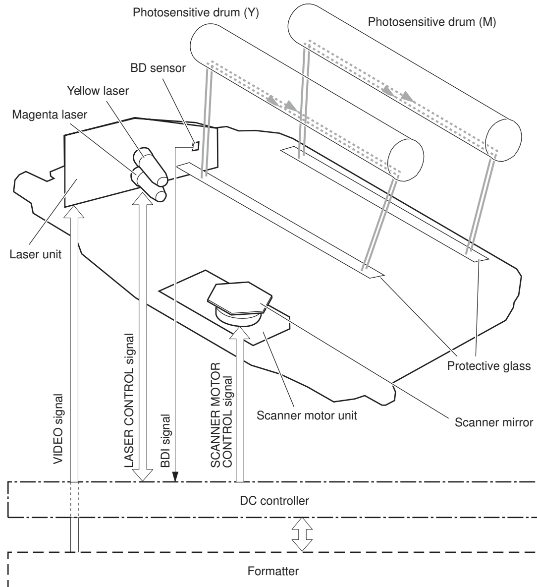
Figure 1-8 Laser/scanner system
