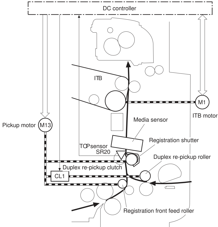
Figure 1-38 Paper-feed mechanism
