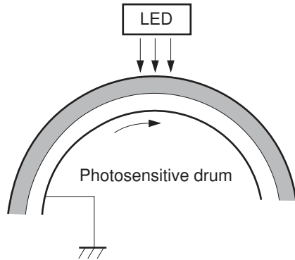
Figure 1-13 Pre-exposure
