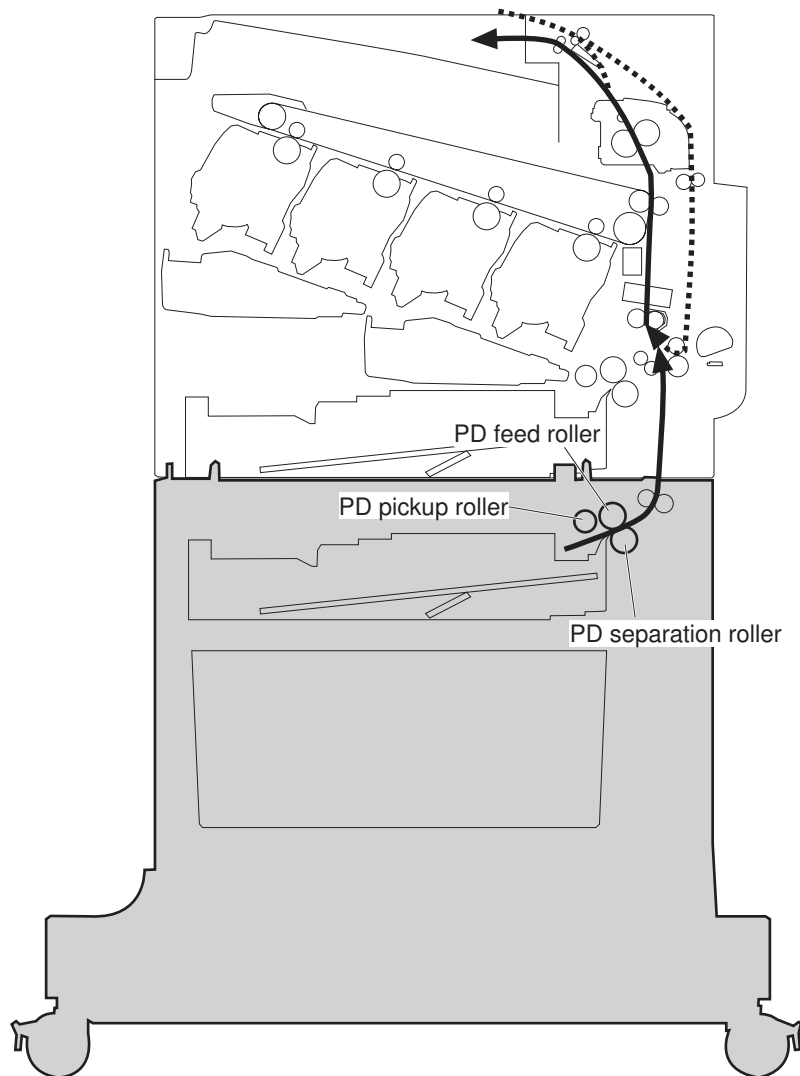
Figure 1-46 1 x 500 optional paper feeder
