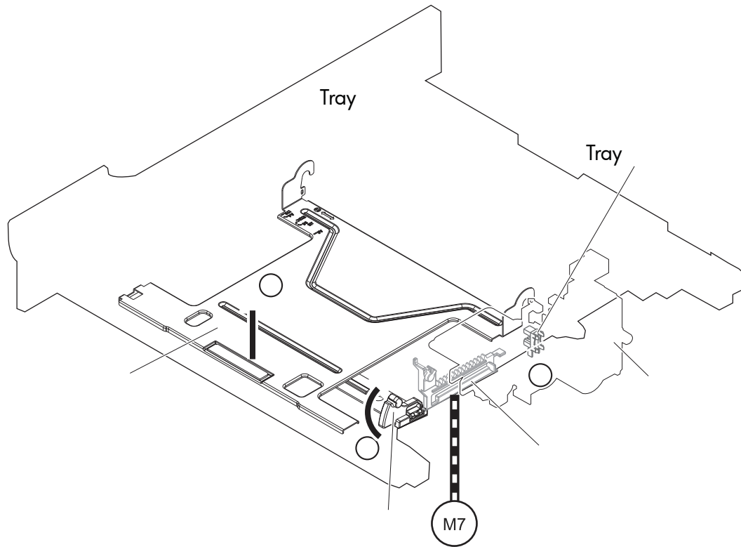
Figure 1-33 Tray lift mechanism
