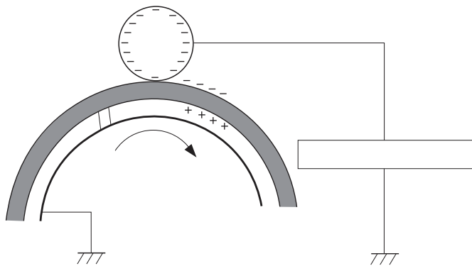
Figure 1-12 Primary charging
