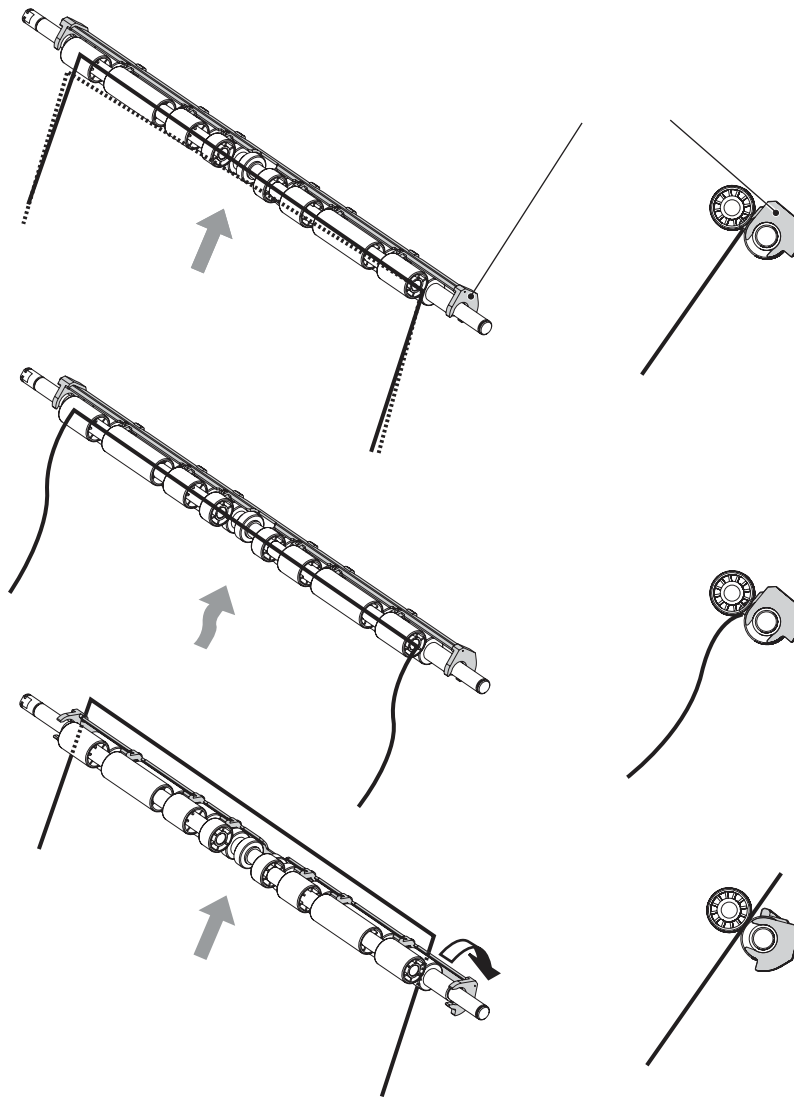
Figure 1-38 Skew-feed prevention
