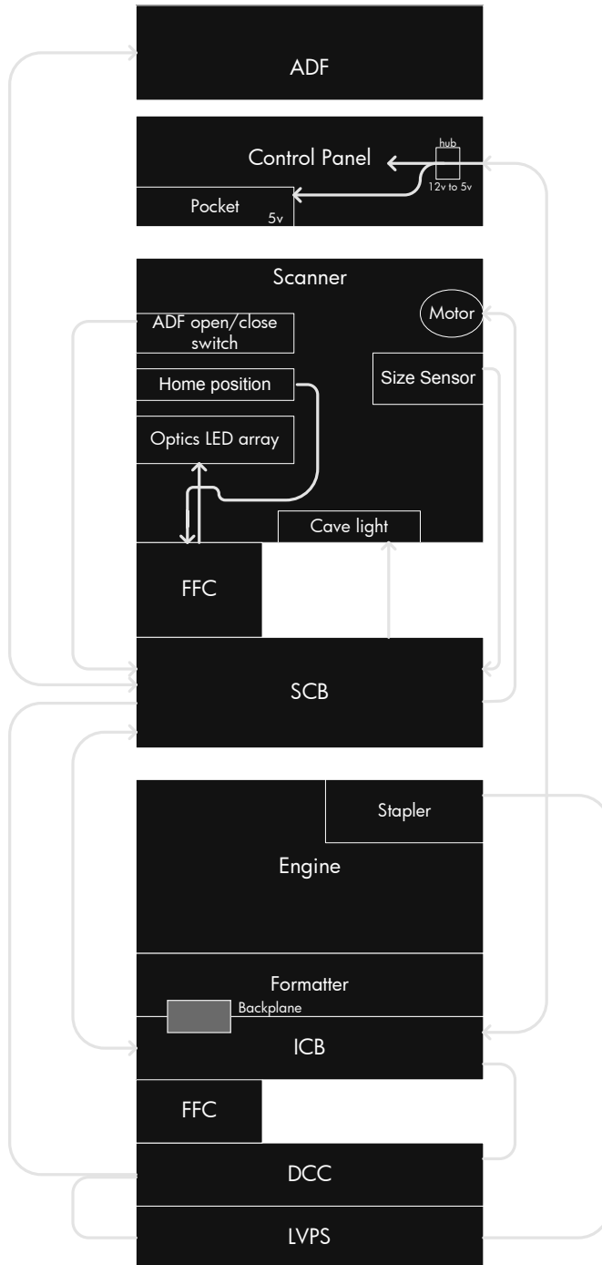
Figure 2-40 Product circuit block diagram
