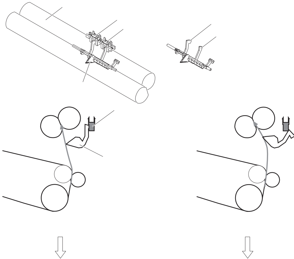
Figure 1-40 Loop-control mechanism
