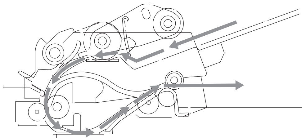
Figure 1-51 ADF path for single-sided documents
