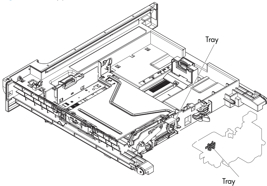
Figure 1-32 Tray presence sensor
