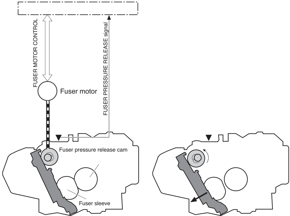
Figure 1-41 Pressure-roller pressurization control
