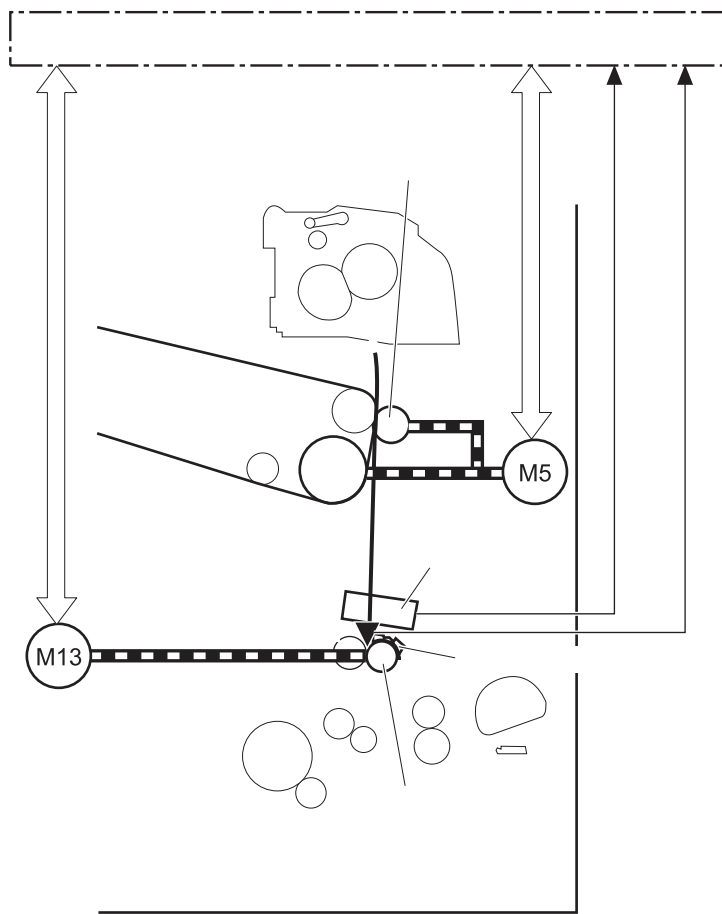
Figure 1-37 Paper-feed mechanism
