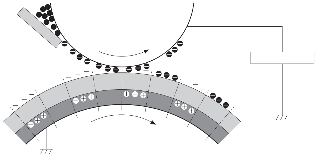
Figure 1-14 Development
