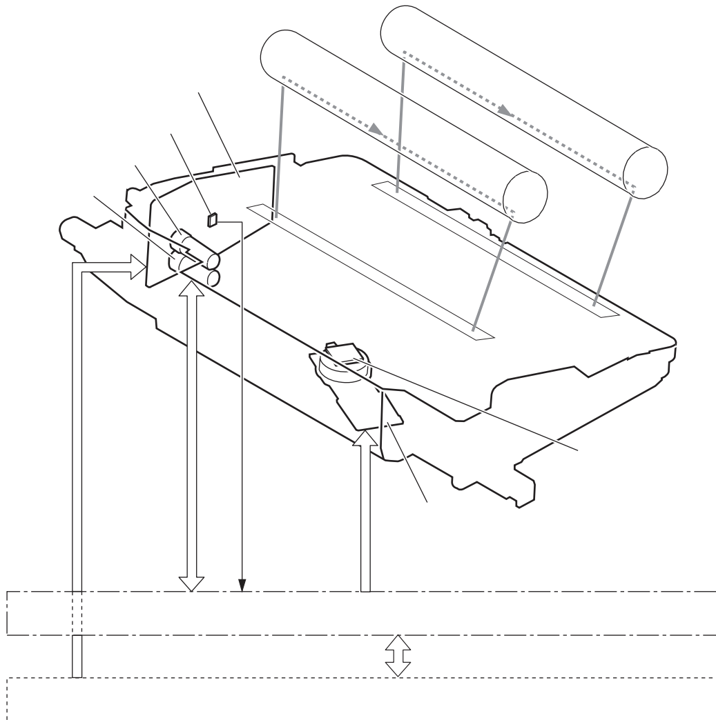
Figure 1-8 Laser/scanner system
