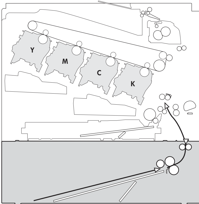
Figure 1-50 Jam detection
