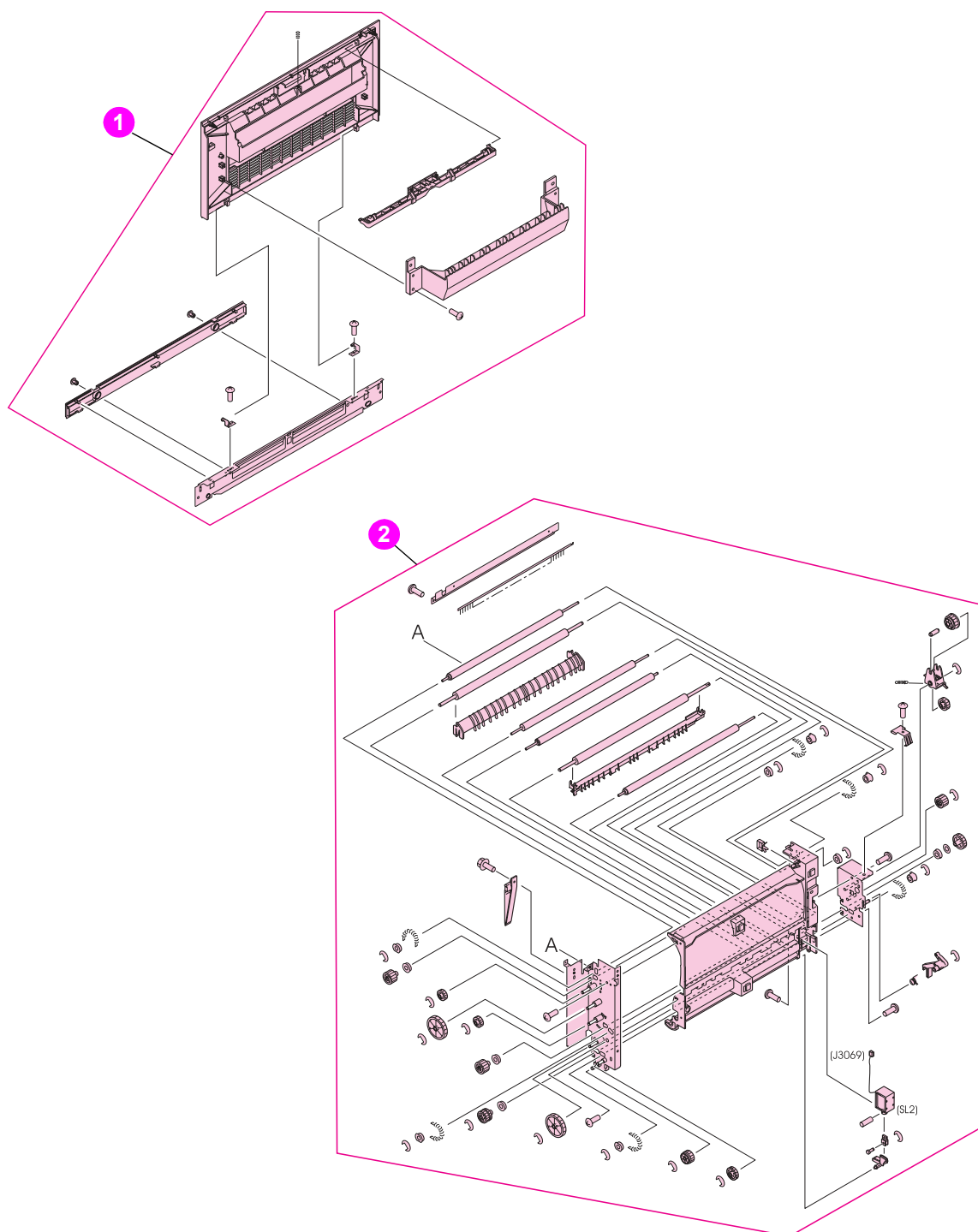
Figure 311. Parts that are unique to the MFP (2 of 2)
