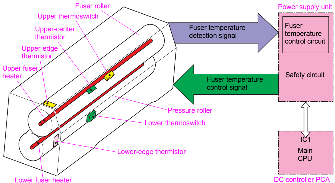
Fuser control circuit
