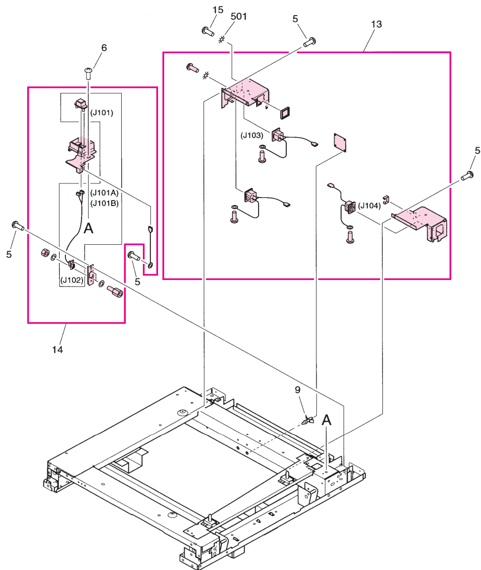
Figure 347. Pedestal main body (1 of 2)
