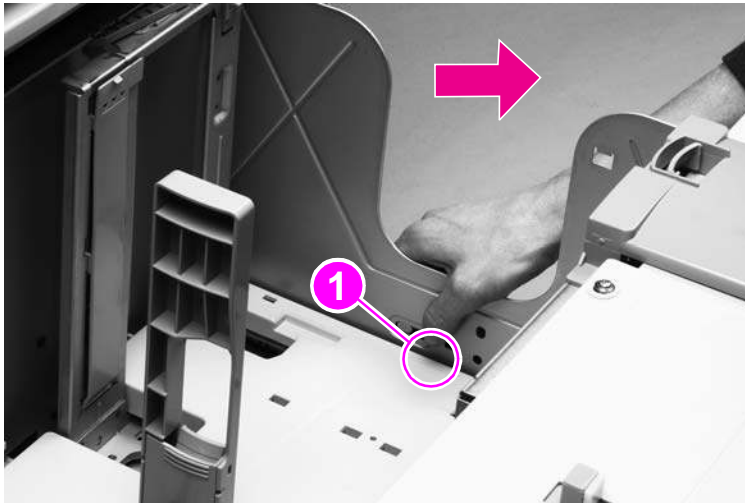
Figure 260. Removing tray 4
