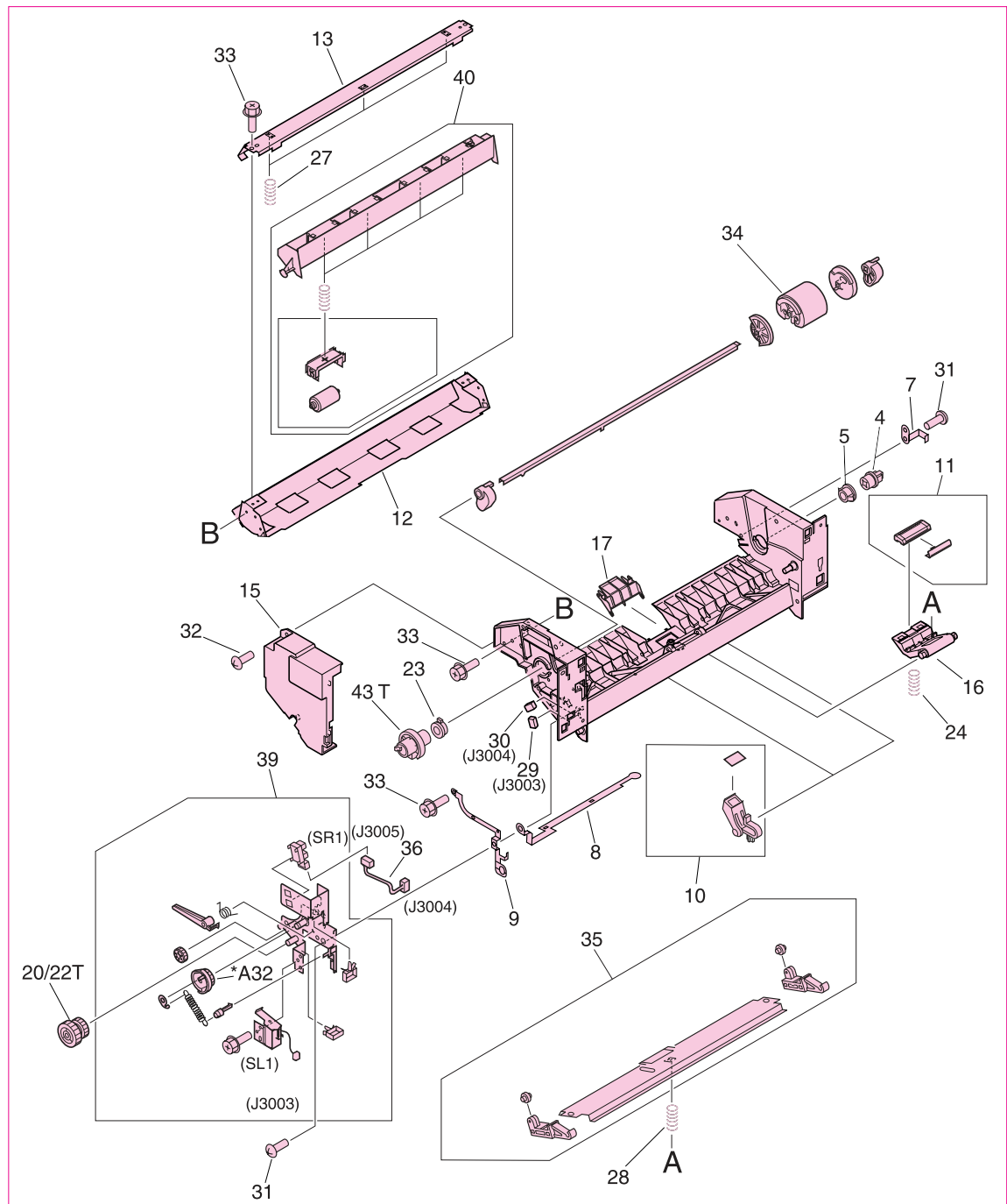
Figure 333. Manual feed pickup assembly (tray 1) (1 of 2)
