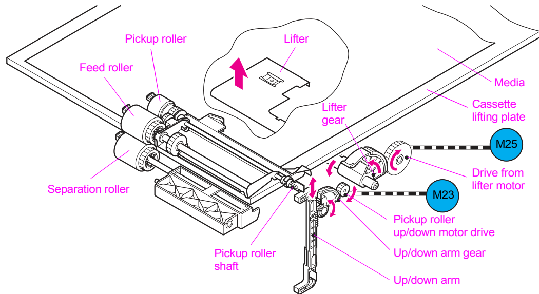
Figure 66. Lifting-up operation
