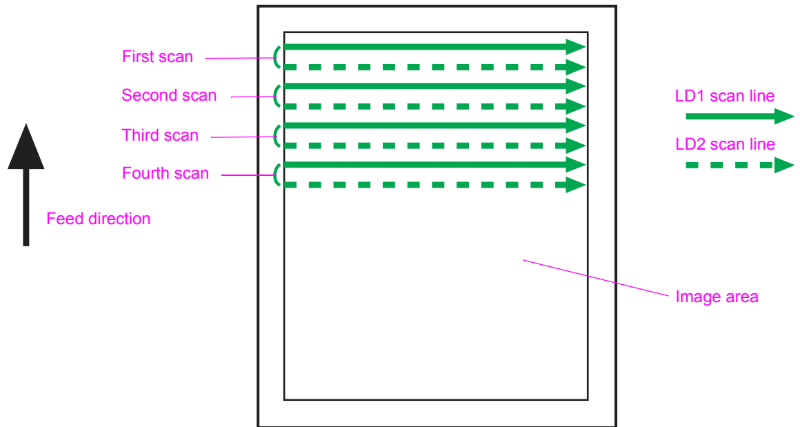
Figure 43. Dual-beam method
