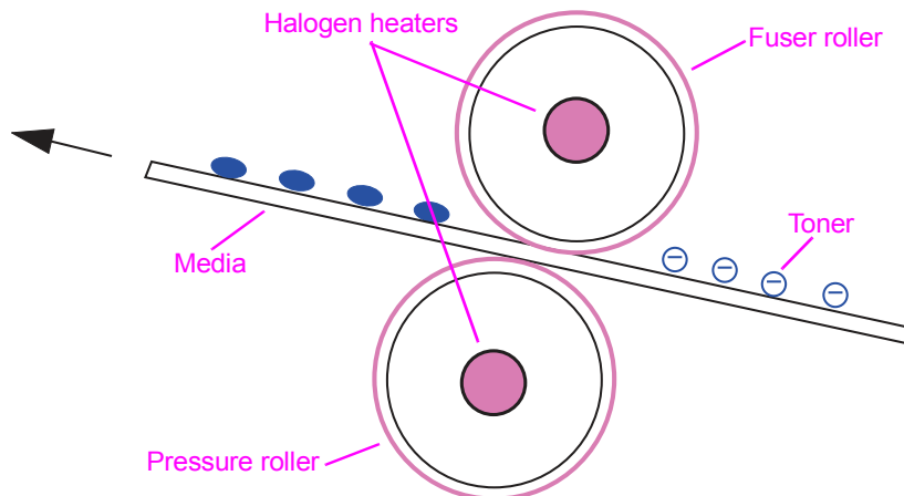
Figure 57. Fusing (step 8)
