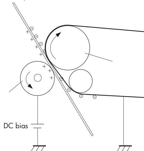
Figure 1-14 Secondary transfer
