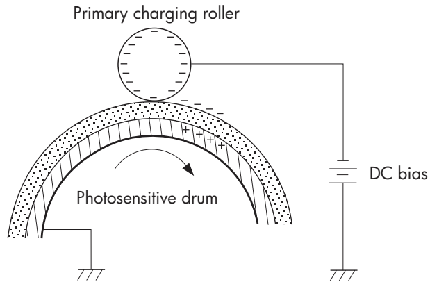
Figure 1-10 Primary charging
