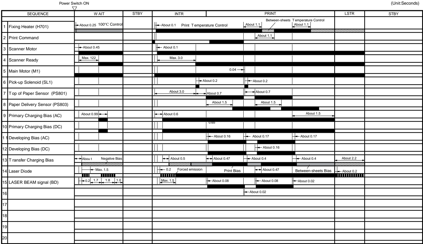
Figure 4-8 Printer timing diagram
