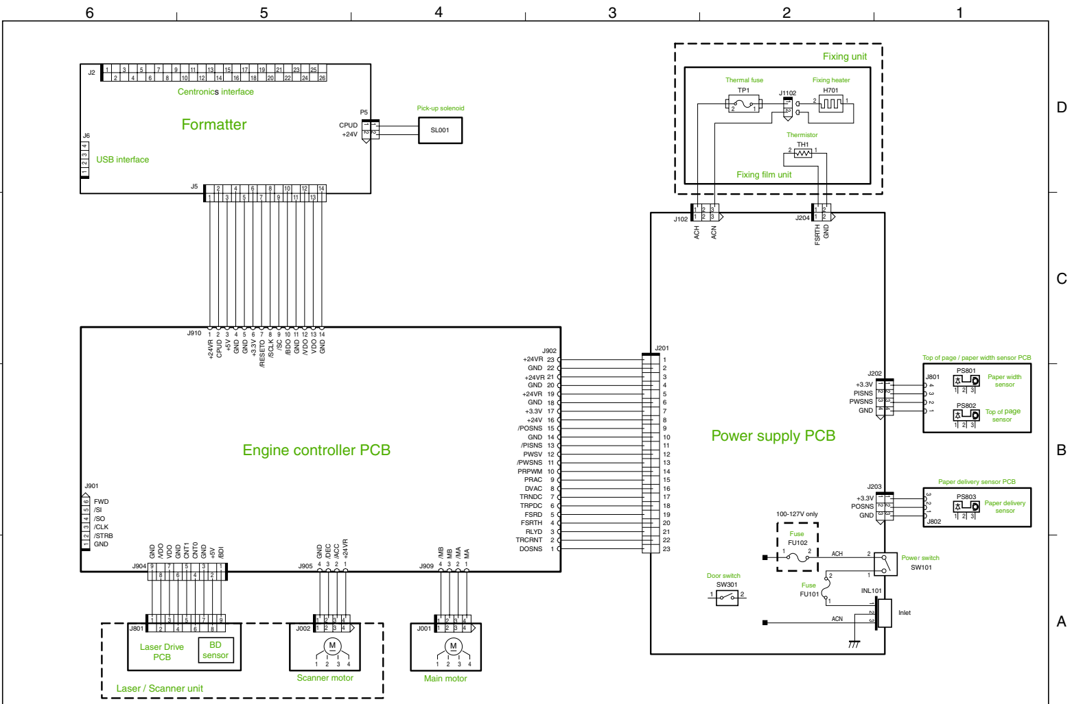
Circuit diagram
