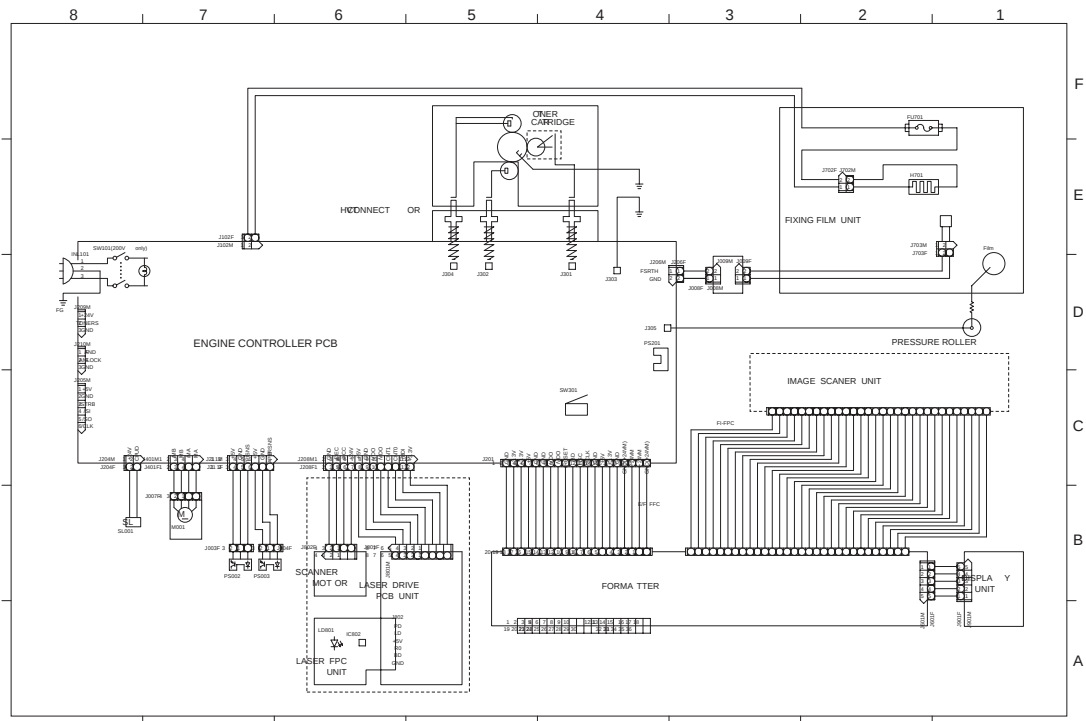
Figure 5-12 Main wiring
