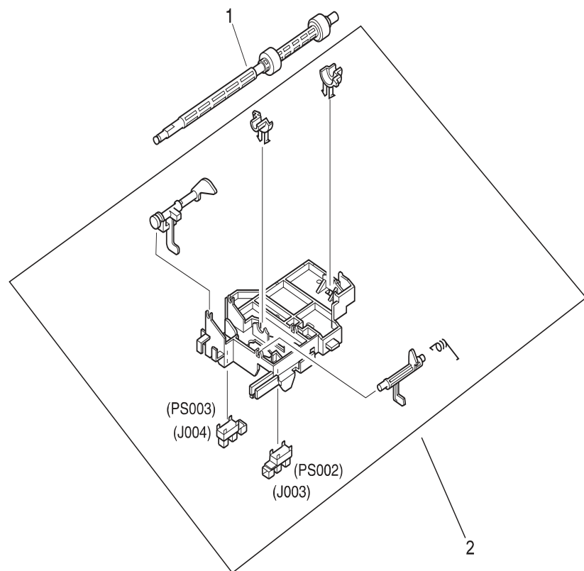
Figure 6-7 Feeder assembly
