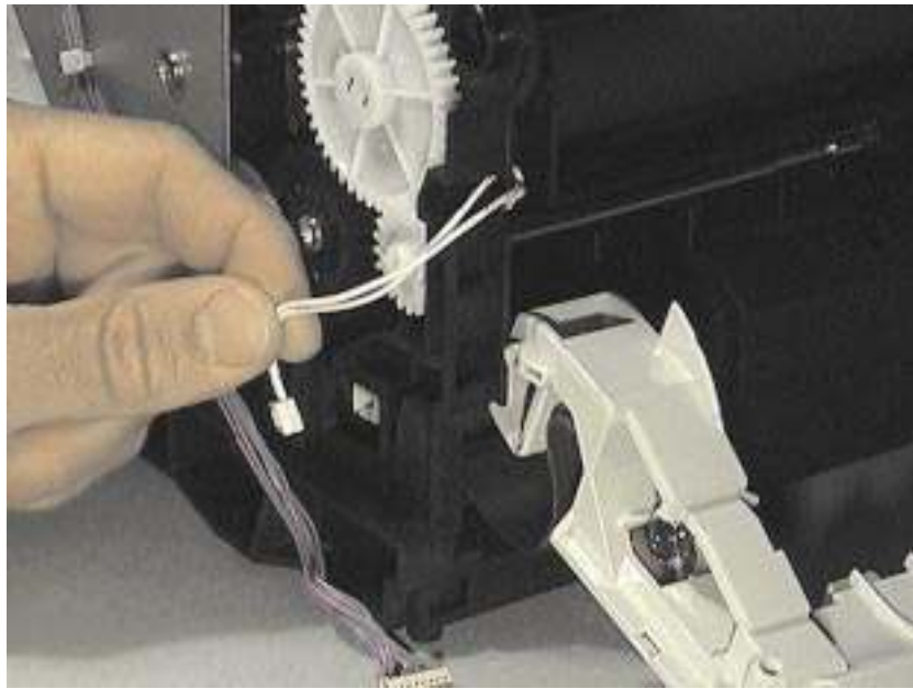
Figure 5-3 Thermistor Connector
