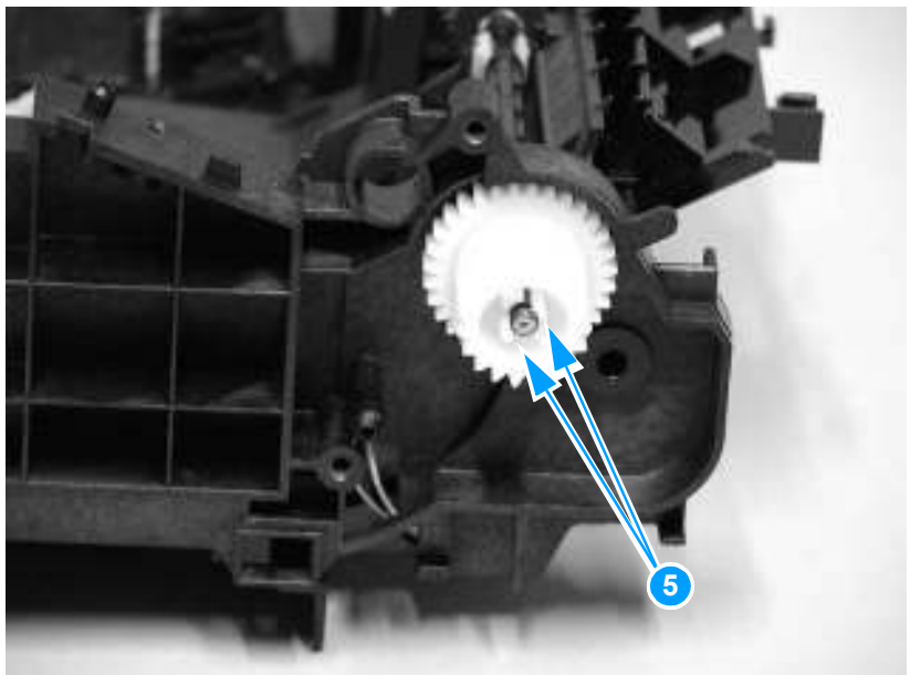
Figure 77. Removing the paper-feed roller (4 of 5)
