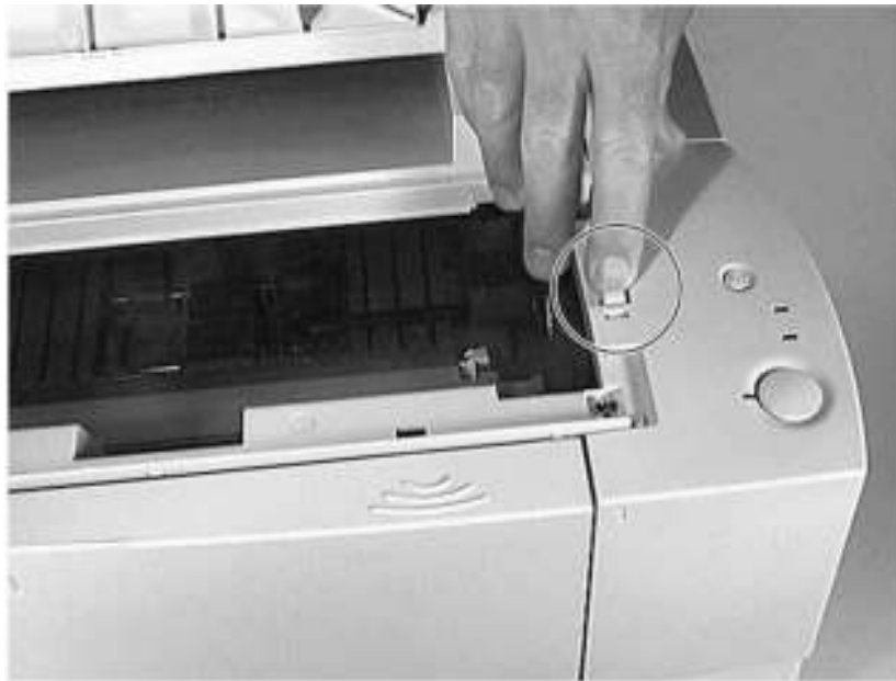
Figure 7-24 DIMM Cover Release Button
