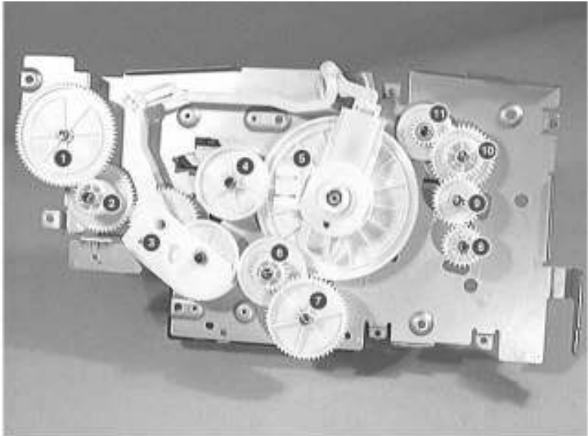
Figure 7-78Printer Drive Assembly
