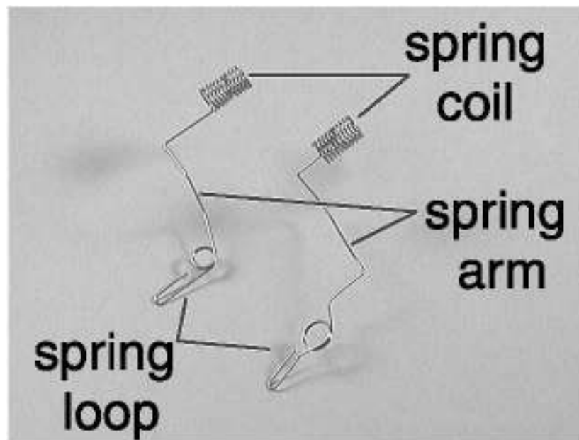
Figure 7-122 Parts of the DC Bias Voltage Contacts (Leaf Springs)
