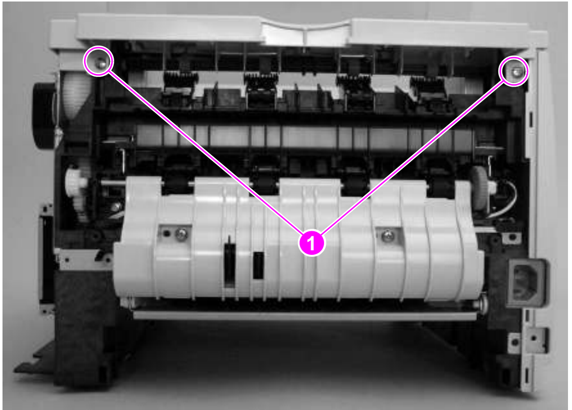
Figure 47. Removing the top-cover assembly (2 of 3)
