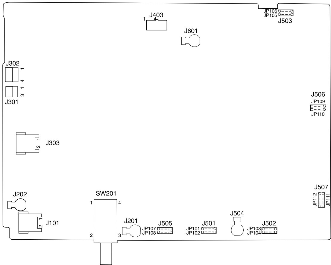
Figure 118. Power supply PCB
