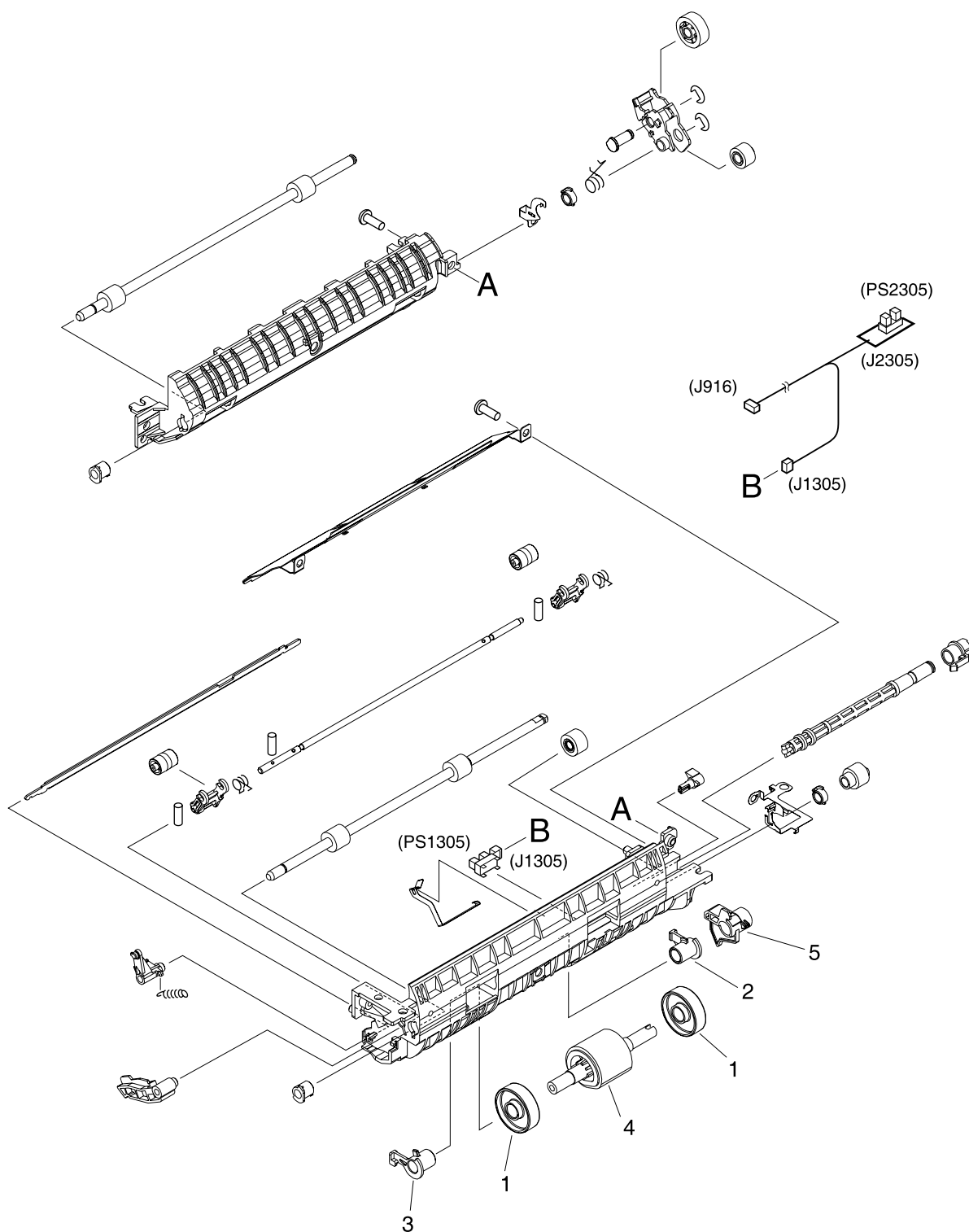
Figure 130. Pickup assembly
