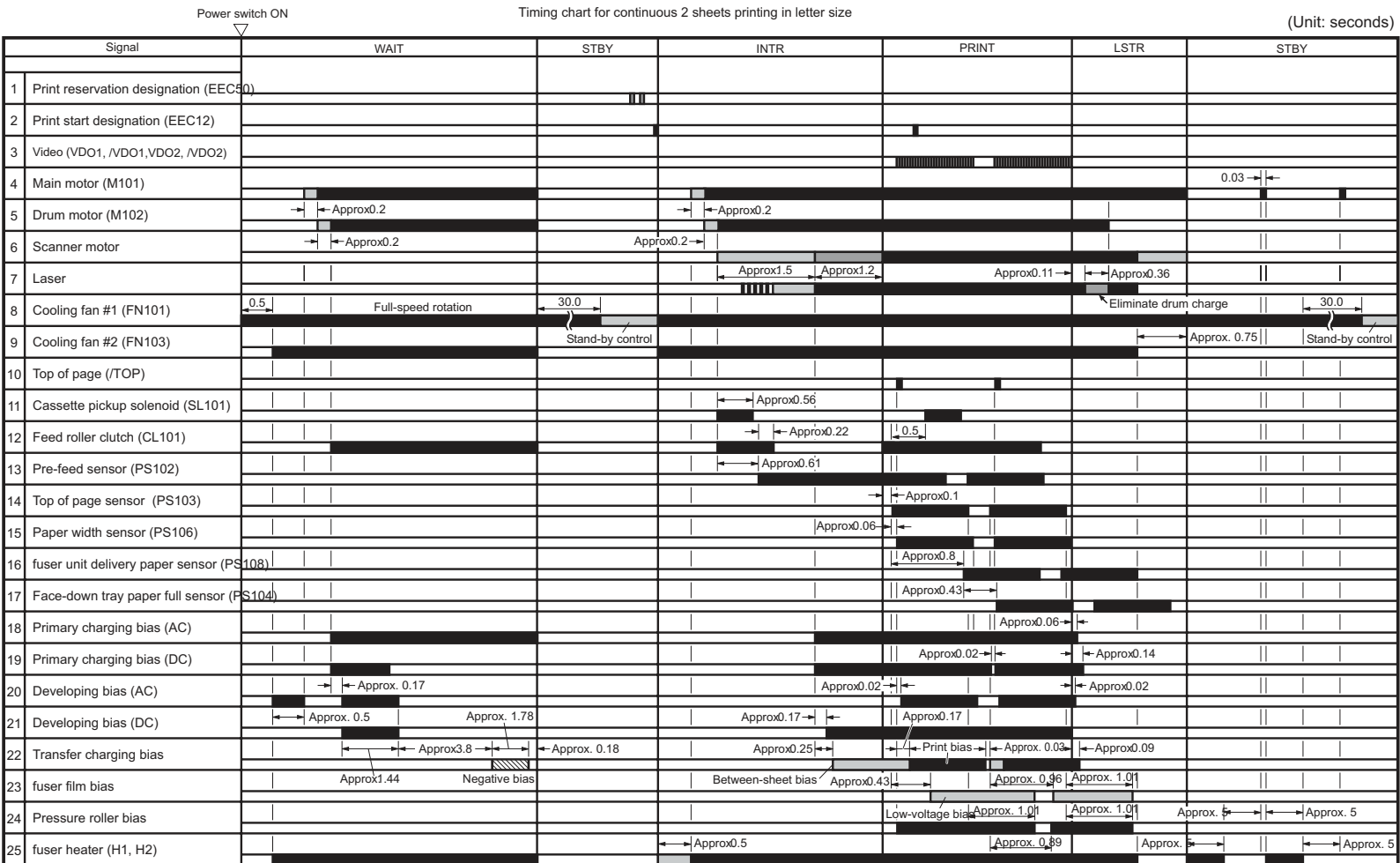
Figure 7-38 HP LaserJet 4250 general timing diagram
