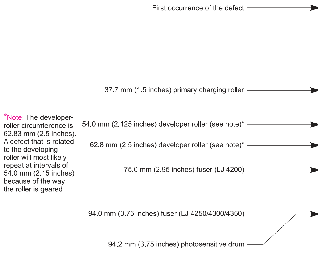
Figure 7-8 Repetitive-defect ruler
