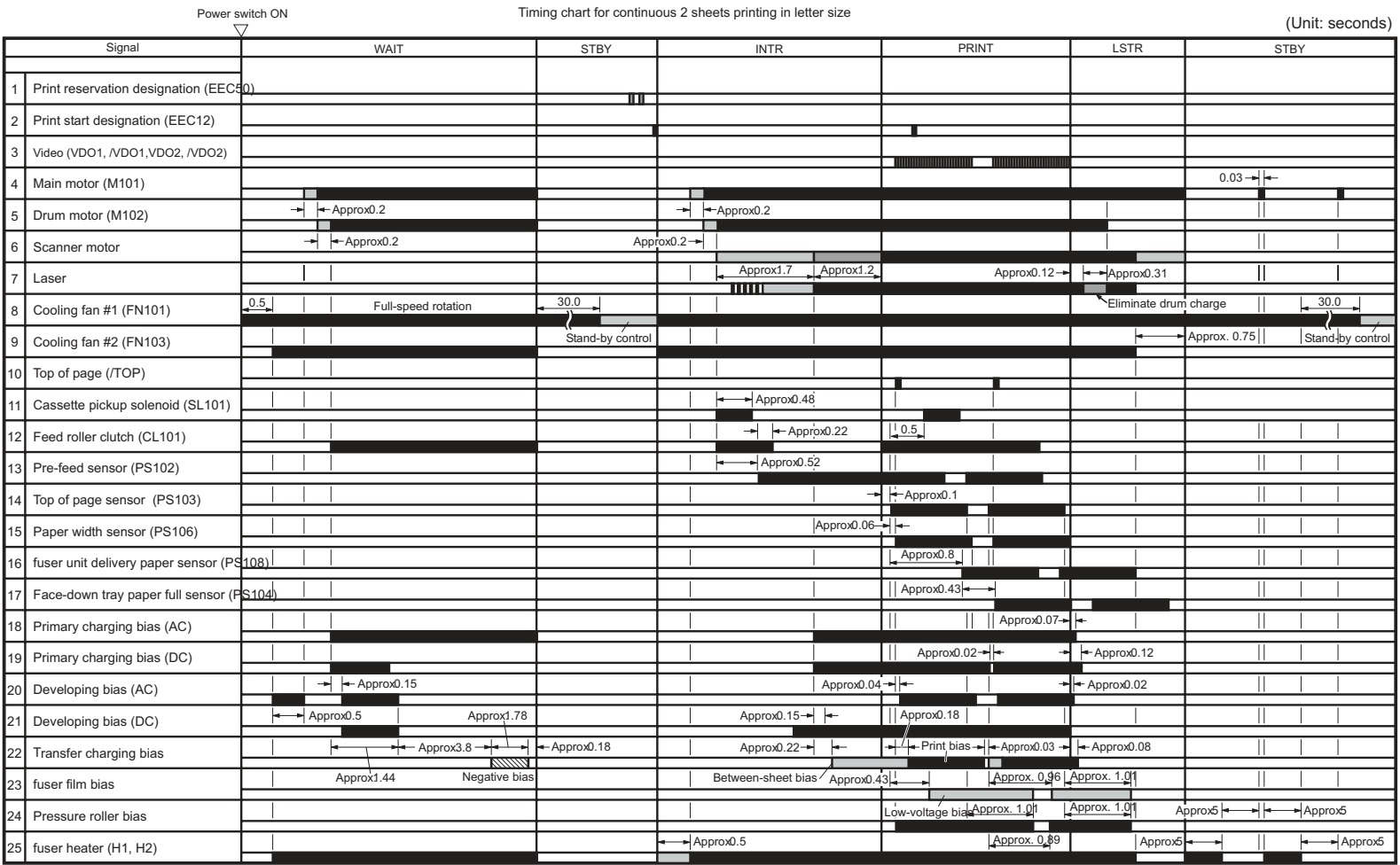
Figure 7-40 HP LaserJet 4350 general timing diagram
