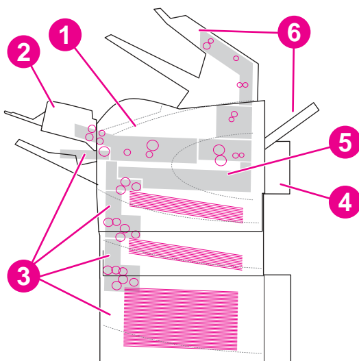
Figure 7-7 Jam locations
