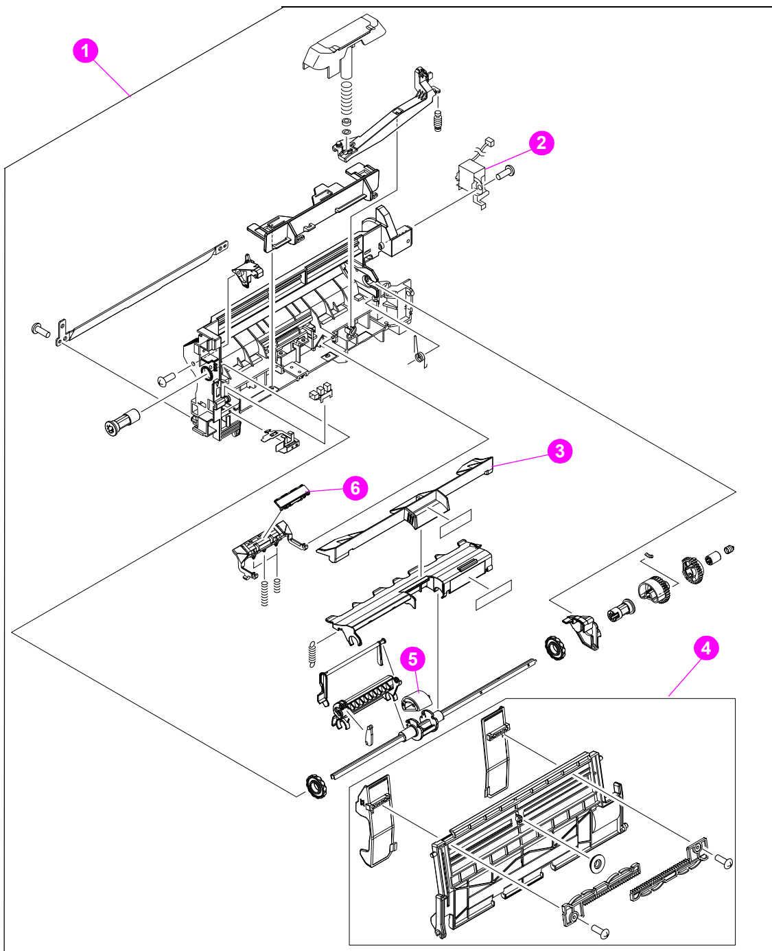
Tray 1 assembly
