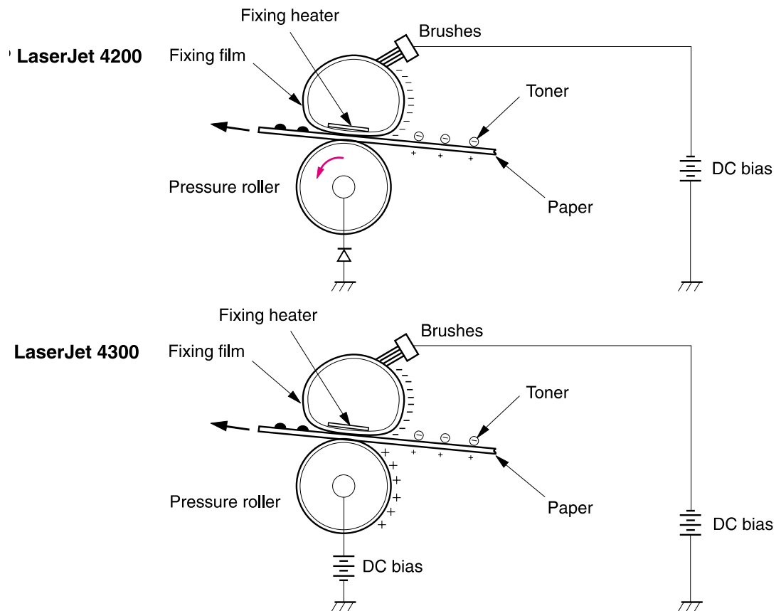
Fusing the image
