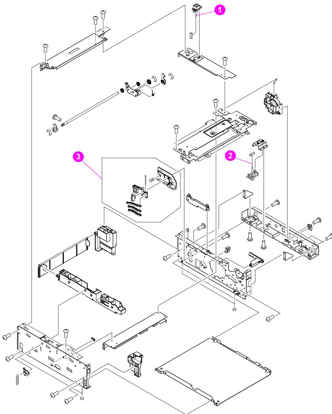
Figure 255. 500-sheet feeder main assemblies (1 of 2)
