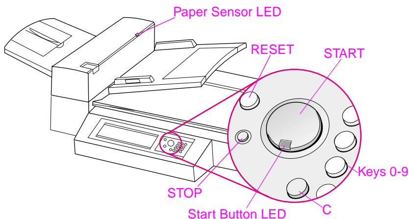
Figure 3-3 Button/LED Functions
