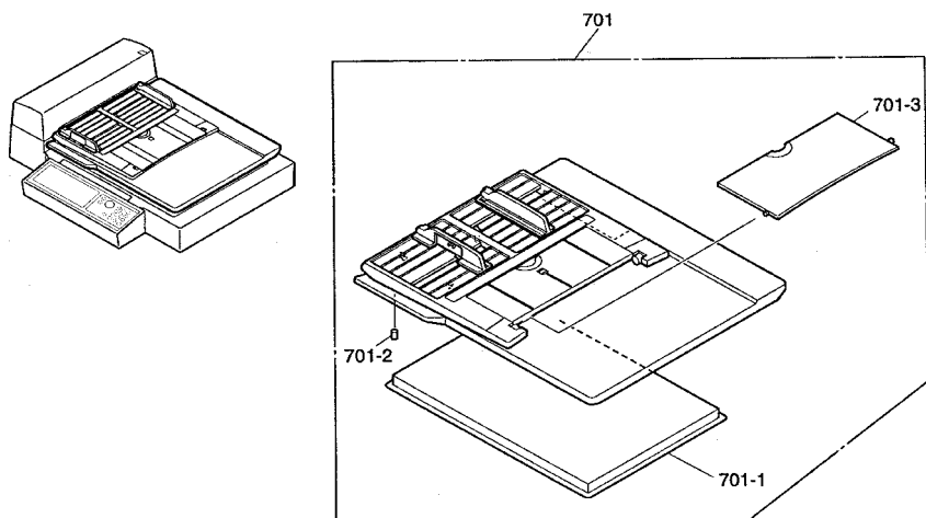
Figure 8-25 Document Cover Assembly
