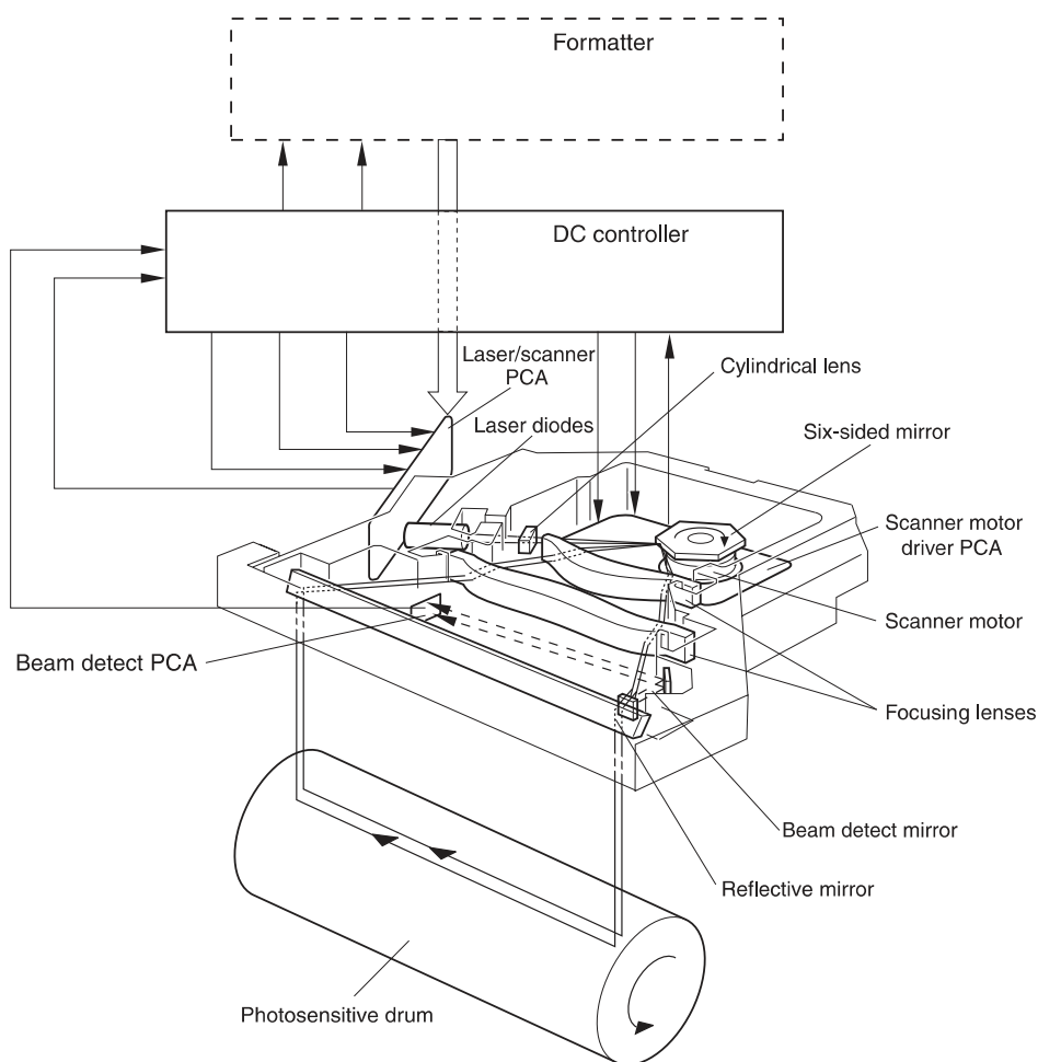
Figure 28. Laser/scanner system
