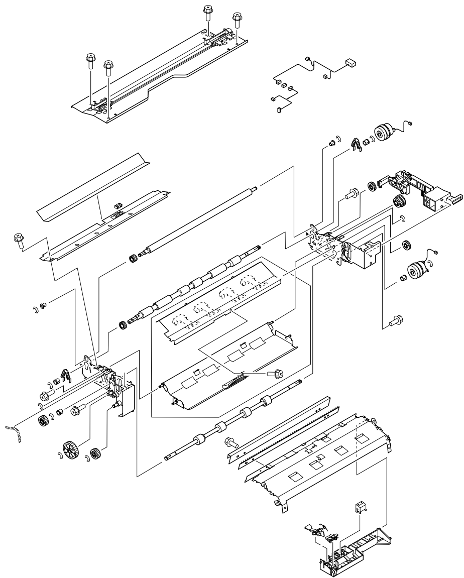
Figure 146. Registration assembly
