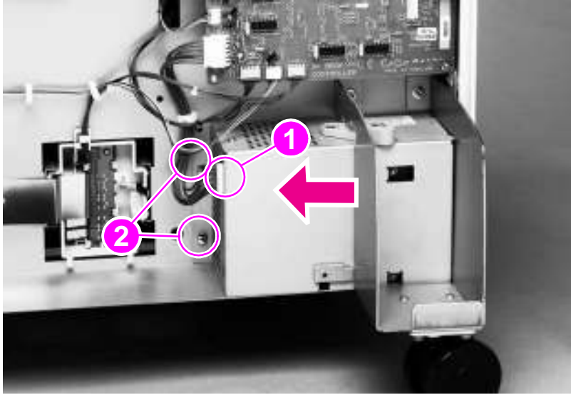
Figure 114. Power supply
