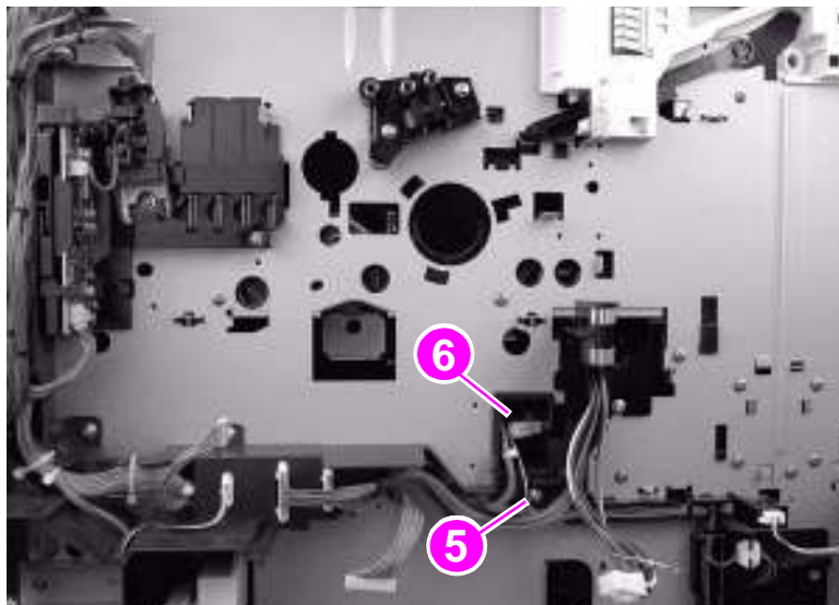
Figure 97. Fuser-connector holder assembly (3 of 3)
