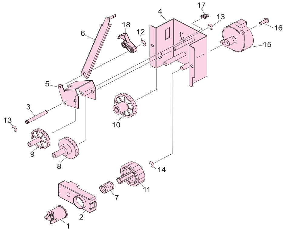
Figure 90. Lifter-driver assembly
