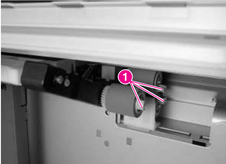
Figure 55. Remove the pickup, feed, and separation rollers
