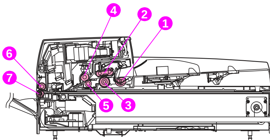
Figure 30. Mechanical structure (2 of 2)
