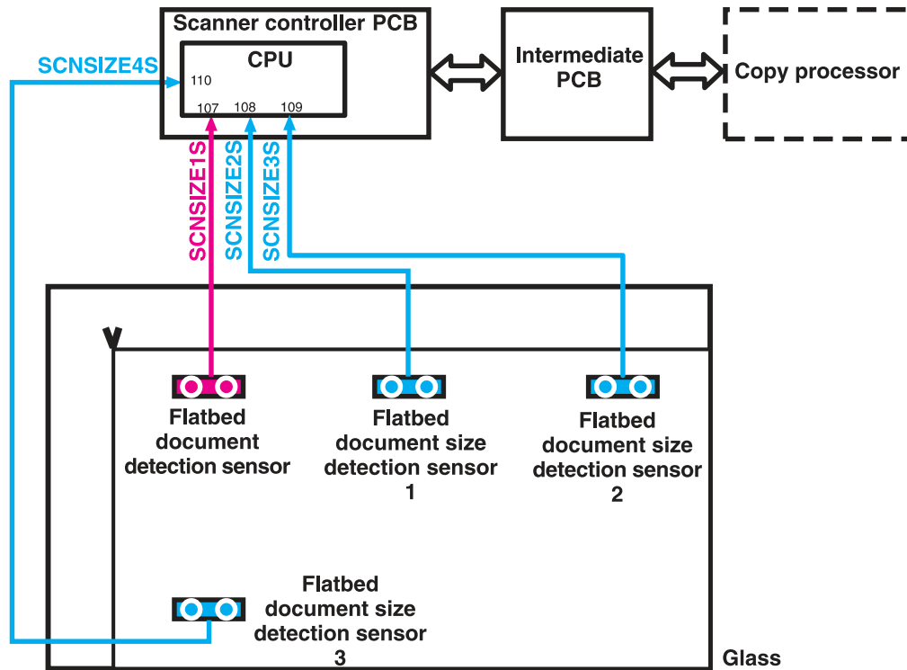
Figure 43. Flatbed document size detection
