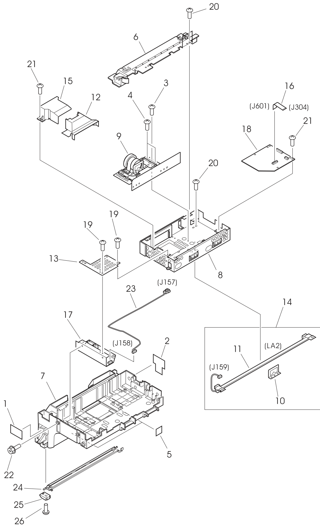
Figure 243. ADF optical assembly
