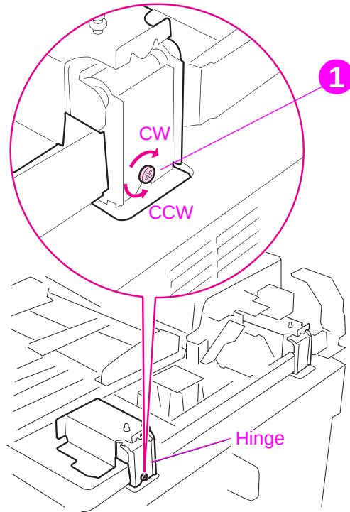
Figure 220. ADF skew adjustment (2 of 3)
