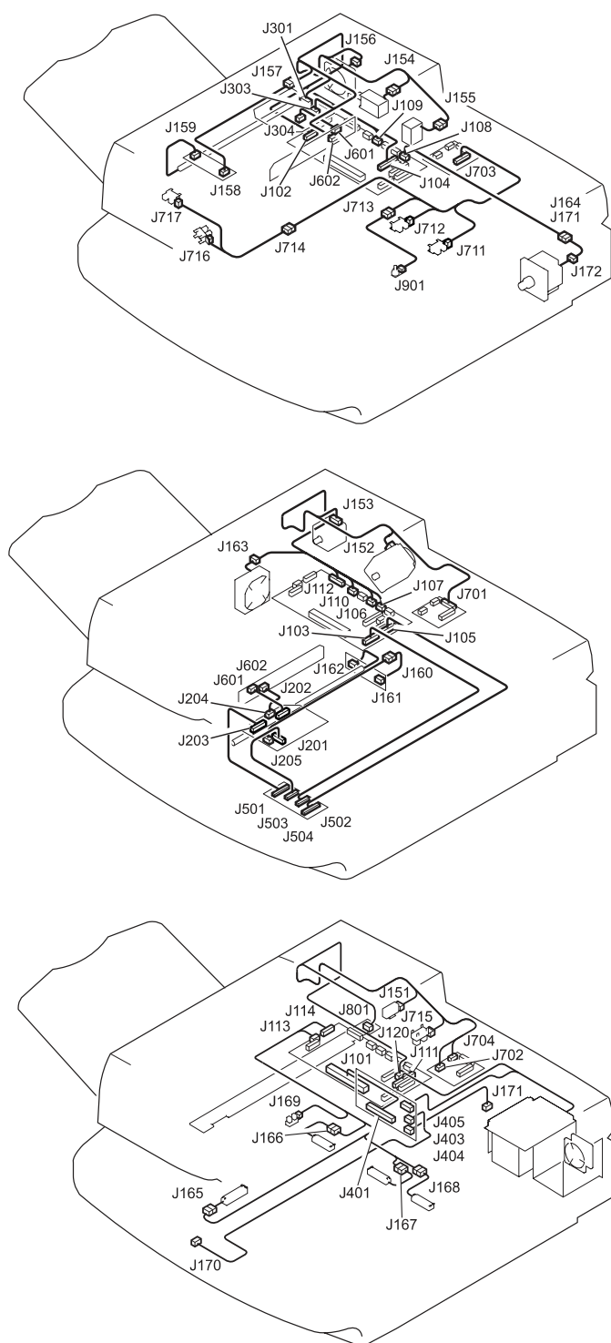
Figure 229. Connector locations
