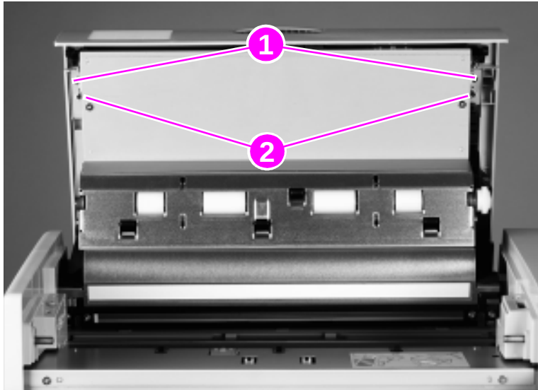
ADF feeder cover (1 of 3)
