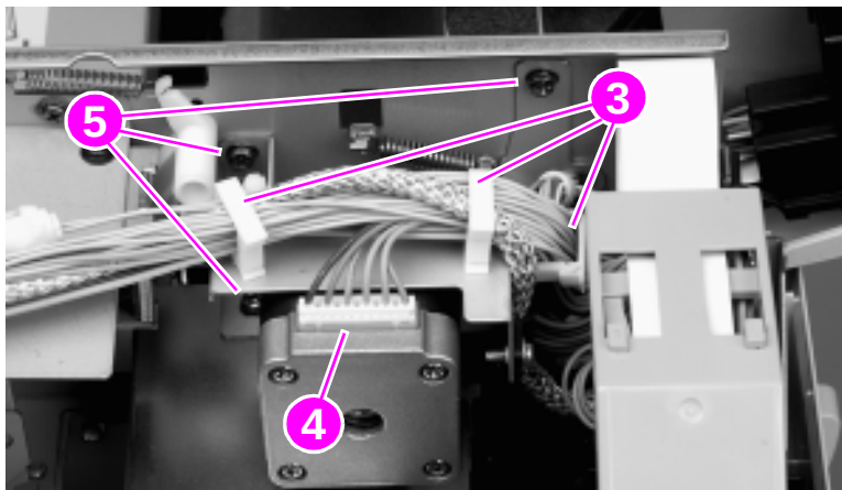
Figure 136. Delivery motor (2 of 2)
