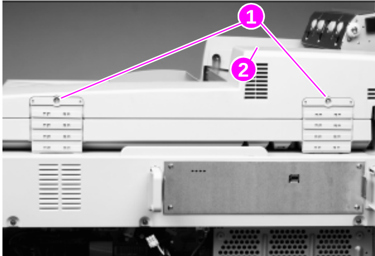
ADF back cover (1 of 2)
