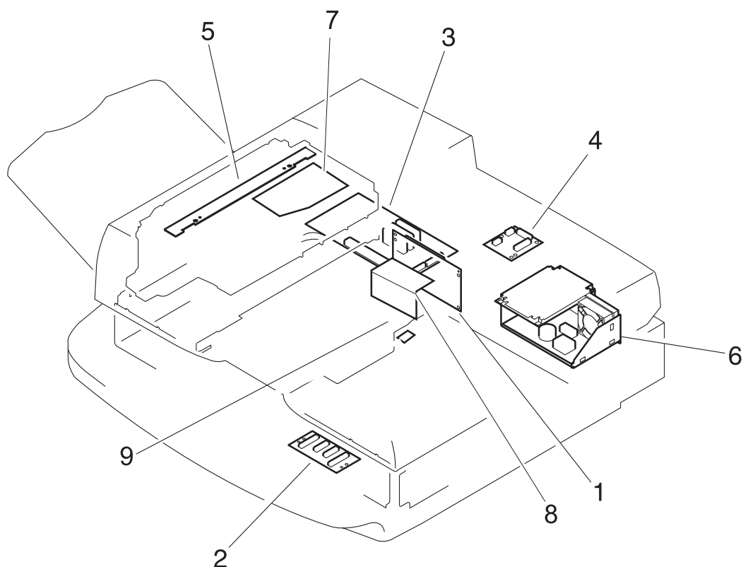
Figure 244. PCB assemblies
