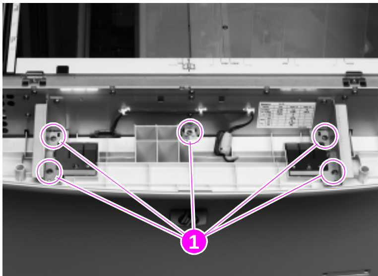
Flatbed lower front cover
