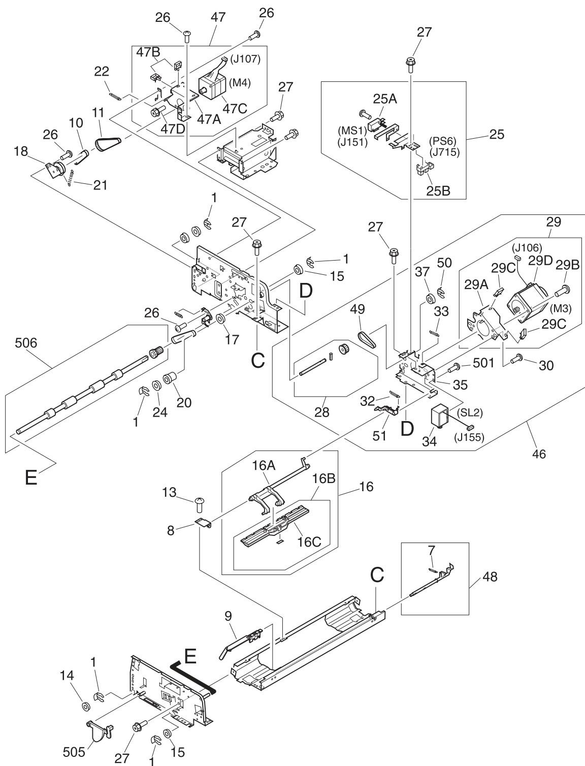
Figure 241. Paper pickup assembly (2 of 2)
