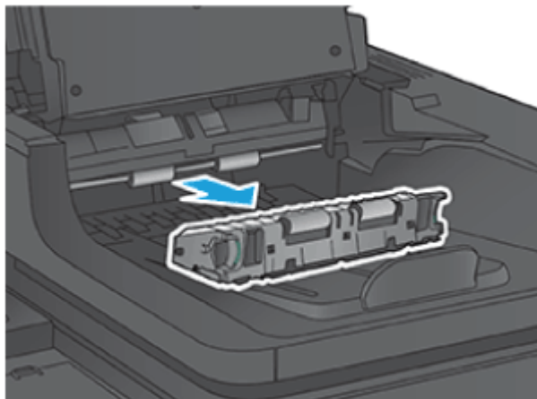
Figure 4-97 Remove the Side 2 Background Selector
