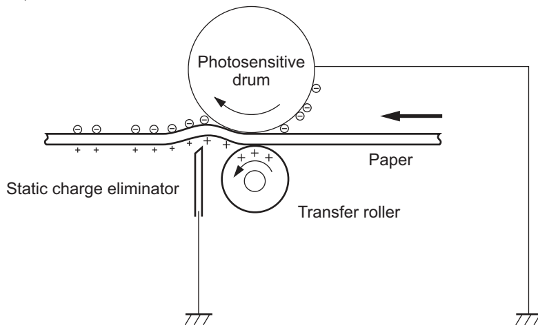
Figure 3-17 Separation
