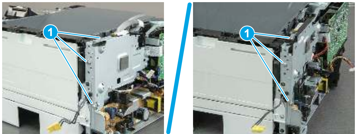
Figure 5-689 Remove three screws
