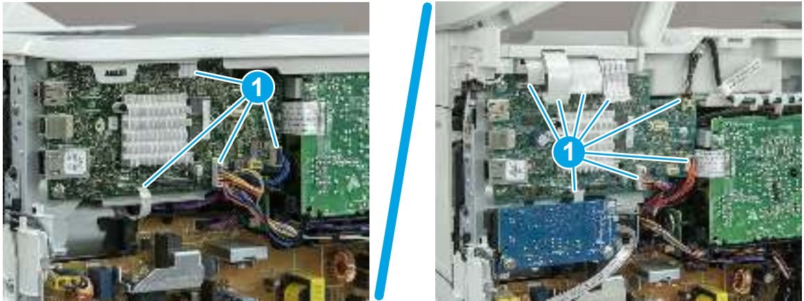
Figure 5-685 SFP/MFP: Disconnect the connectors
