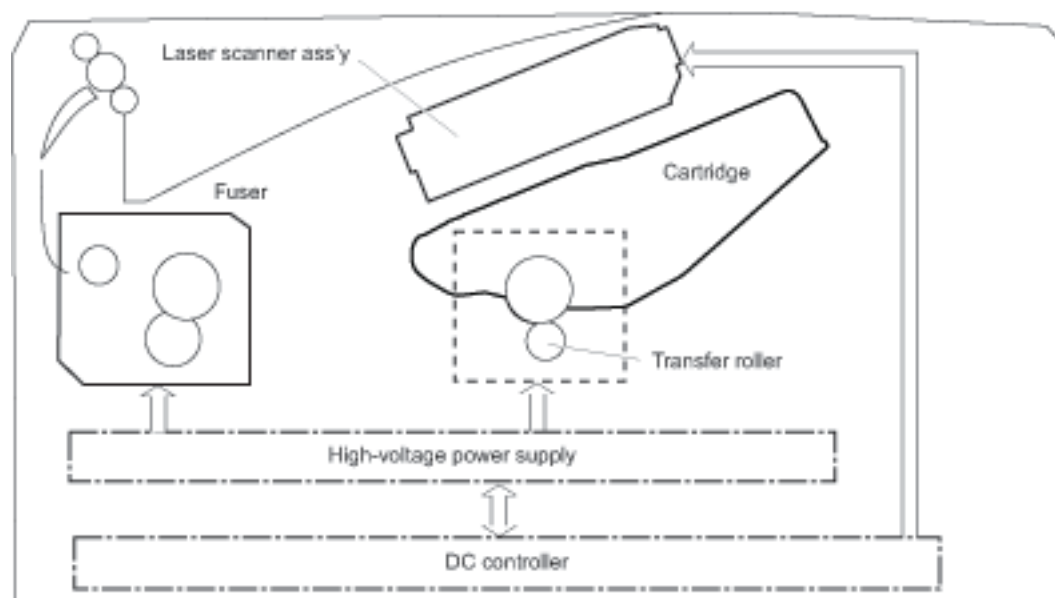
Figure 3-9 Image-formation system
