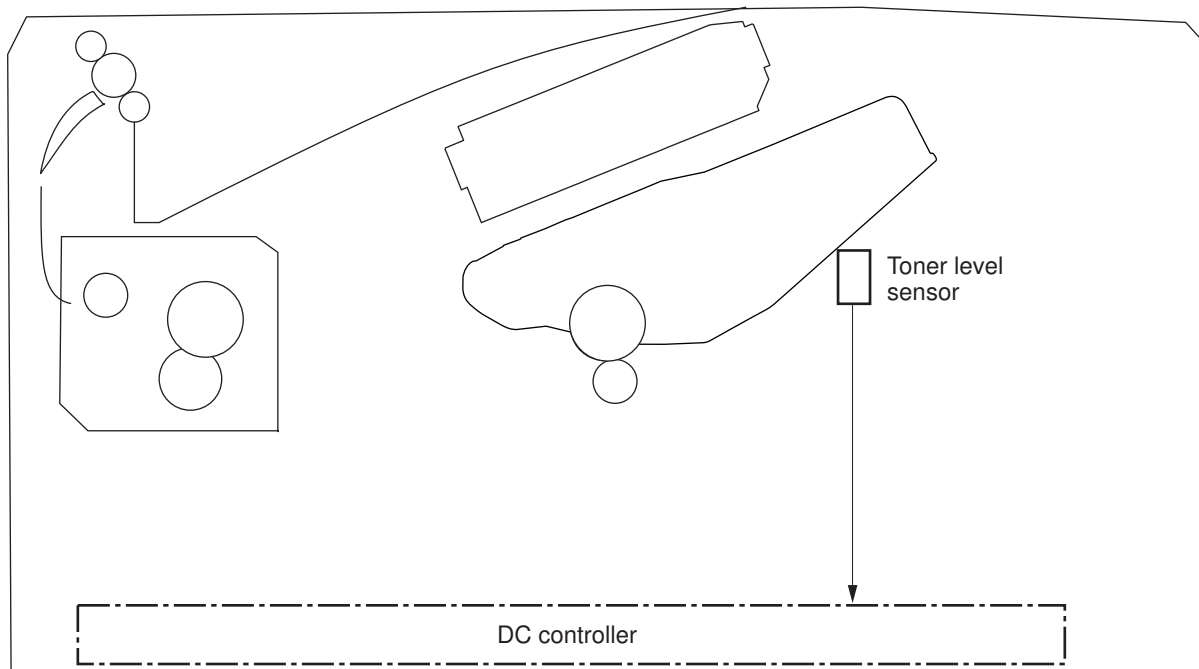
Figure 3-11 Toner-level sensor
