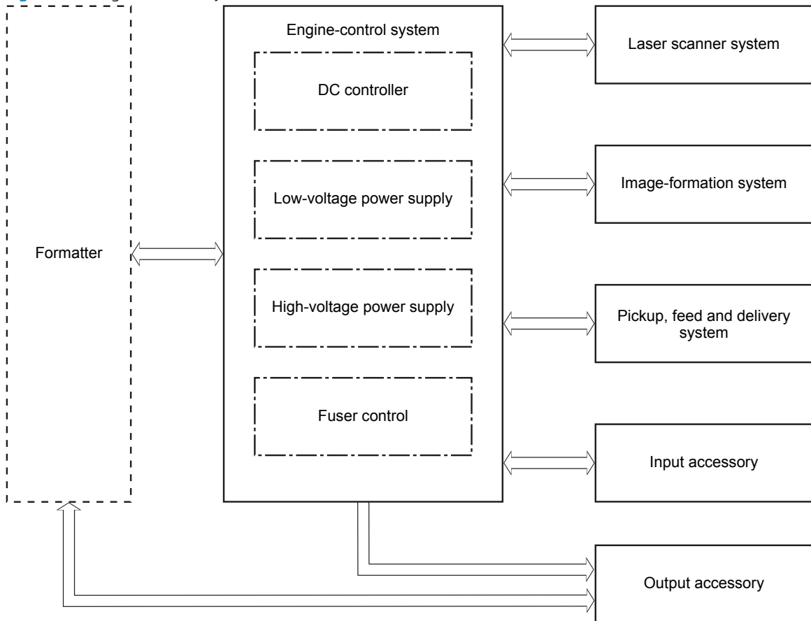
Figure 1-2 Engine-control system
