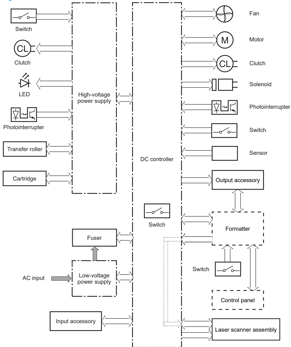
Figure 1-3 DC controller
