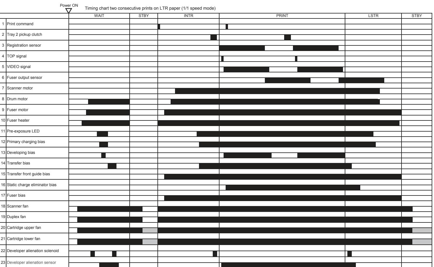
Figure 2-90 General timing chart
