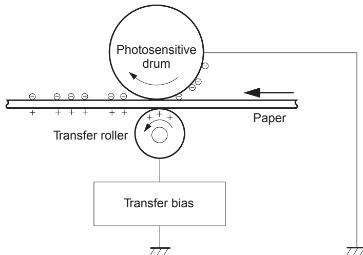
Figure 1-18 4. Transfer
