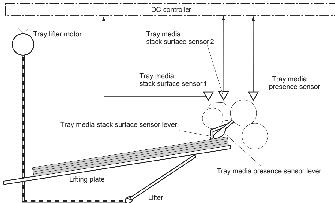
Figure 1-51 Trays 3 and 4 paper feeder lift operation
