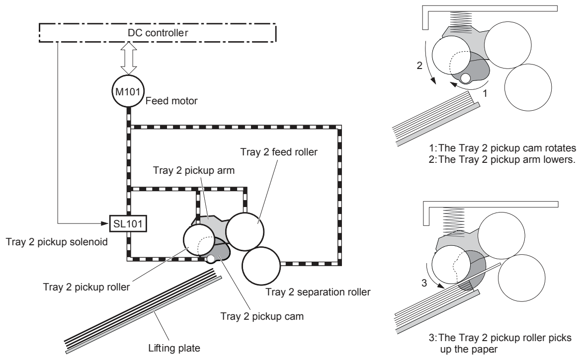
Figure 1-28 Tray 2 pickup
