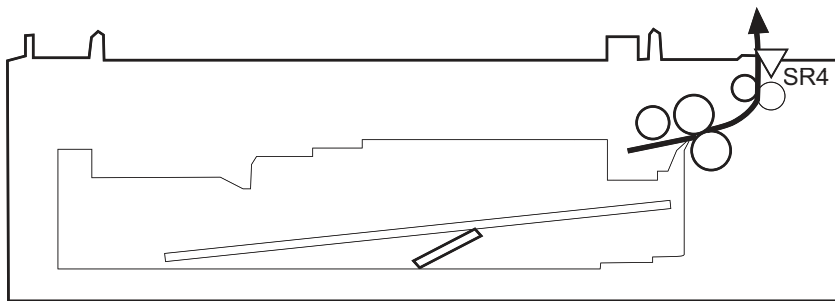
Figure 1-53 1x500-sheet paper feeder media feed sensor
