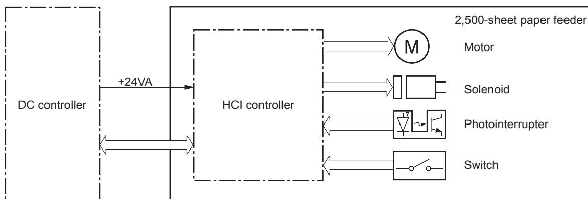
Figure 1-49 Signal flow for the 2,500-sheet high-capacity paper feeder controller
