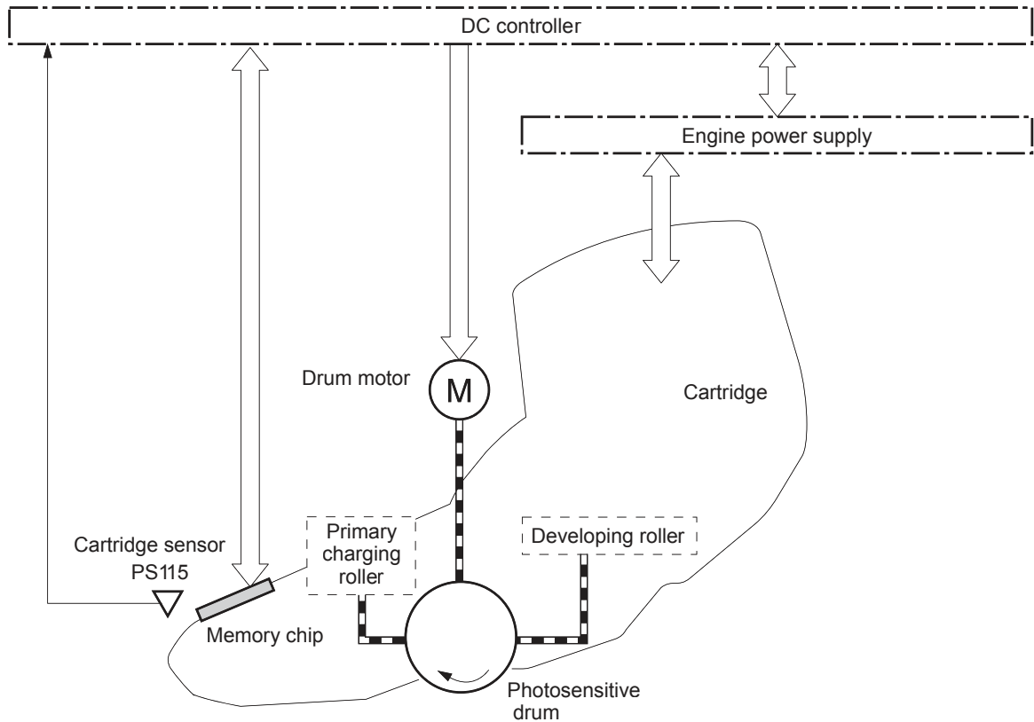
Figure 1-22 Toner Cartridge
