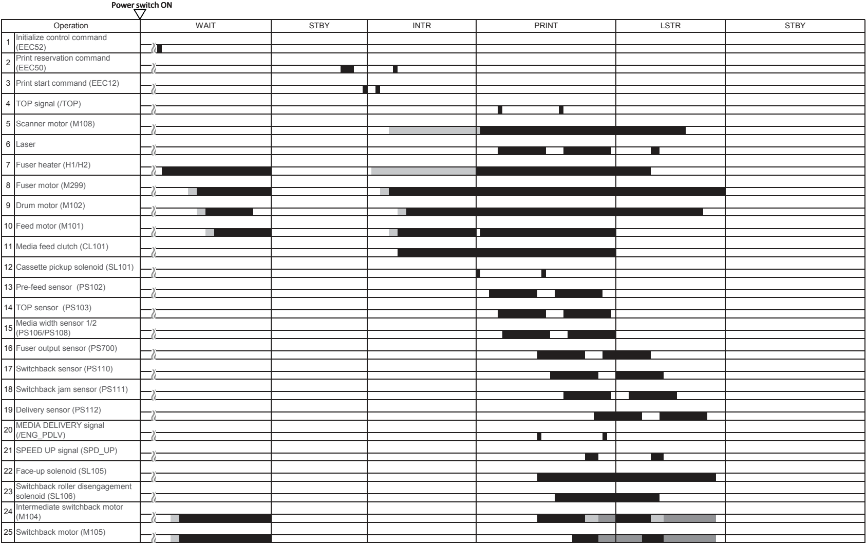
Figure 2-52 General timing chart (1 of 2)
