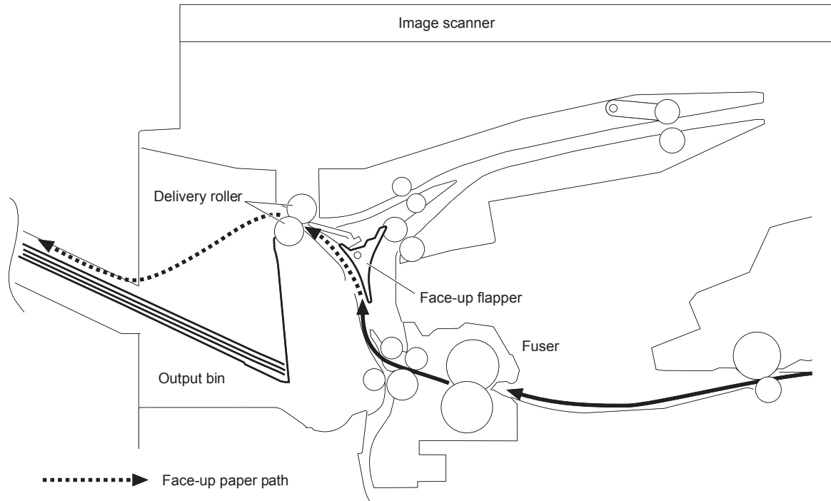
Figure 1-37 Face-up delivery
