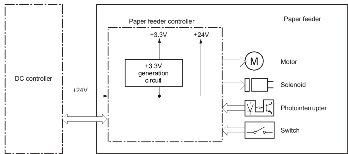
Figure 1-45 Signal flow for the 1x500-sheet paper feeder controller
