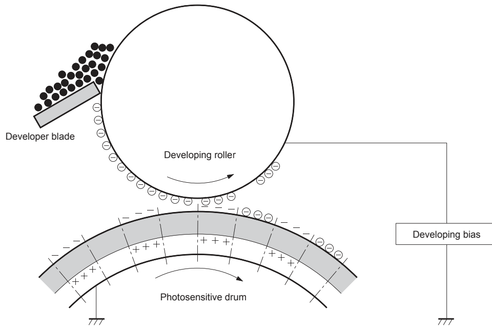
Figure 1-17 3. Developing
