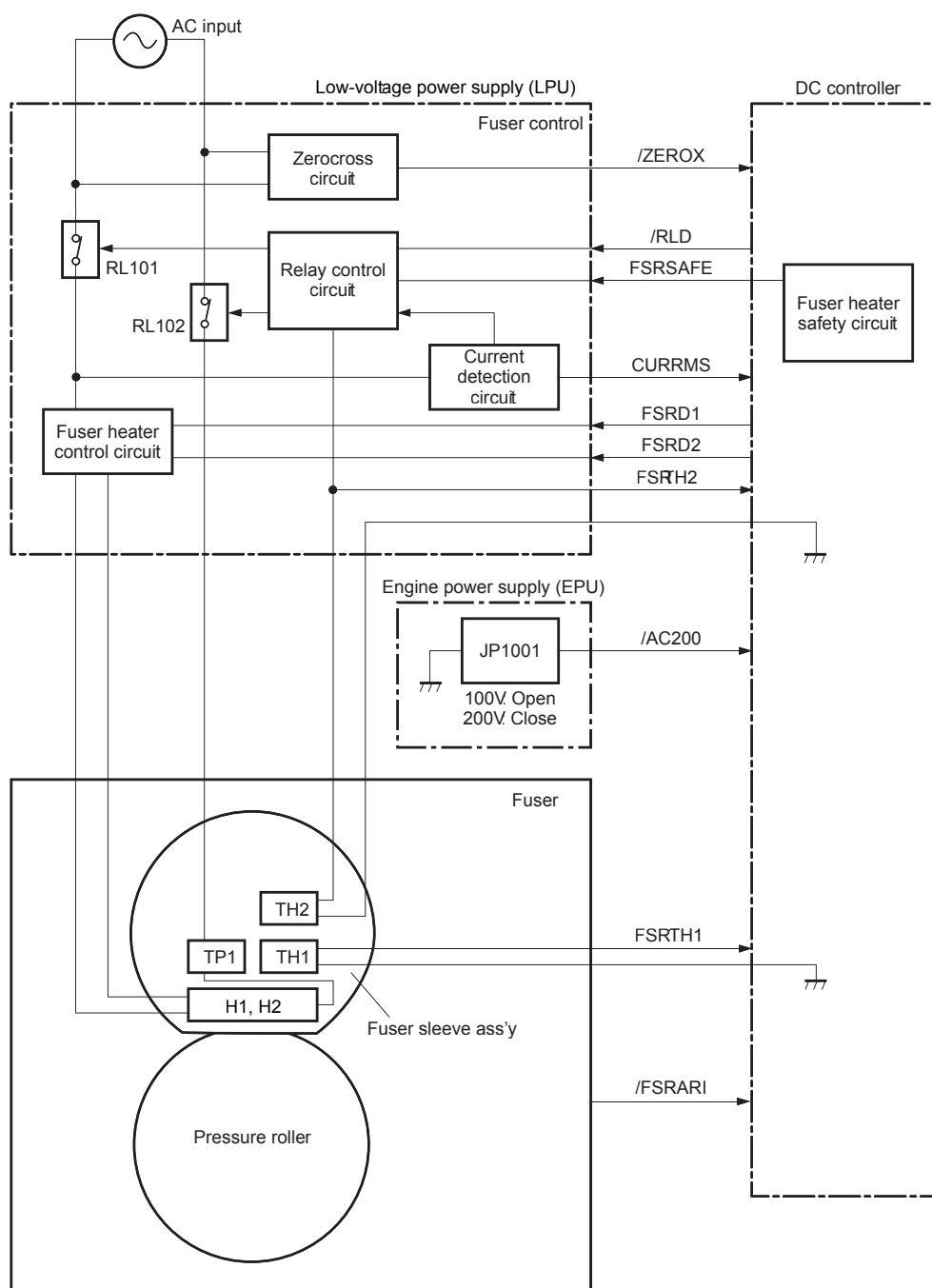
Figure 1-10 Fuser circuit
