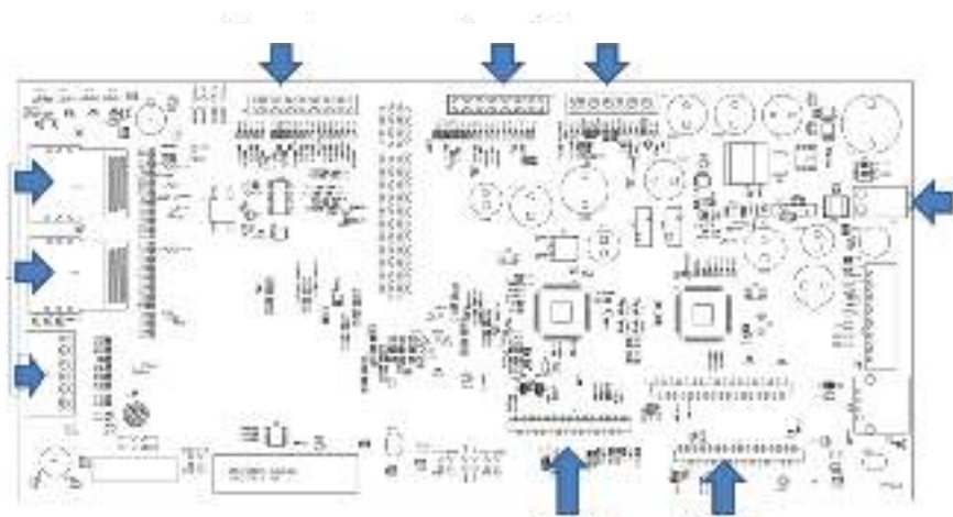
Figure 2-49 Scanner controller board (SCB) connectors
