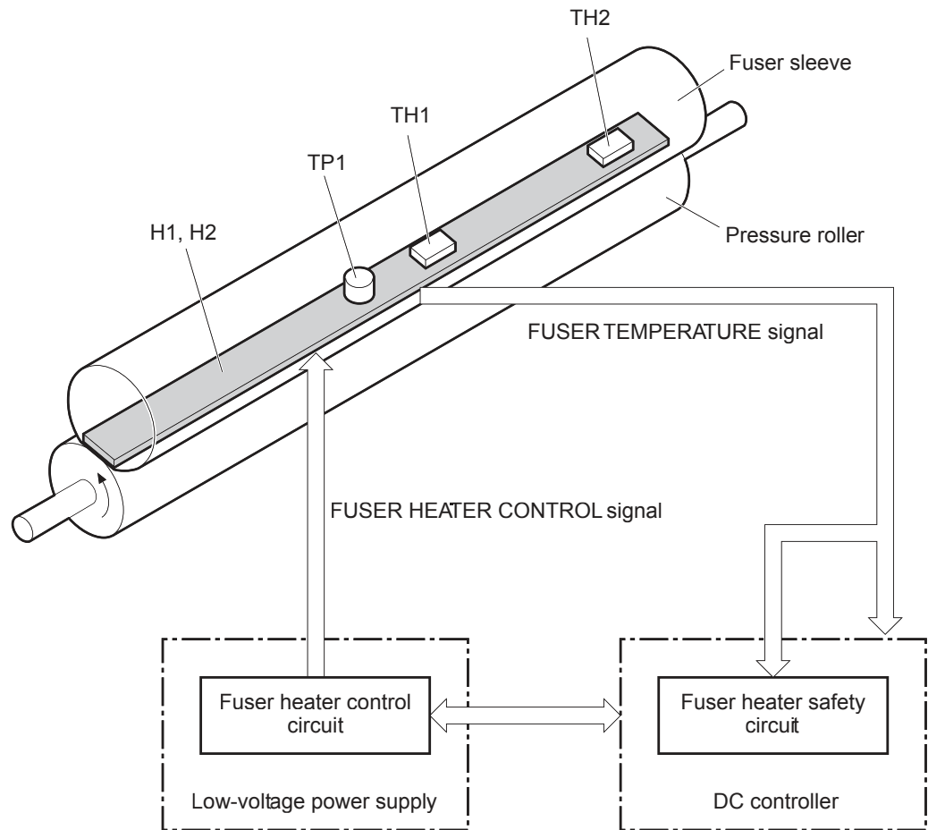
Figure 1-9 Fuser components
