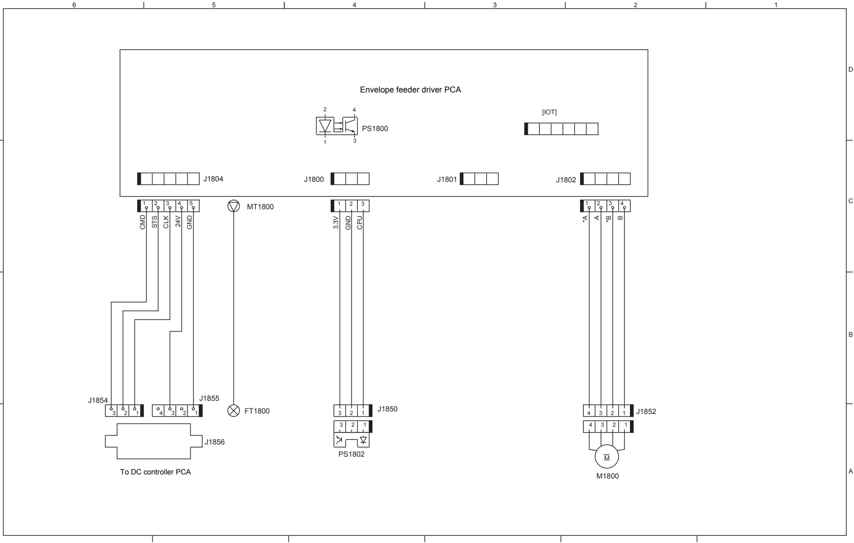
Figure 2-58 General circuit diagram for the envelope feeder
