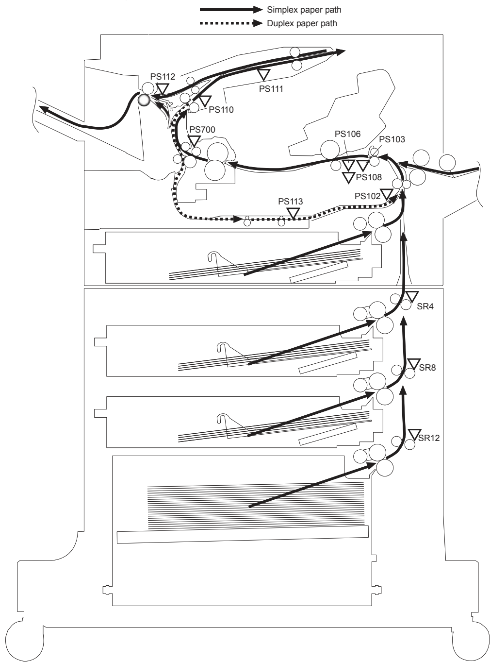
Figure 1-41 Jam detection sensors
