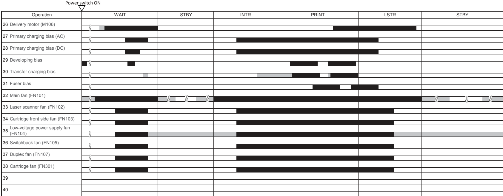
Figure 2-53 General timing chart (2 of 2)
