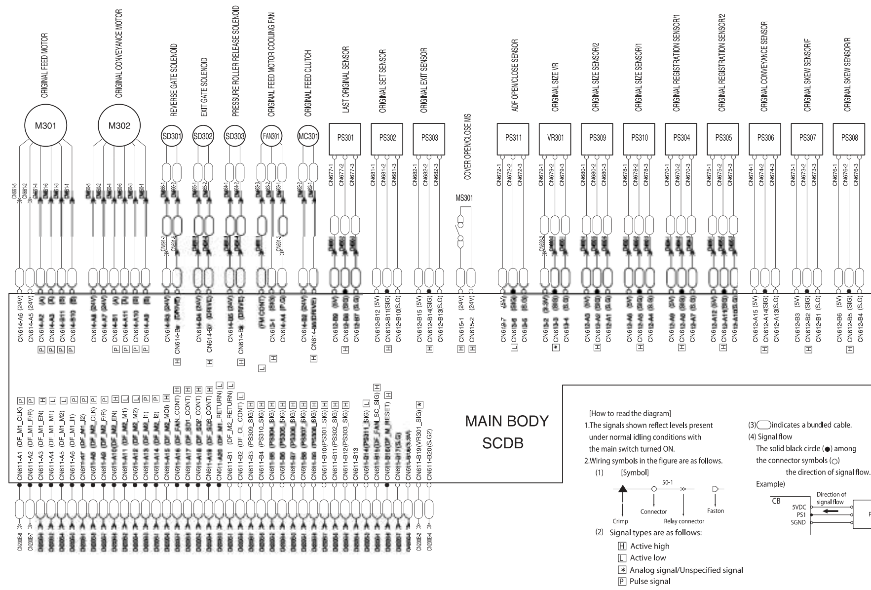
ADF Overall Wiring Diagram
