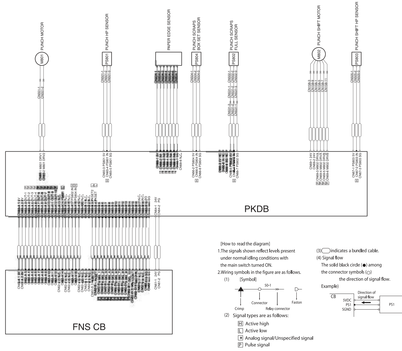
PK(Punch Kit) Overall Wiring Diagram
