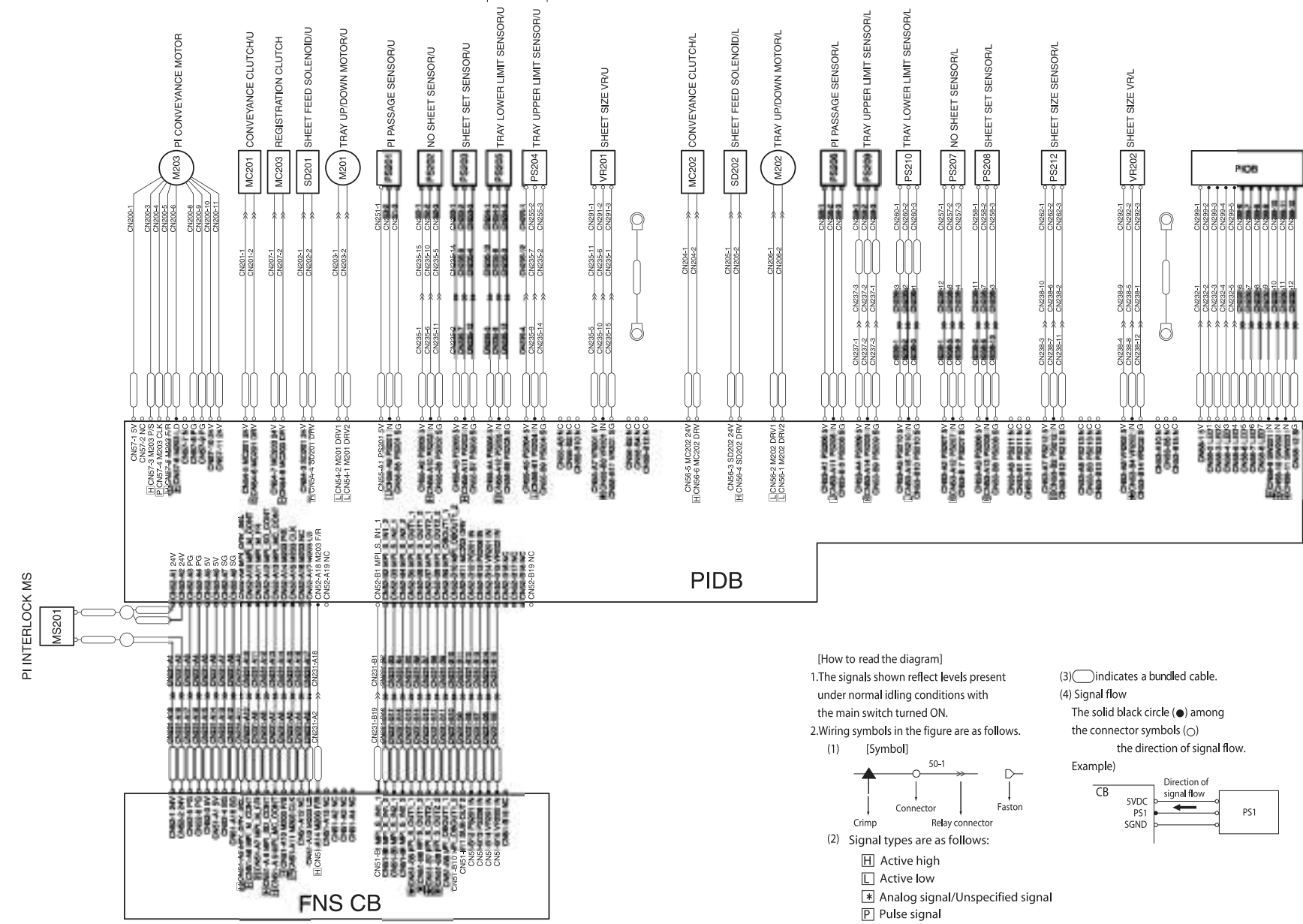
PI (Post Insertion) Overall Wiring Diagram
