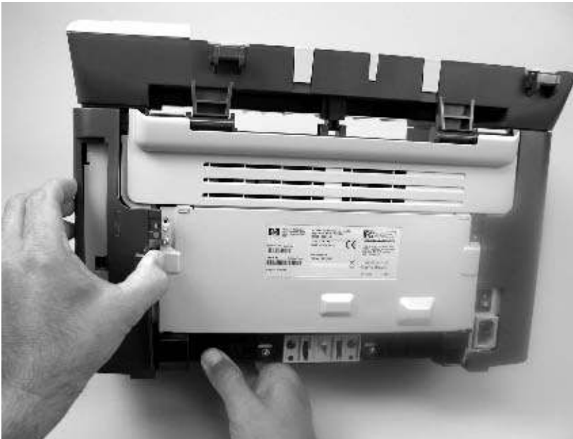
Figure 6-9 Remove the scanner assembly (2 of 11)
