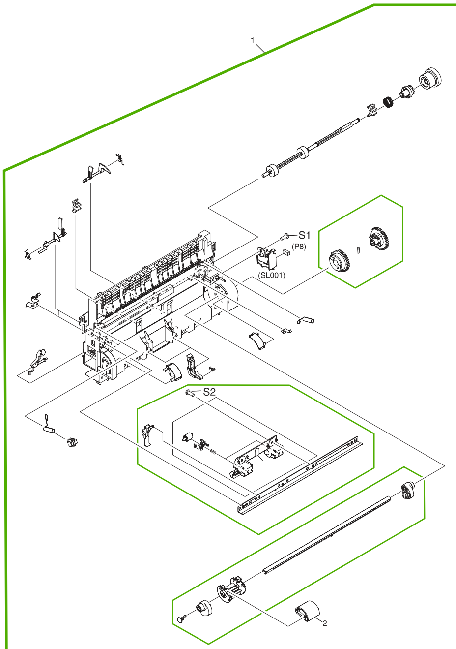
Figure 8-9 Paper-pickup assembly
