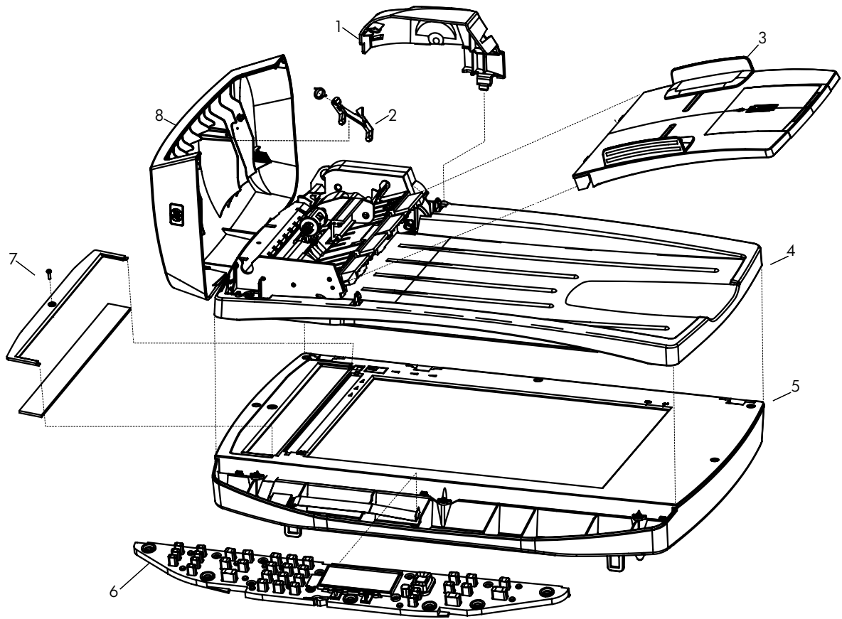
Figure 7-1 Scanner and ADF assemblies
