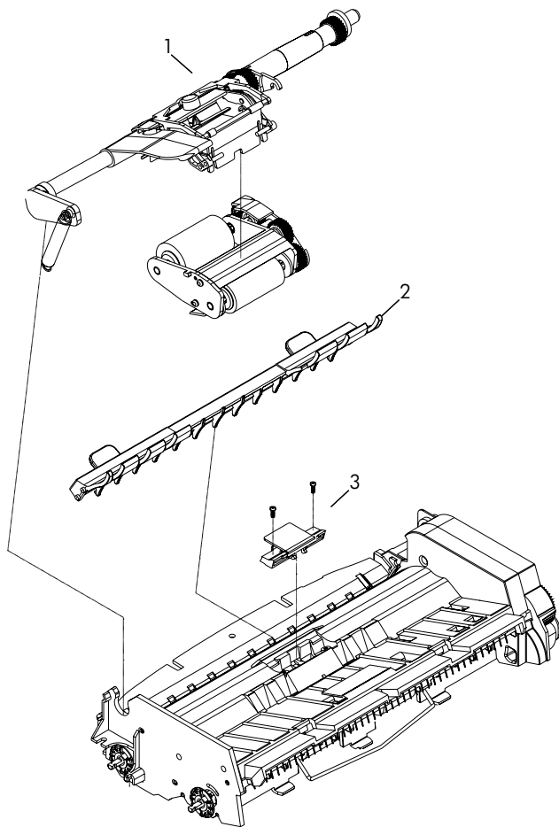
Figure 7-2 ADF internal components
