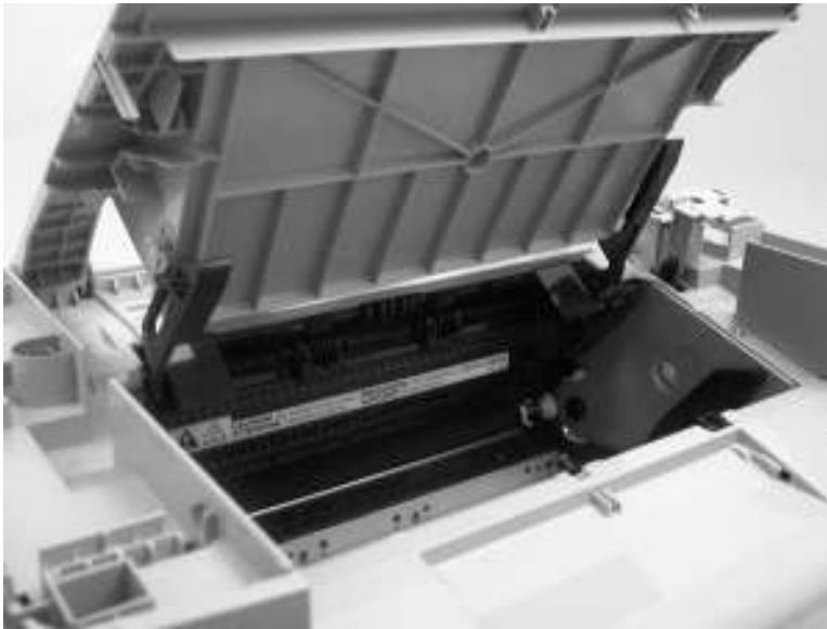
Figure 5-57 Remove the print-cartridge door (1 of 2)
