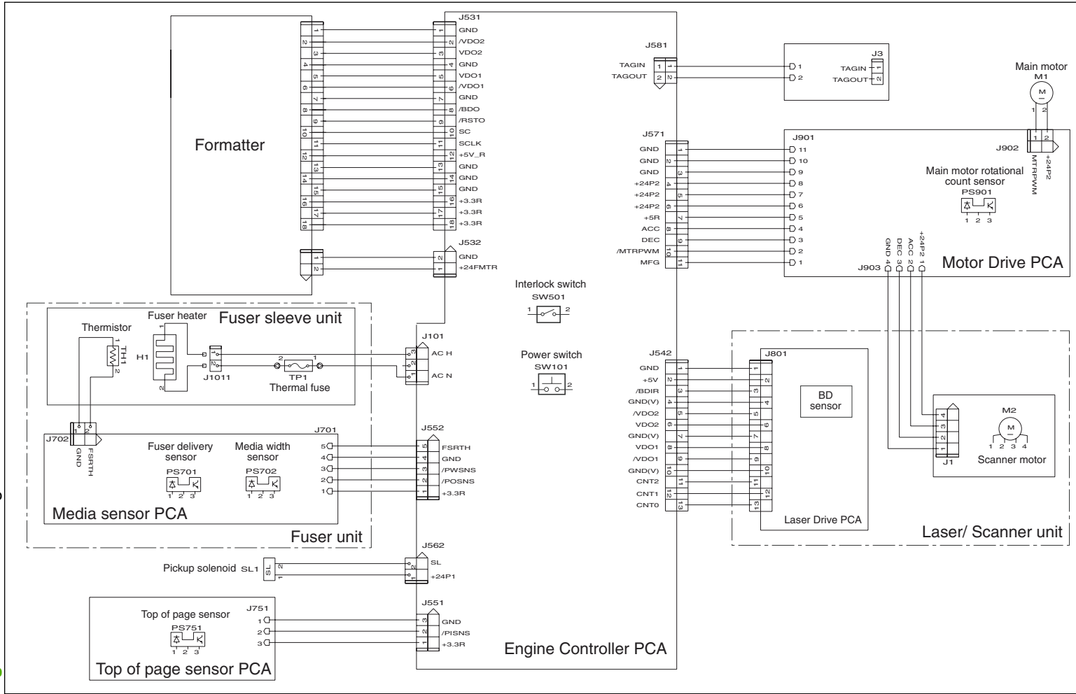
Figure 6-12 Circuit diagram
