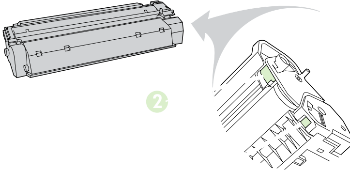
Figure 6-2 Print-cartridge high-voltage connection points (left side)
