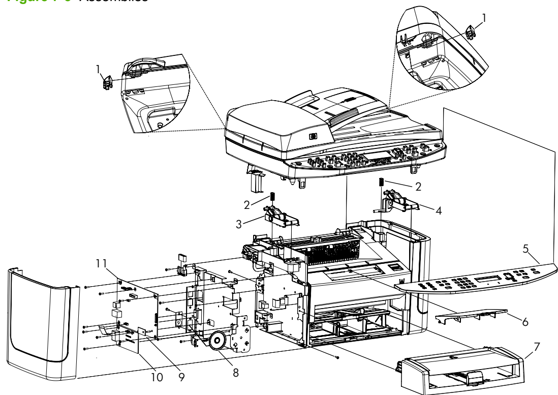
Figure 7-3 Assemblies
