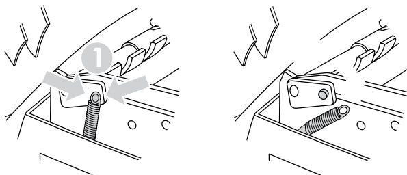
Figure 5-21 Replacing the ADF pickup roller assembly (2 of 6)
