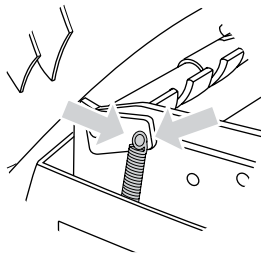
Figure 5-25 Replacing the ADF pickup roller (6 of 6)
