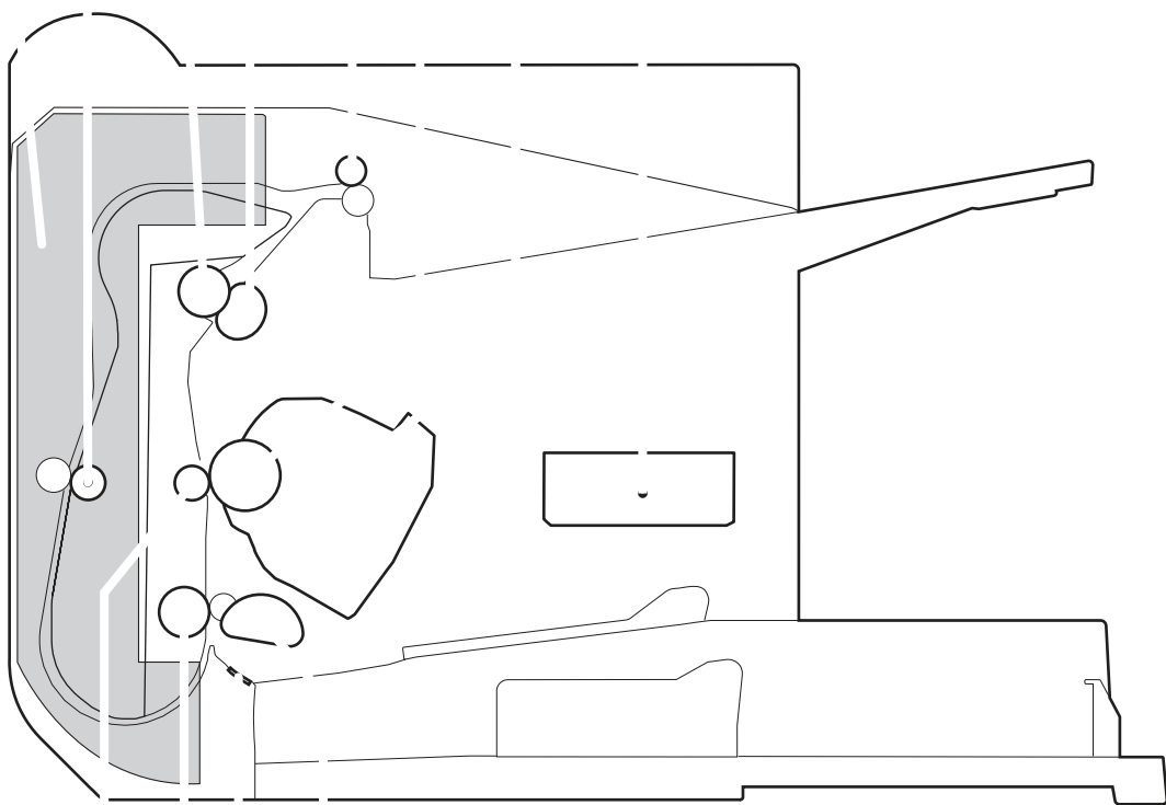
Figure 3-4 Cross-sectional view
