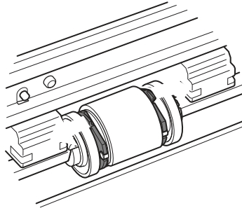
Figure 1-6 Remove the pickup roller (1 of 2)
