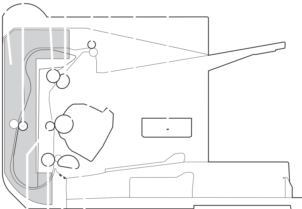
Figure 2-8 Cross-sectional view
