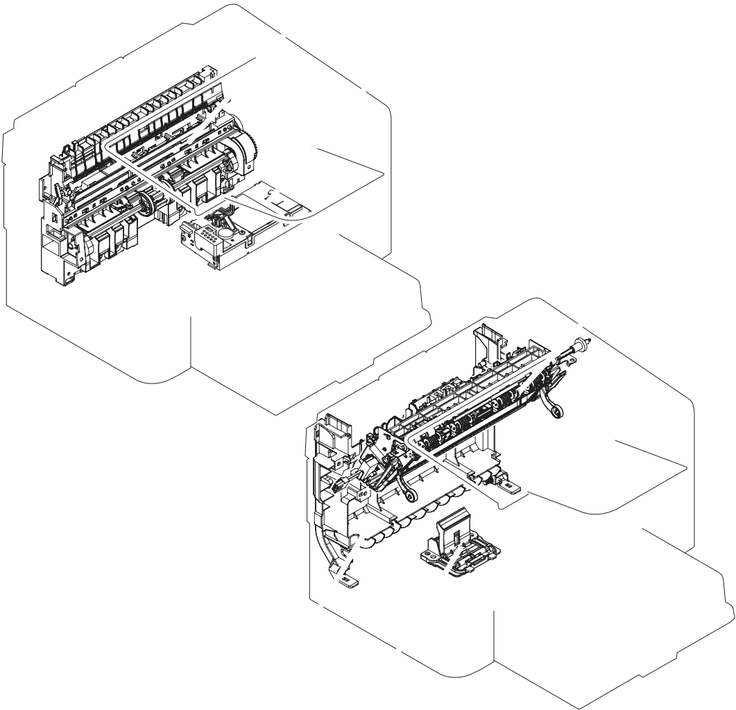
Figure 2-5 Main assemblies
