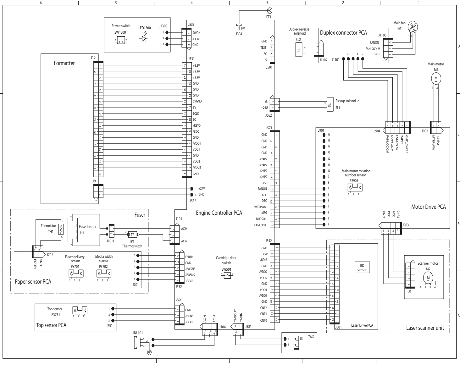
Figure 2-10 Circuit diagram
