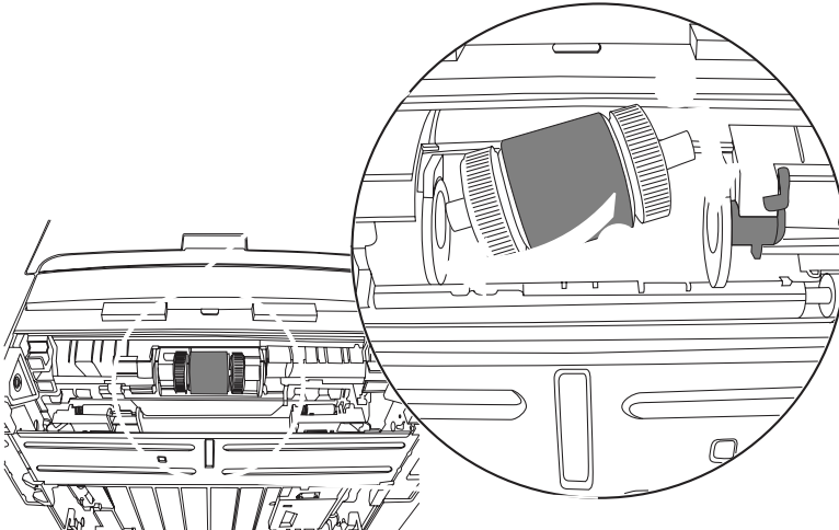
Figure 3-5 Replace the tray 2 pickup roller (5 of 7)
