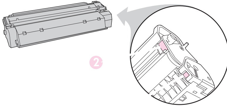
Figure 6-3 Print-cartridge high-voltage connection points (left side)
