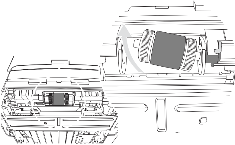
Figure 3-4 Replace the tray 2 pickup roller (4 of 7)
