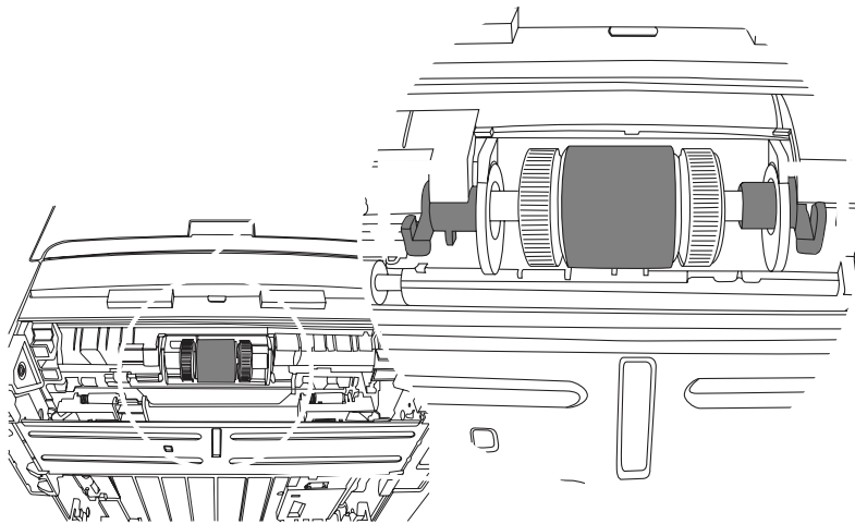
Figure 3-7 Replace the tray 2 pickup roller (7 of 7)
