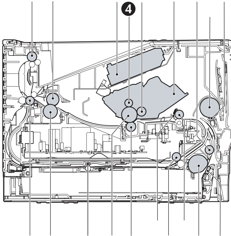
Figure 4-4 Cross-section of printer
