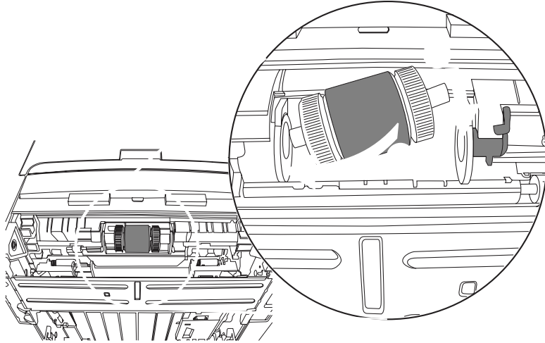
Figure 3-20 Clean the tray 2 pickup roller (4 of 6)
