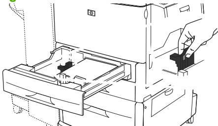
Figure 3-12 Load undetectable standard-size paper in Trays 2, 3, and 4 (3 of 6)
