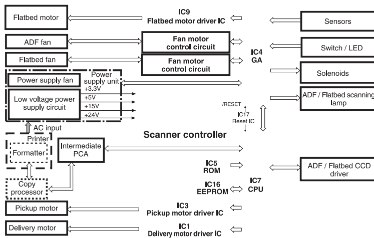
Figure 5-12 Scanner controller circuit
