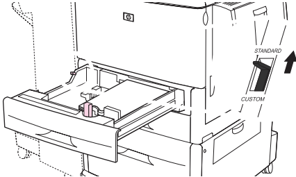
Figure 3-8 Load Trays 2, 3, and 4 (5 of 6)
