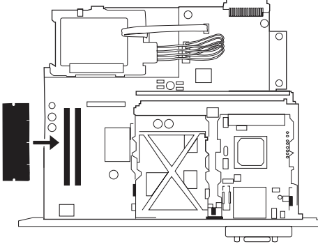
Figure 4-28 Install DDR memory DIMMs (6 of 8)
