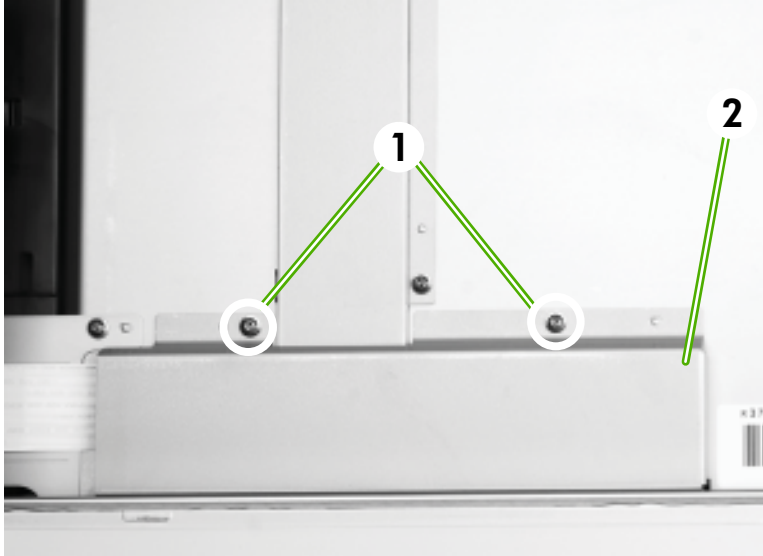
Figure 6-116 Remove the flatbed intermediate PCA (1 of 2)
