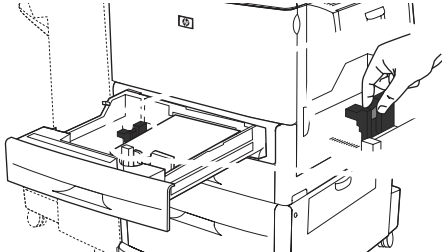
Figure 3-19 Load custom media in Trays 2, 3, and 4 (4 of 6)
