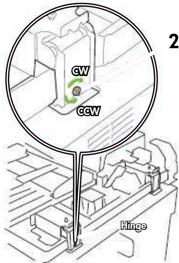
Figure 7-14 The ADF skew adjustment screw
