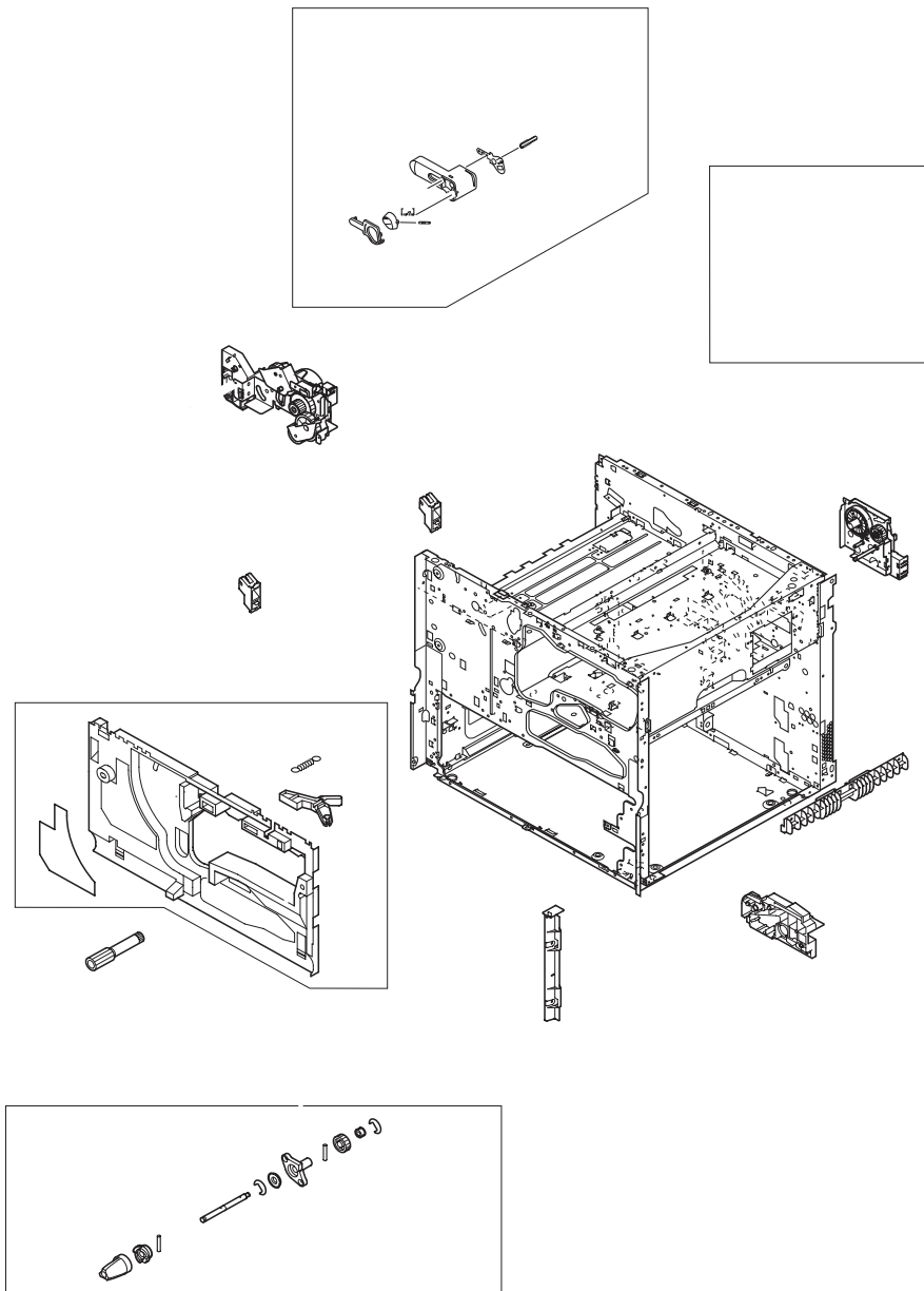
Figure 8-18 Print engine internal components (1 of 4)
