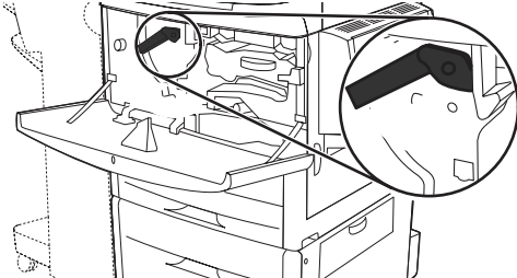
Figure 4-6 Clean the paper path (5 of 6)
