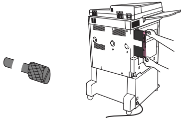
Figure 4-29 Install DDR memory DIMMs (7 of 8)
