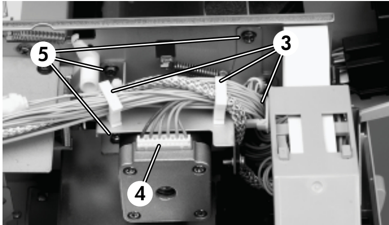
Figure 6-76 Remove the delivery motor (2 of 2)
