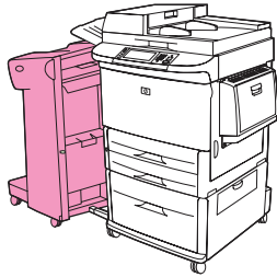
Figure 7-68 Clear a staple jam from the stapler/stacker (1 of 9)
