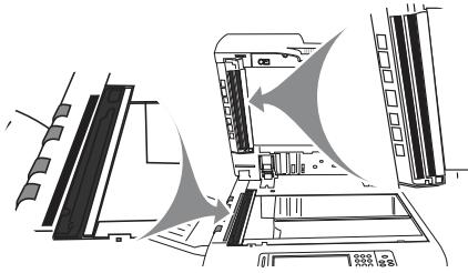
Figure 4-9 Clean the ADF delivery system (2 of 5)
