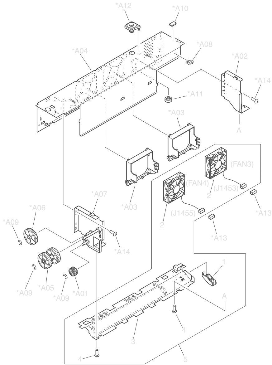
Figure 8-29 Delivery assembly
