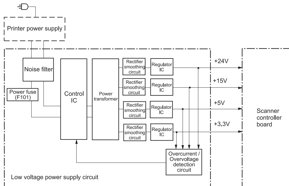
Figure 5-11 Power supply
