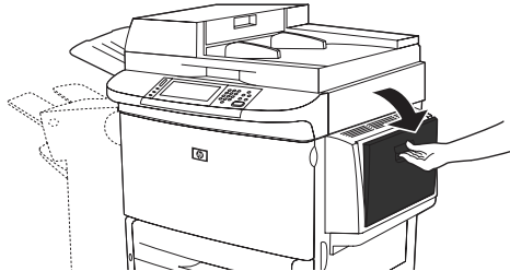
Figure 7-23 Clear jams in Tray 1 (1 of 2)
