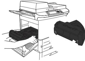
Figure 7-19 Clear jams in the duplex printing accessory (3 of 6)
