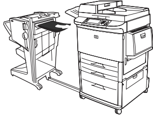
Figure 7-50 Clear booklet jams in the multifunction finisher (2 of 7)
