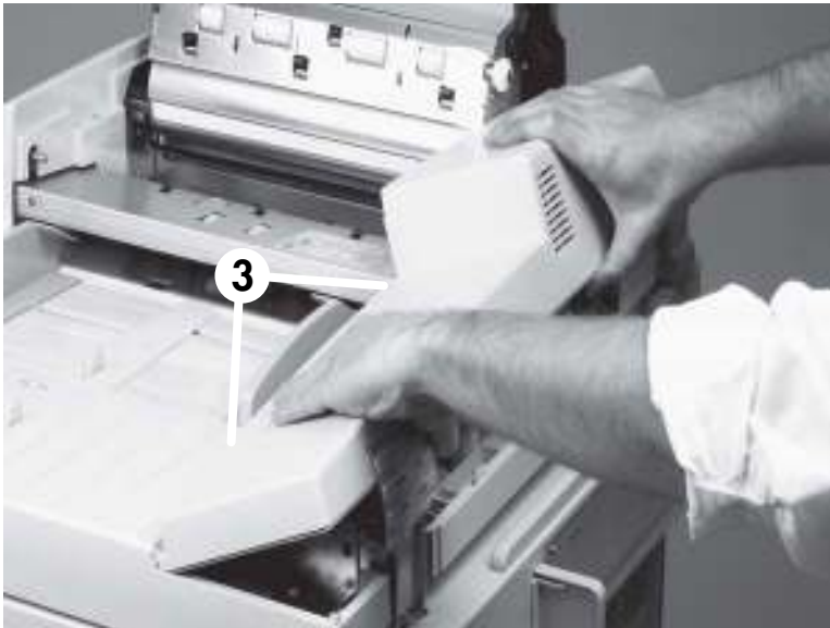
Figure 6-12 Remove the ADF back cover (2 of 2)
