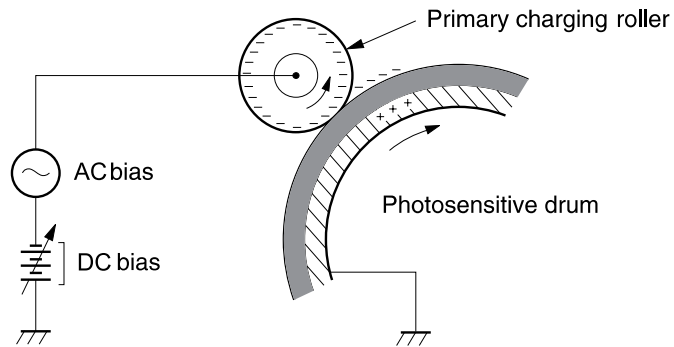
Figure 4-9 Primary charging
