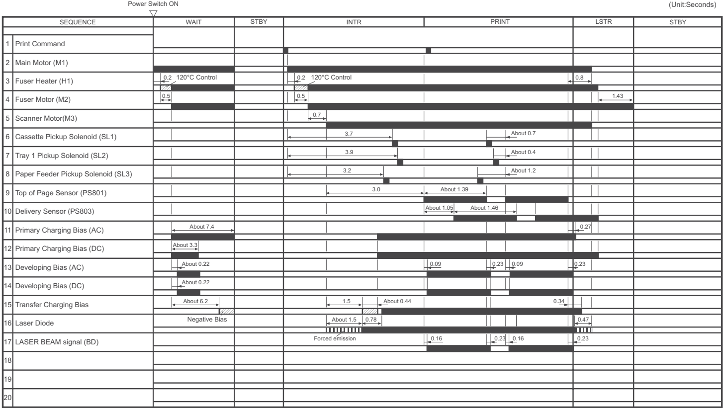
Figure 4-17 Timing diagram
