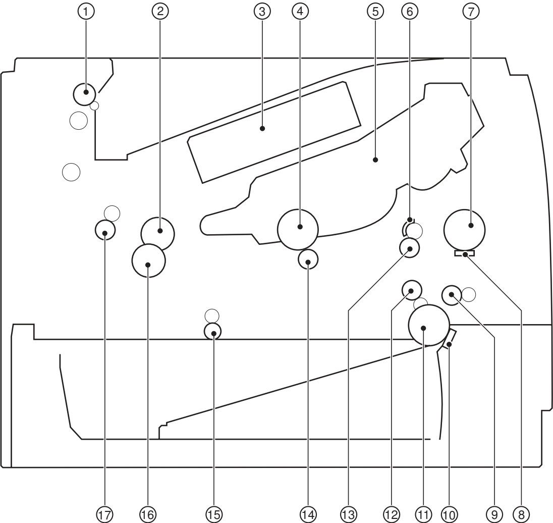
Figure 3-21 Product cross section
