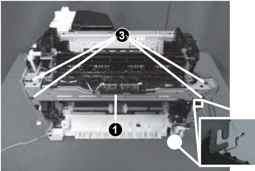
Figure 1-1802 Install the fuser
