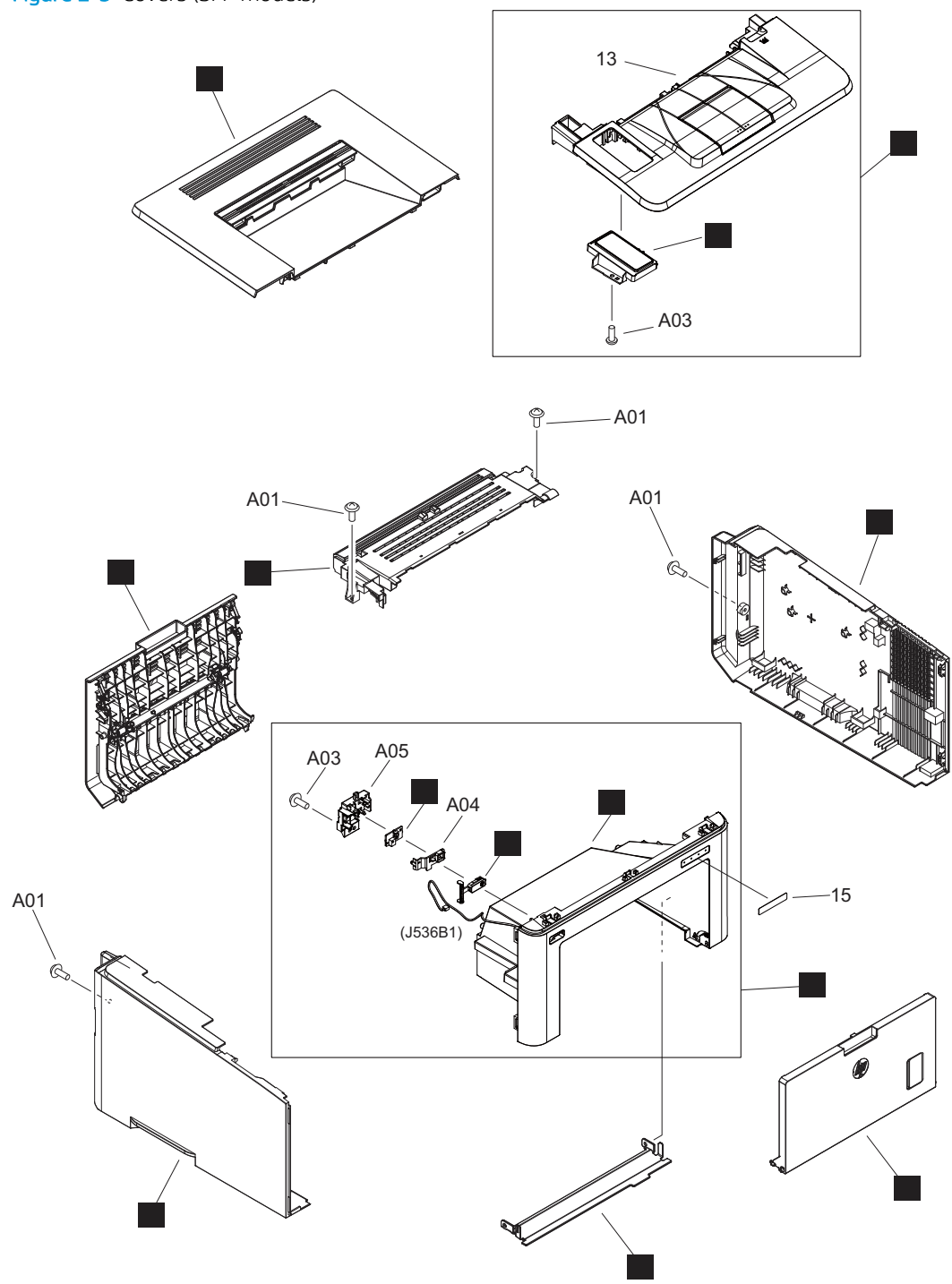
Figure 2-3 Covers (SFP models)
