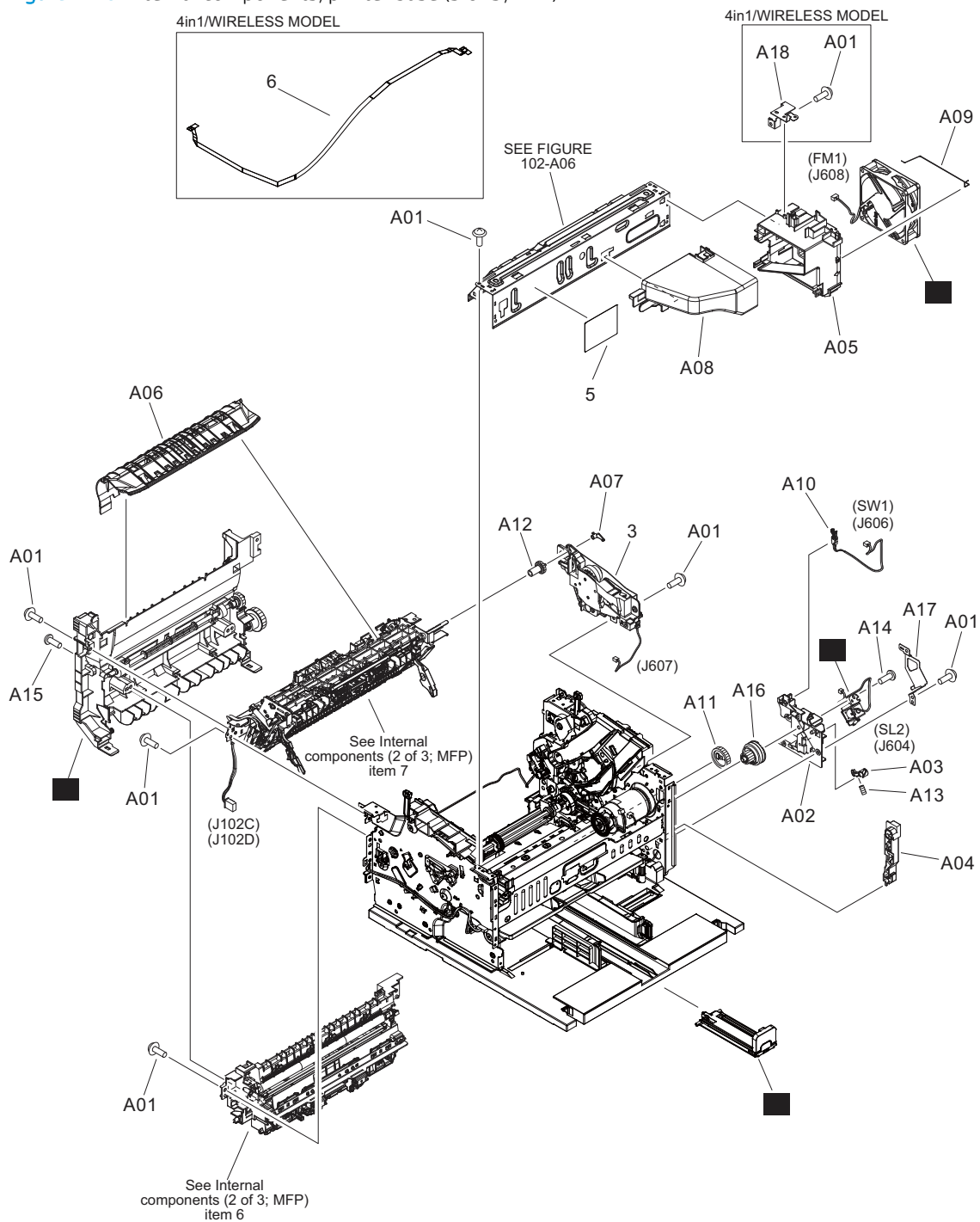
Figure 2-10 Internal components, printer base (3 of 3; MFP)
