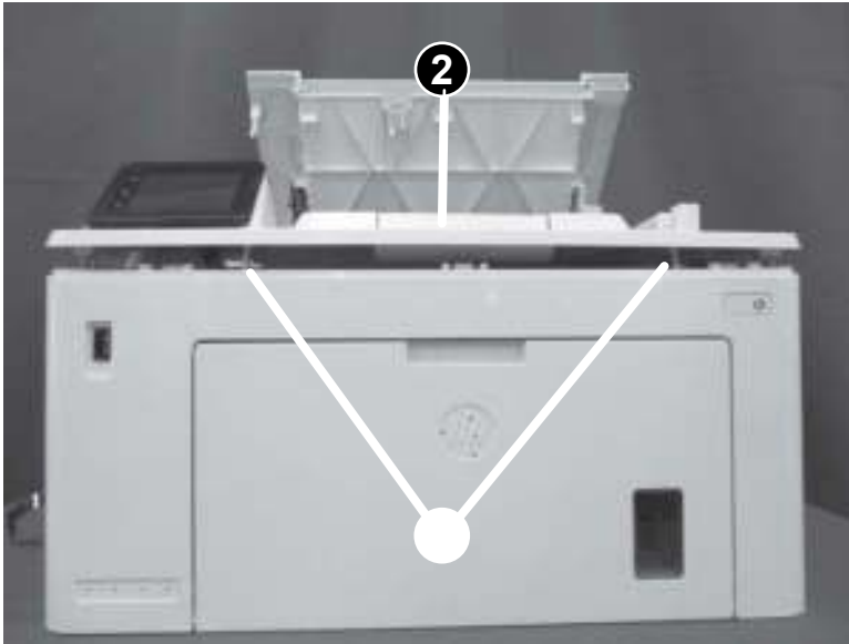
Figure 1-371 Release two tabs and remove the cover (MFP)
