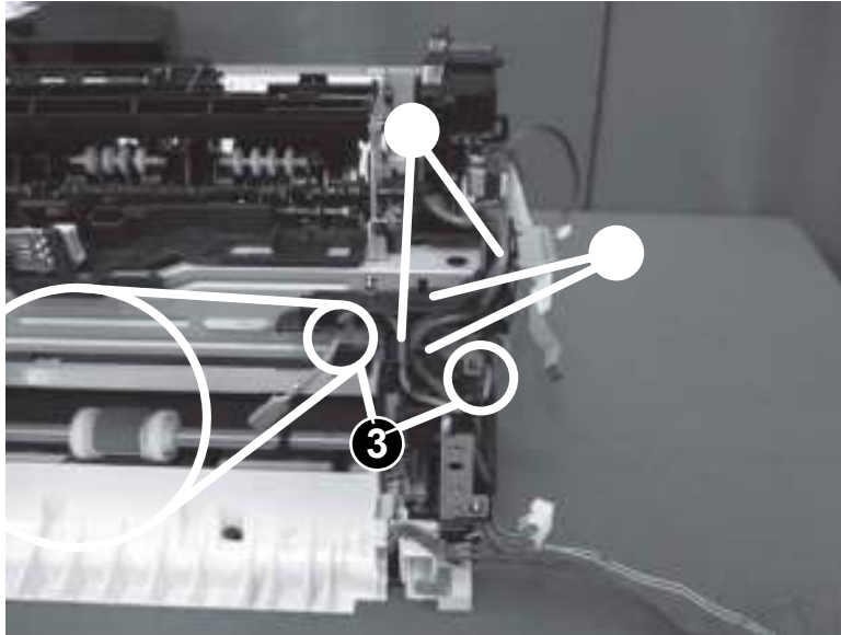
Figure 1-1805 Install the cables
