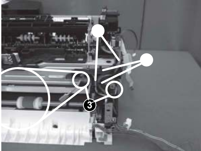
Figure 1-1791 Release the cables
