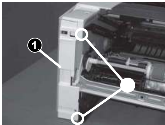
Figure 1-2107 Install the cover
