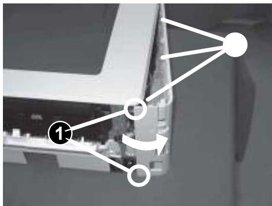
Figure 1-1551 Release two bosses and three tabs
