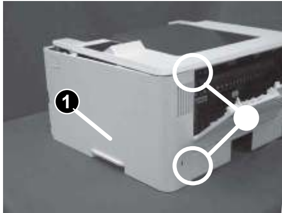
Figure 1-1433 Install the cover
