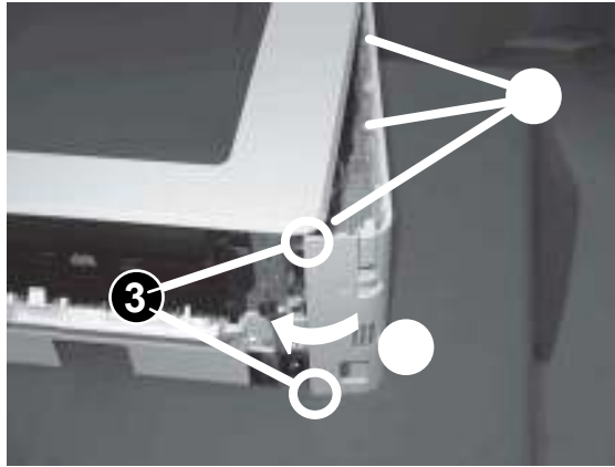
Figure 1-2148 Engage three tabs and two bosses
