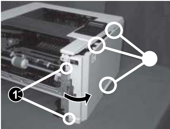
Figure 1-185 Release two bosses and three tabs
