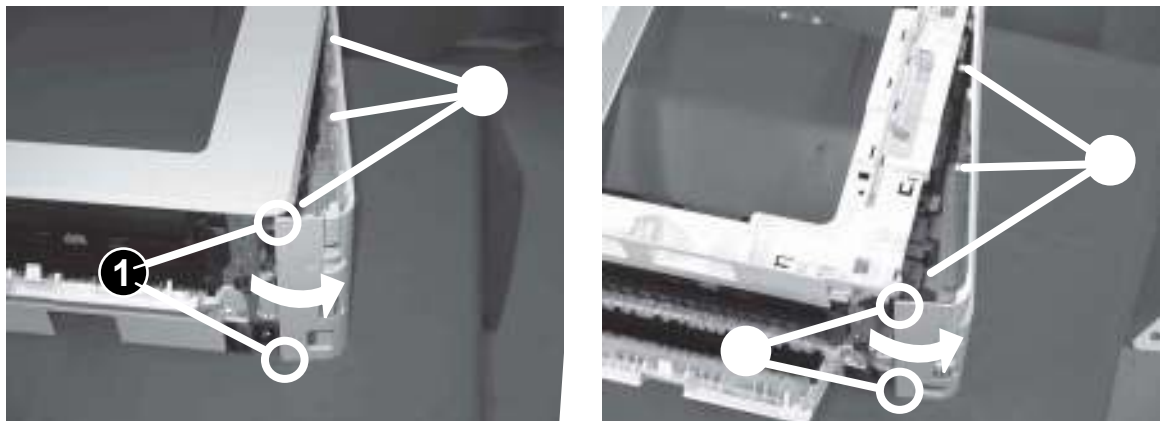
Figure 1-861 Release two bosses and three tabs
