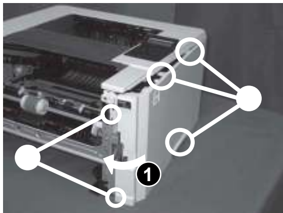
Figure 1-1434 Engage two bosses and one tab
