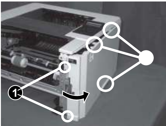
Figure 1-1354 Release two bosses and three tabs
