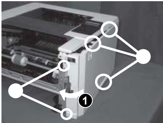
Figure 1-1238 Engage two bosses and one tab
