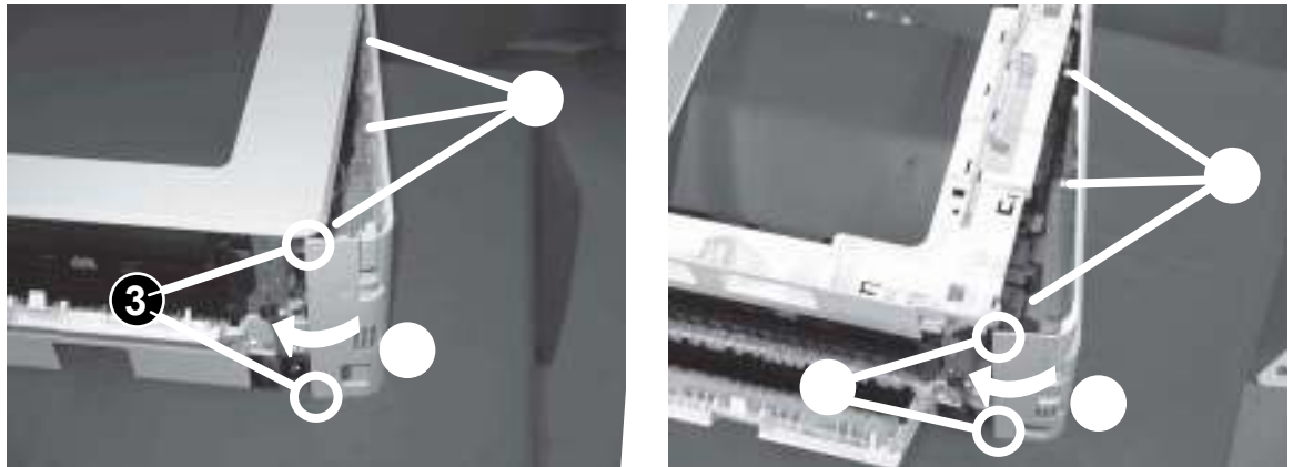
Figure 1-845 Engage three tabs and two bosses
