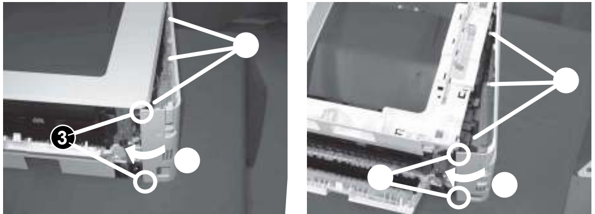
Figure 1-111 Engage three tabs and two bosses
