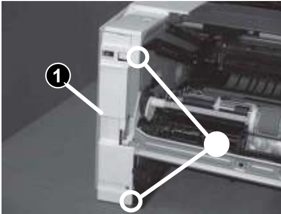
Figure 1-936 Install the cover
