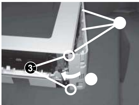
Figure 1-166 Engage three tabs and two bosses
