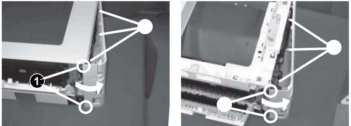
Figure 1-1216 Release two bosses and three tabs
