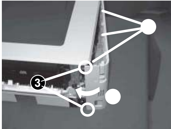
Figure 1-2191 Engage three tabs and two bosses
