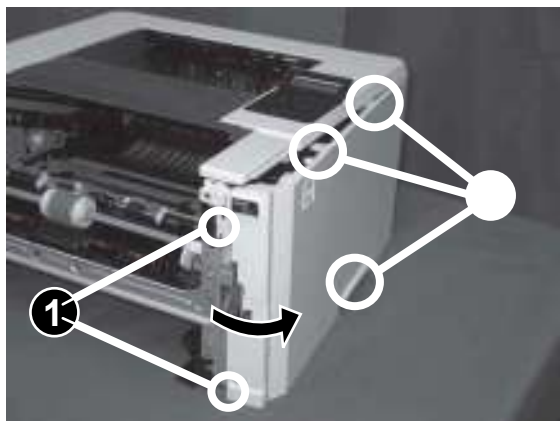
Figure 1-1651 Release two bosses and three tabs
