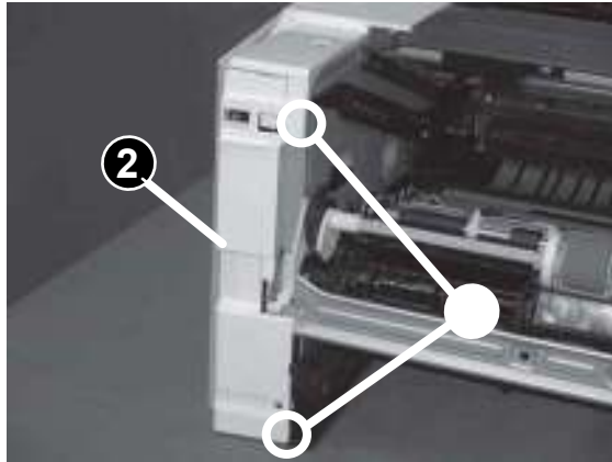
Figure 1-1125 Remove the cover
