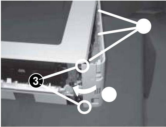
Figure 1-791 Engage three tabs and two bosses
