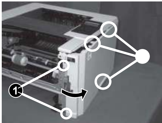
Figure 1-1127 Release two bosses and three tabs
