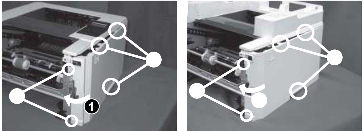
Figure 1-1016 Engage two bosses and one tab
