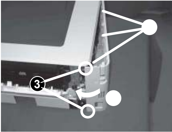
Figure 1-434 Engage three tabs and two bosses
