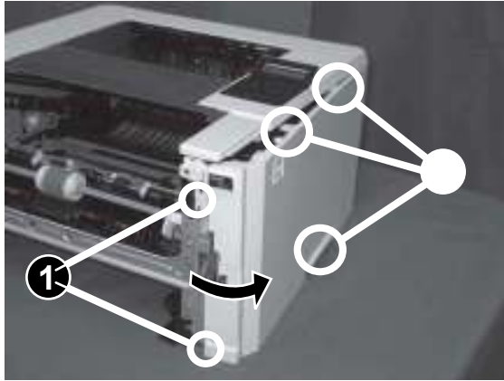
Figure 1-956 Release two bosses and three tabs
