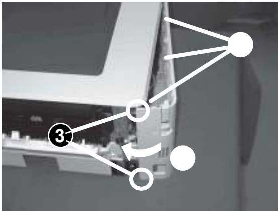
Figure 1-937 Engage three tabs and two bosses
