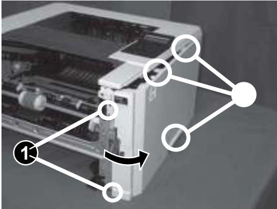
Figure 1-1261 Release two bosses and three tabs
