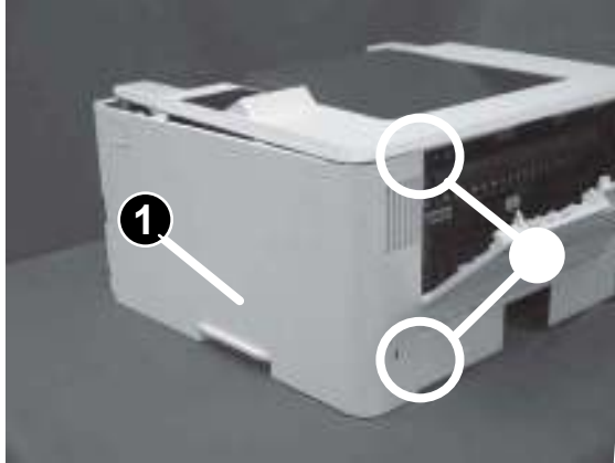
Figure 1-1237 Install the cover
