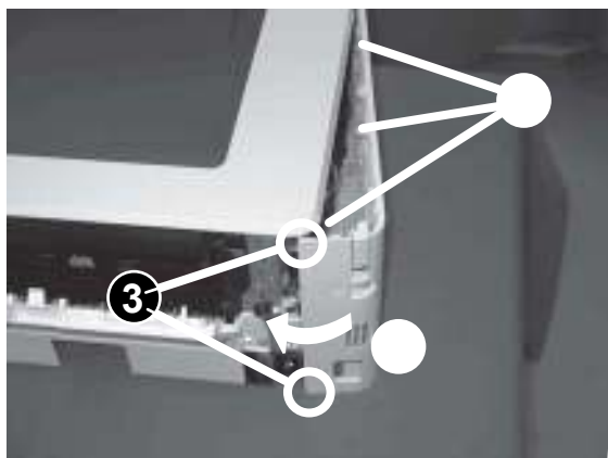
Figure 1-1200 Engage three tabs and two bosses
