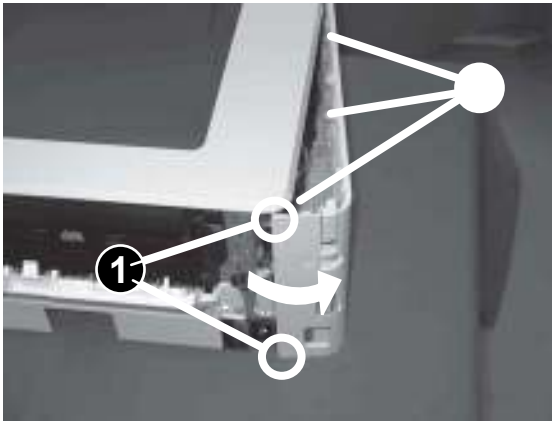
Figure 1-2178 Release two bosses and three tabs
