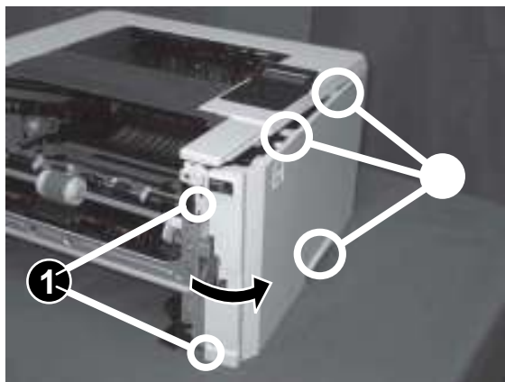
Figure 1-1859 Release two bosses and three tabs
