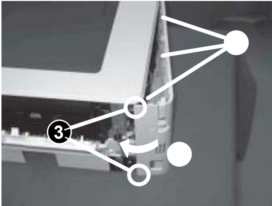
Figure 1-202 Engage three tabs and two bosses
