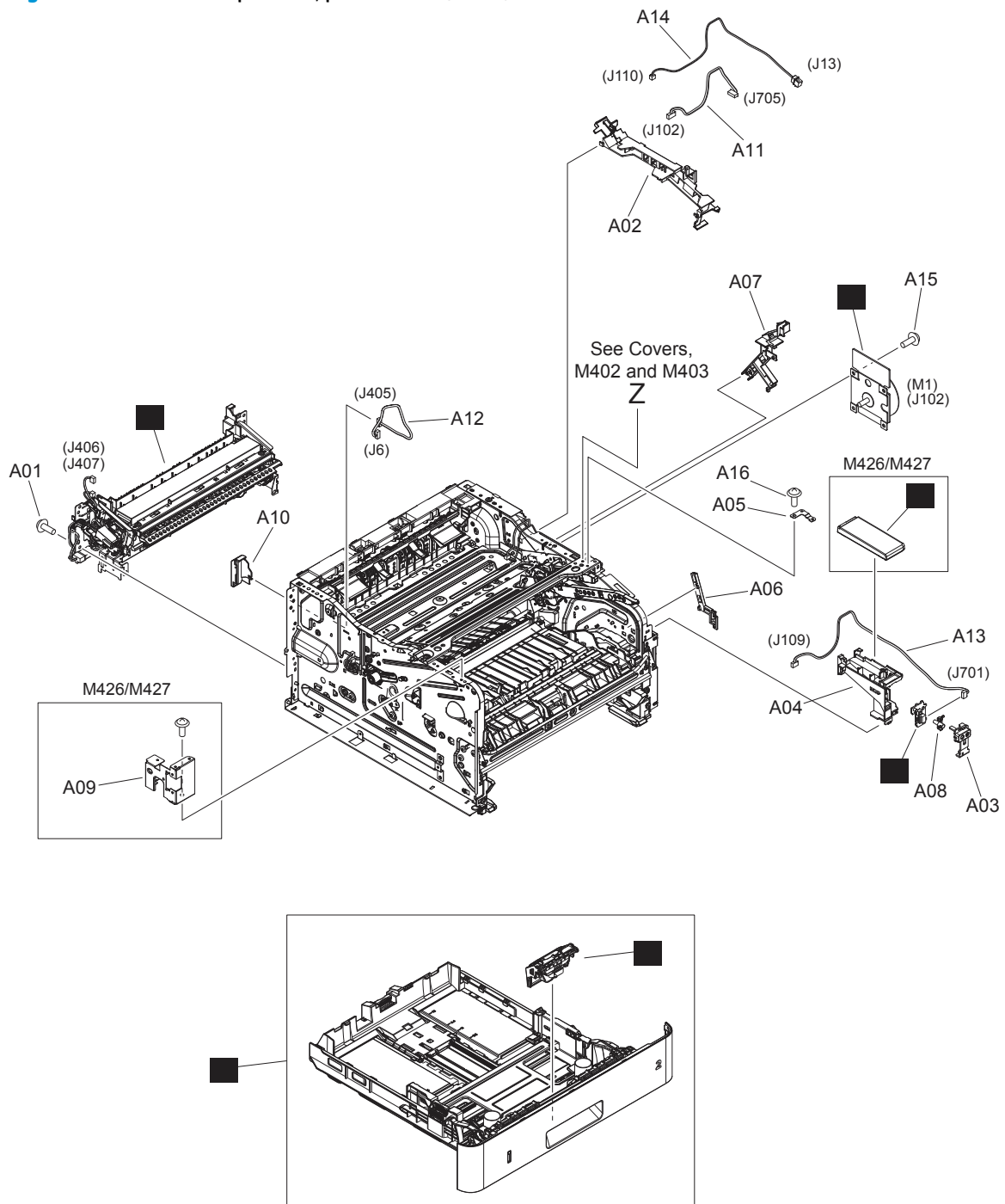
Figure 2-5 Internal components, printer base (2 of 3)
