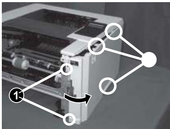
Figure 1-130 Release two bosses and three tabs
