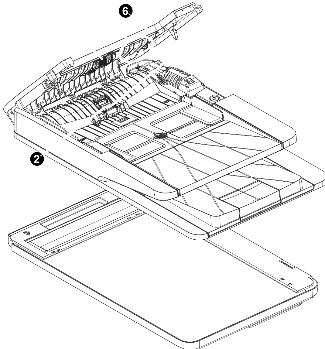
Figure 2-1 Main assemblies (document feeder and image scanner)
