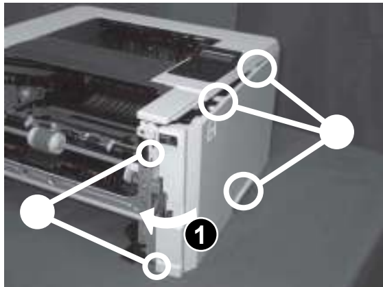
Figure 1-712 Engage two bosses and one tab
