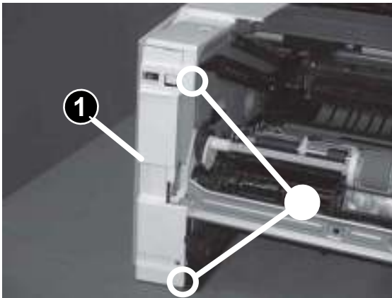
Figure 1-820 Install the cover
