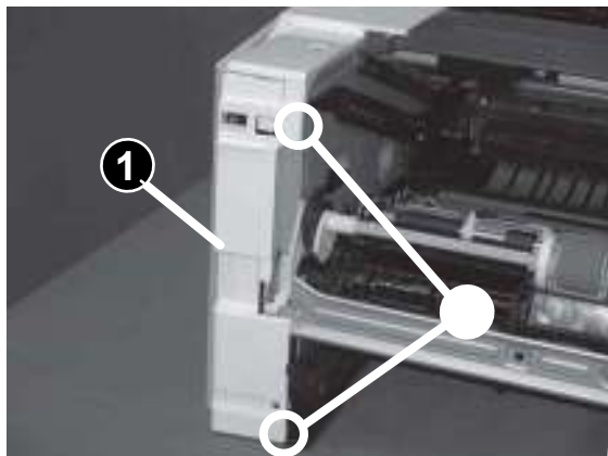
Figure 1-1334 Install the cover
