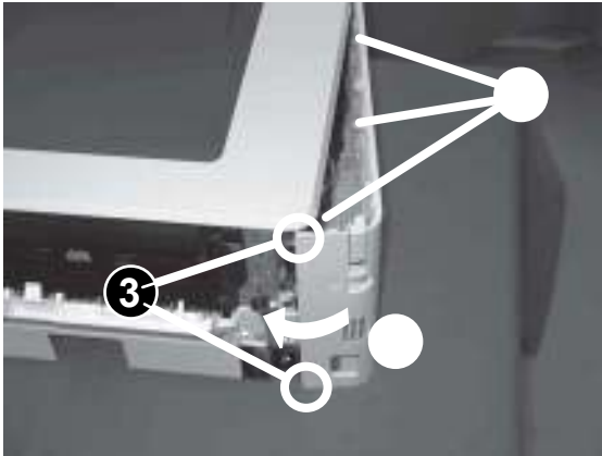
Figure 1-354 Engage three tabs and two bosses
