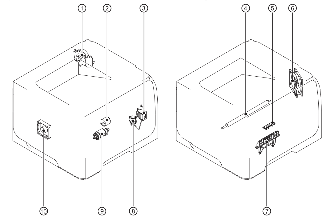
Figure 2-8 Motors, fans, solenoids, and rollers assembly locations
