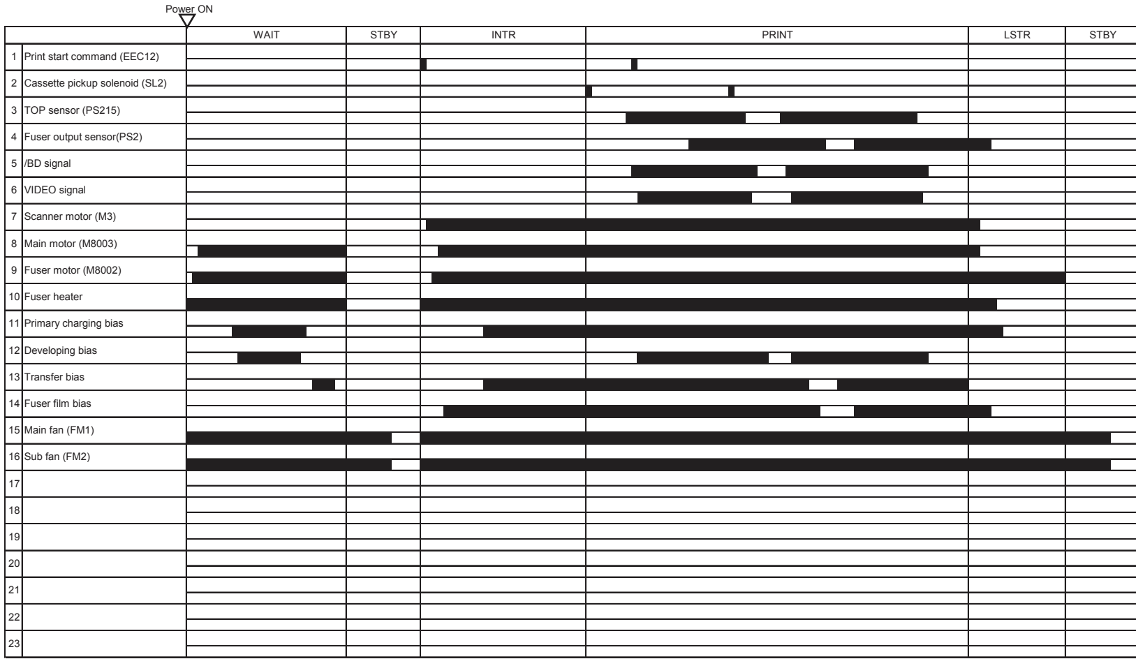
Figure 2-11 General timing chart
